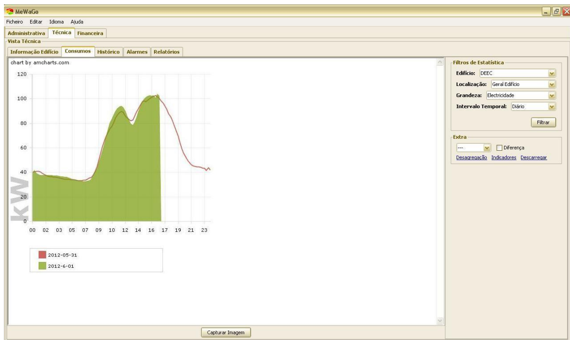
Figura 12 – MeWaGo Desktop
