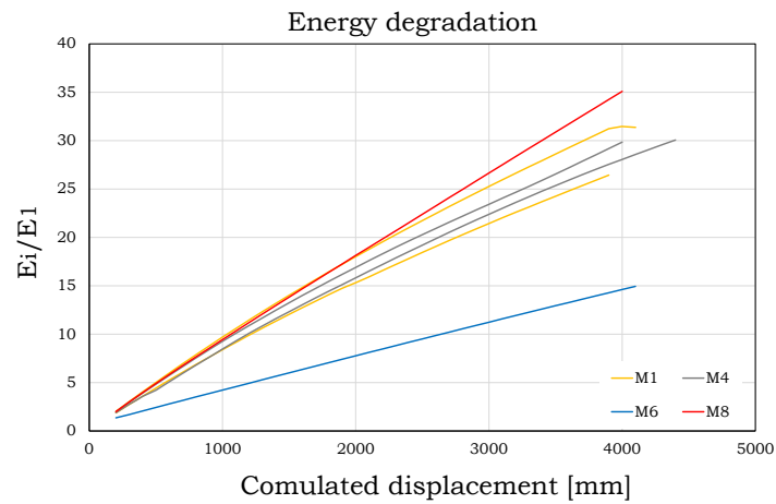
Fig. 2.24 – Energy degradation
