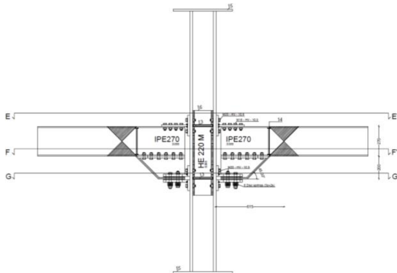
Fig. 4.9 – Internal joint configuration (HE220M / IPE270 - Horizontal pads)
