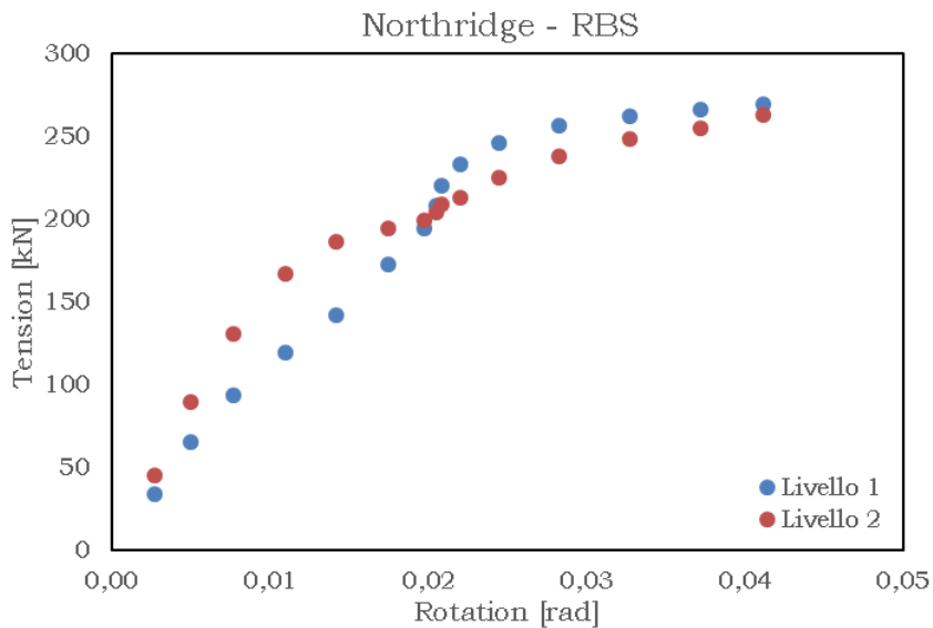
Fig. 5.135 – Tension vs rotation – NORTHTRIDGE RBS
