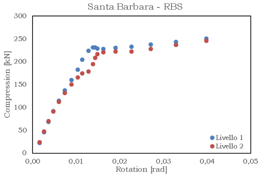
Fig. 5.146 – Compression vs rotation – SANTA BARBARA RBS
