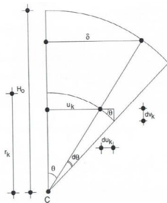
Fig. 5.8 – Rigid movement of structural elements
