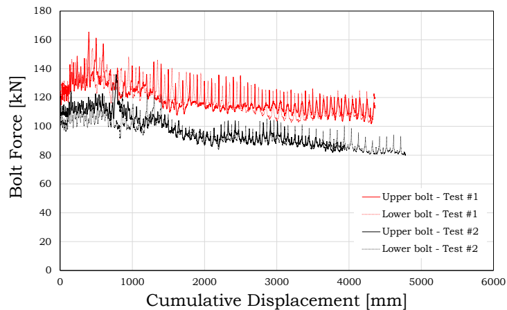
Fig. 2.13 – Bolt forces – M4
