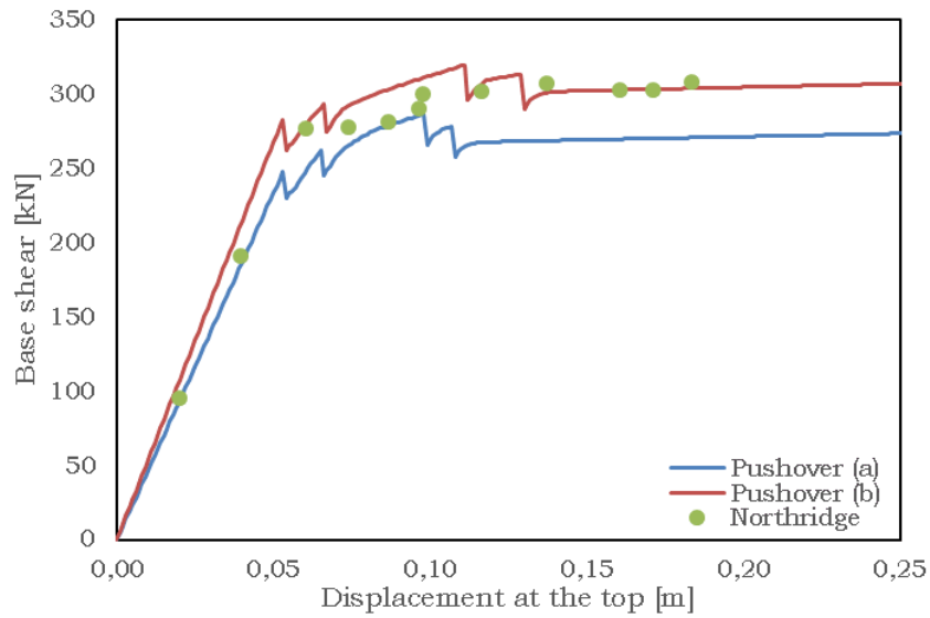
Fig. 5.124 – Base shear vs Displacement at the top – NORTHTRIDGE Max friction
