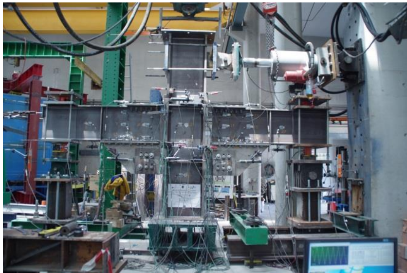
Fig. 4.75 – Setup of the test.
