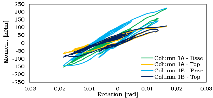
Fig. 5.202 – Columns hysteretic curves - RBS 1
