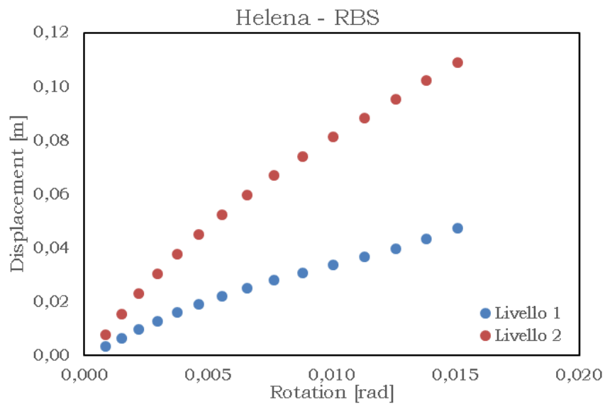
Fig. 5.85 – Displacement vs rotation – HELENA RBS
