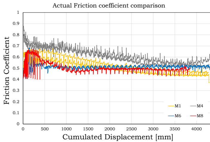
Fig. 2.21 – Comparisons: “Actual” friction coefficient vs cumulated displacement
