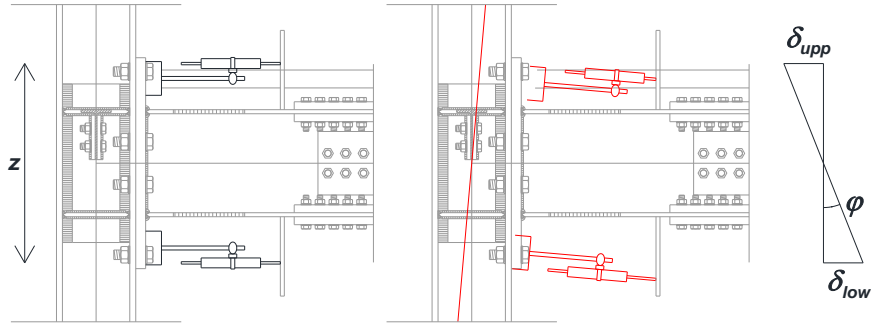
Fig. 5.191 – Transducers layout
