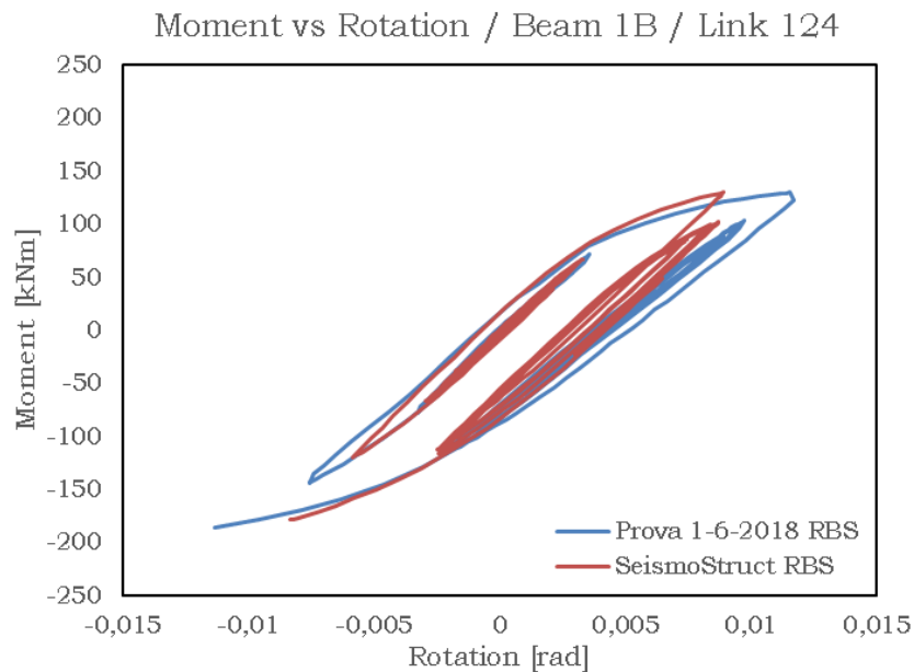
Fig. 5.195 – Moment vs rotation - Beam 1B - RBS 1
