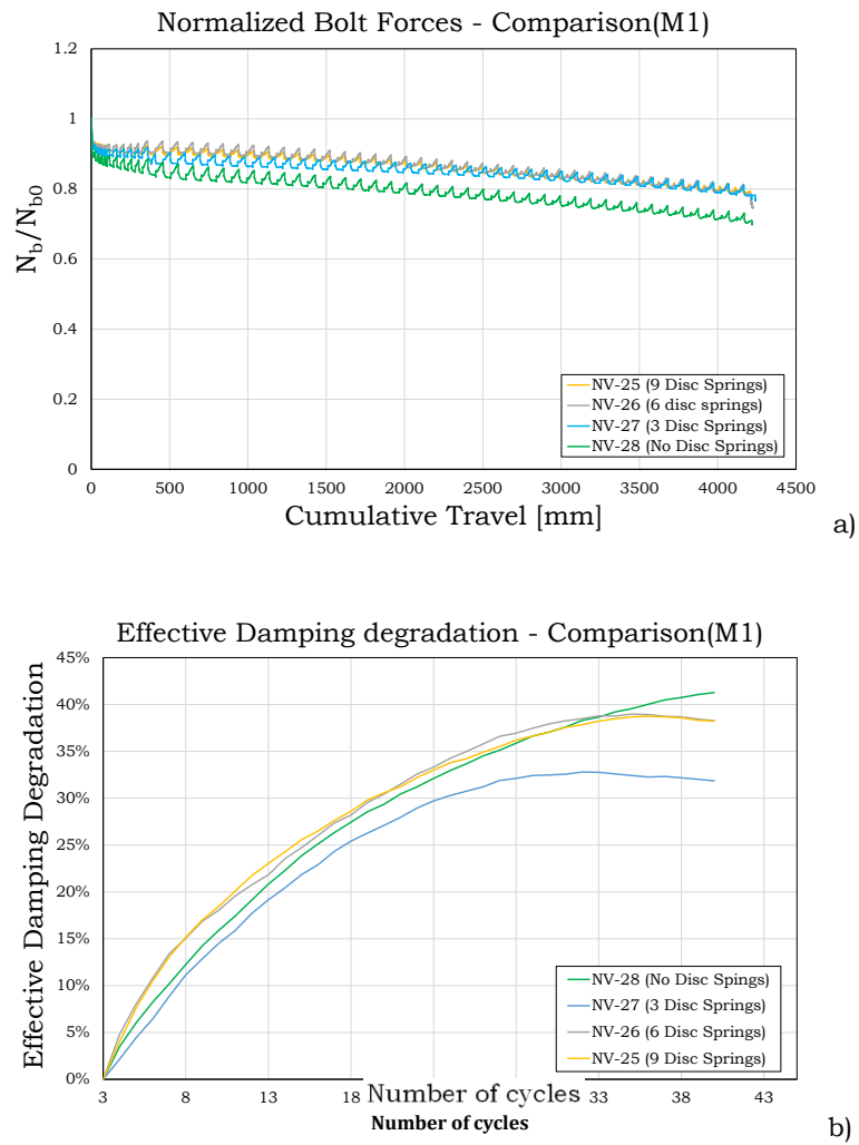
Fig. 2.36 – Bolts' preloading and effective damping for material M1
