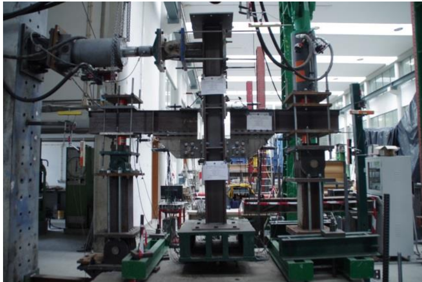
Fig. 4.43 – Setup of the test.
