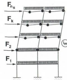
Fig. 5.5 – Mechanism type 2
