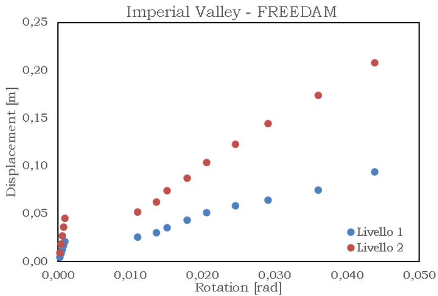
Fig. 5.93 – Displacement vs rotation – IMPERIAL VALLEY min friction
