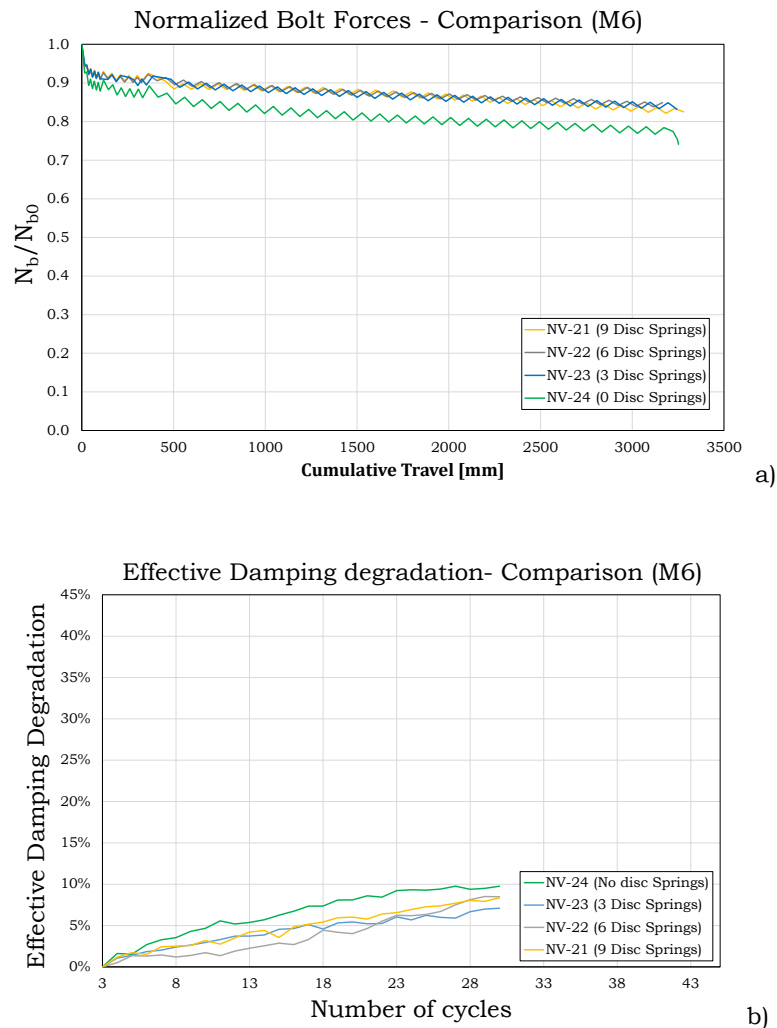
Fig. 2.38 – Bolts' preloading and effective damping for material M6
