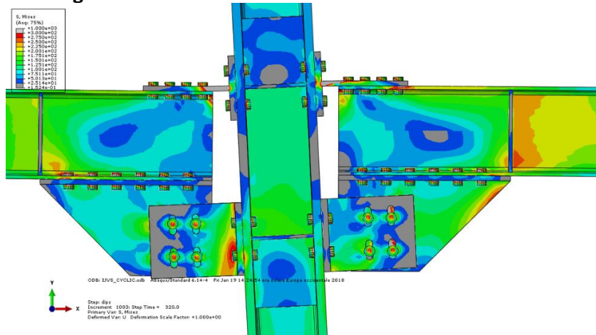
Fig. 4.109 – Stresses in the nodal area
