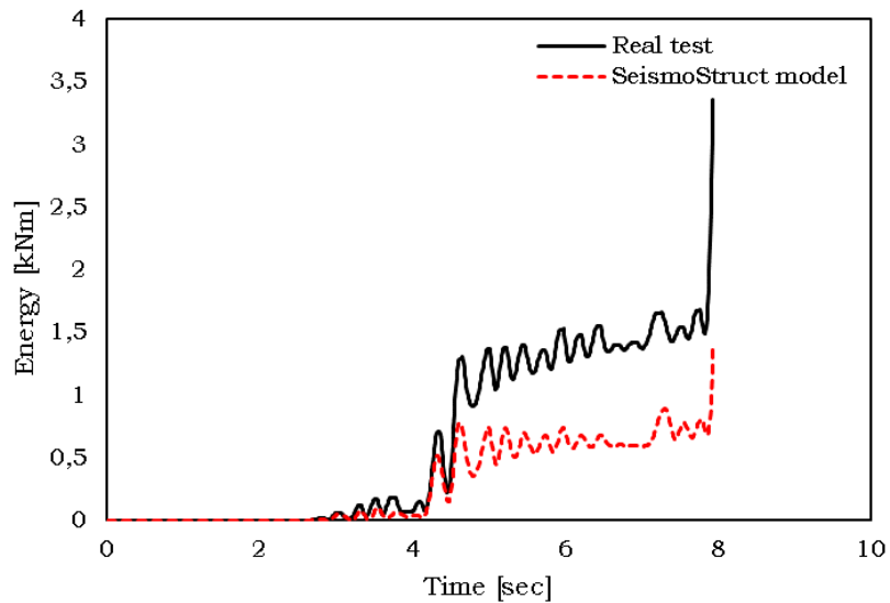
Fig. 5.207 – Energy vs time - Beam 1B - RBS 2
