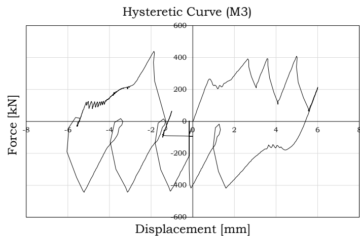
Fig. 2.9 – Hysteretic behaviour of soft materials: M3
