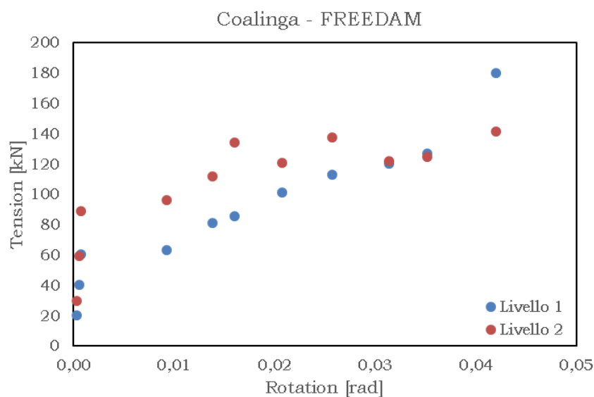
Fig. 5.71 – Tension vs rotation – COALINGA min friction
