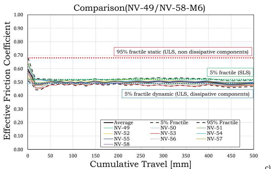
Fig. 4.1 – Design values of the friction coefficient (static or dynamic)
