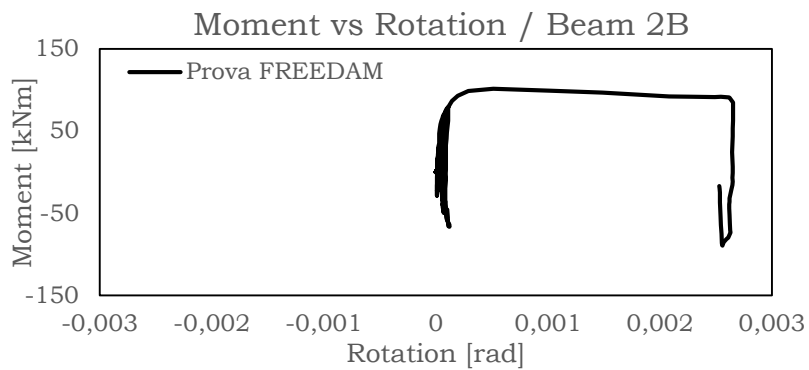
Fig. 5.222 - Moment vs rotation - Beam 2B - FREEDAM
