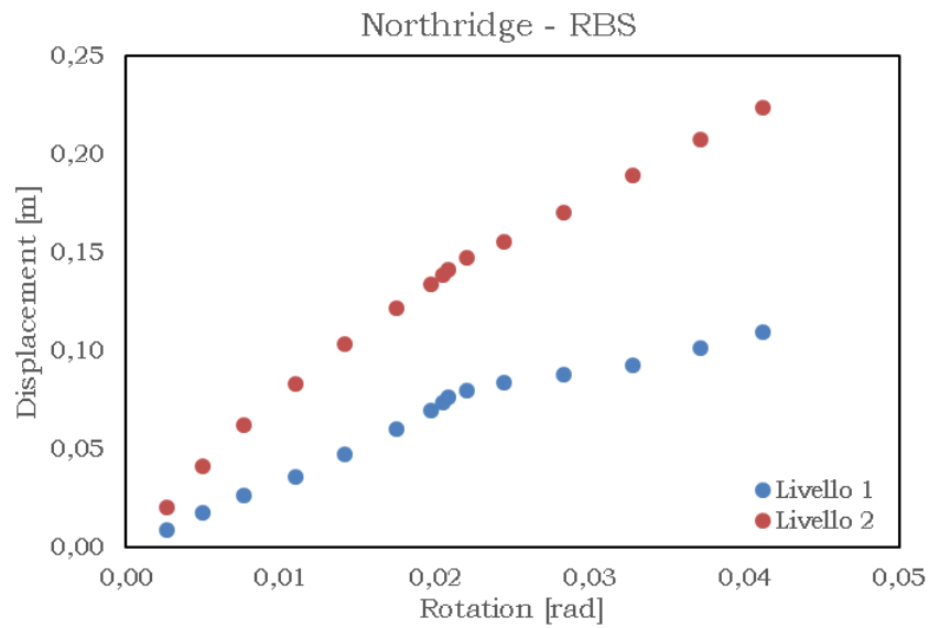
Fig. 5.133 – Displacement vs rotation – NORTHTRIDGE RBS
