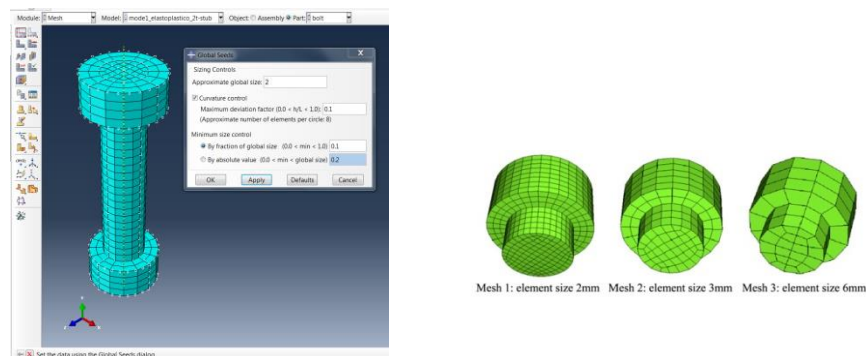
Fig. 4.94 – FE model - bolts
