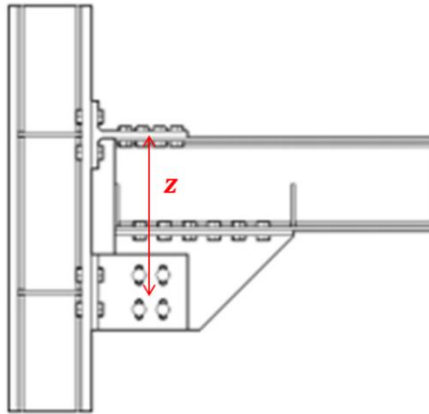
Fig. 5.29 – Lever arm scheme
