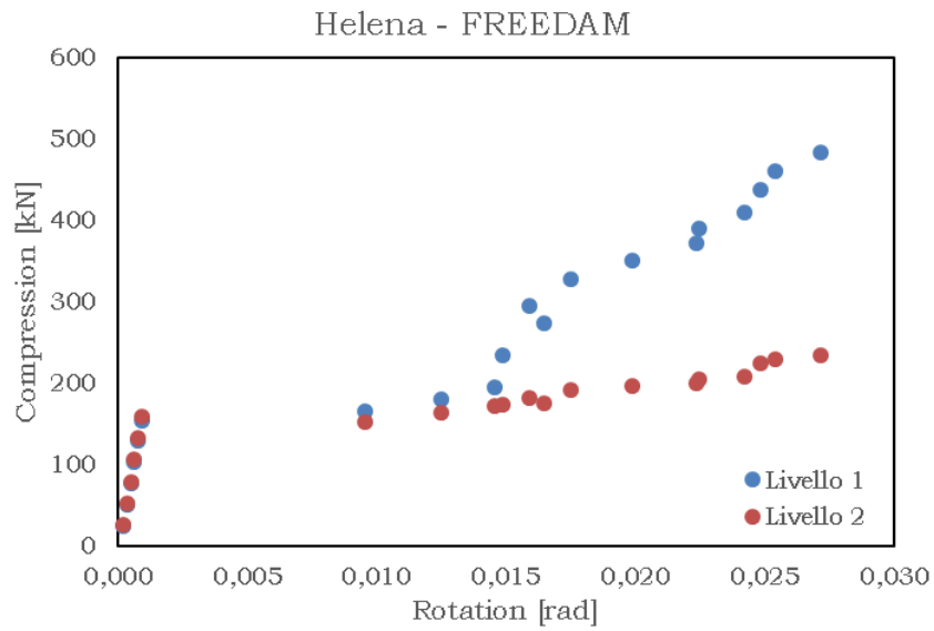
Fig. 5.82 – Compression vs rotation – HELENA min friction
