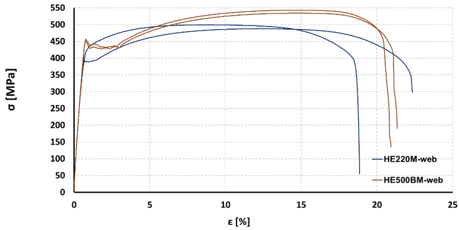
Fig. 4.23 – Stress-strain curves of the coupon tests from HE220M and HE500BM profile.
