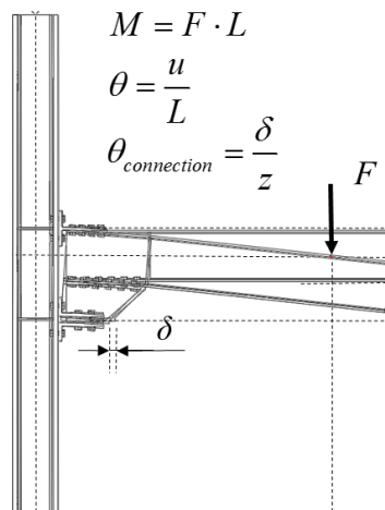
Fig. 4.99 – Static scheme for the evaluation of the bending moment
