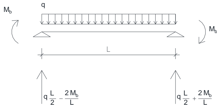
Fig. 5.19 – Scheme of the beam for the evaluation of the axial forces in the columns.
