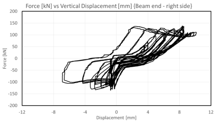
Fig. 4.41 – Force vs Vertical Displacement at the beam end - Right side
