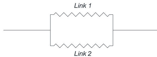
Fig. 5.51 – Plasticity model
