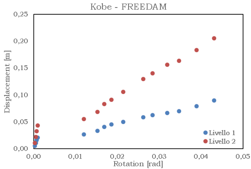
Fig. 5.105 – Displacement vs rotation – KOBE min friction
