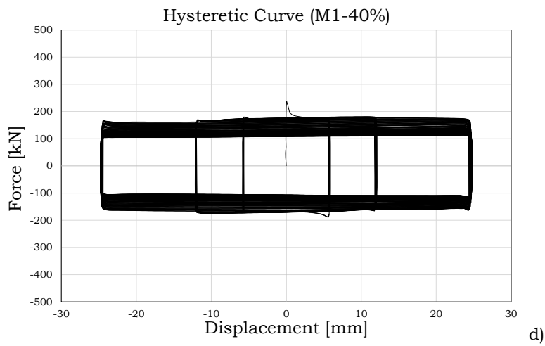
Fig. 2.25 – Influence of the bolts' pre-load over the force-displacement hysteretic response (M1)
