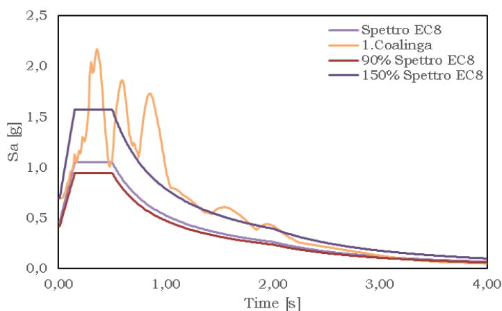
Fig. 5.169 – Spectral acceleration vs time - COALINGA
