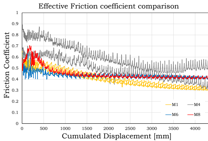
Fig. 2.22 – Comparisons: “Effective” friction coefficient vs cumulated displacement
