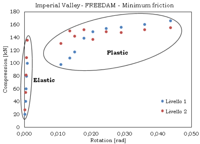
Fig. 5.165 – Compression vs rotation – FREEDAM min friction
