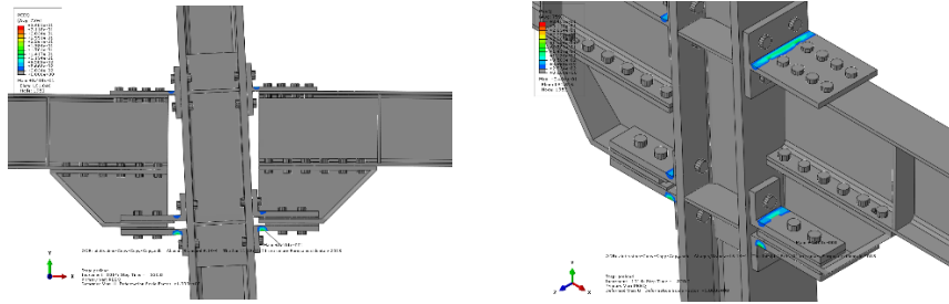
Fig. 4.100 – Plastic deformation in the connection
