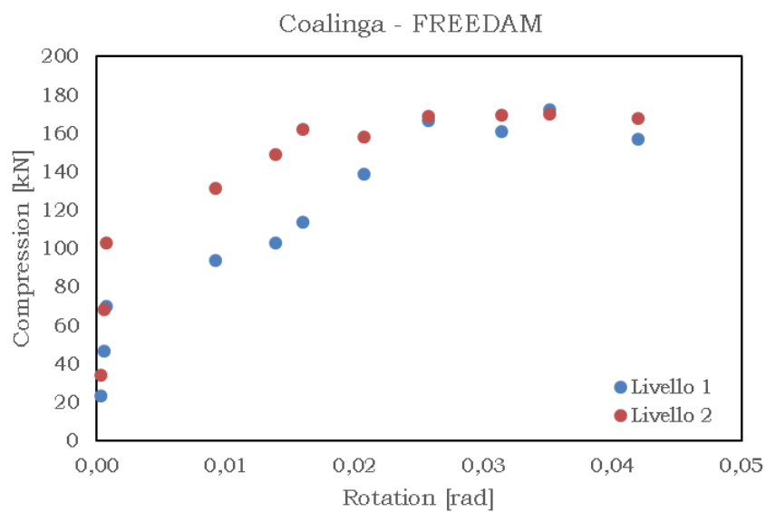
Fig. 5.70 – Compression vs rotation – COALINGA min friction
