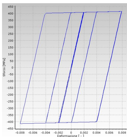
Fig. 5.48 – Hysteresis loops for Steel S355
