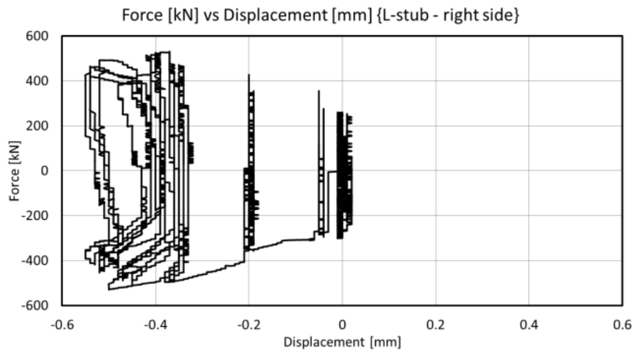
Fig. 4.83 – Force vs Relative displacement between L-stub and column - Right side
