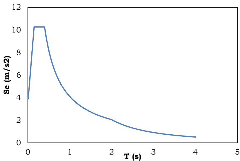
Fig. 5.21 – Spectrum according to Eurocode 8 [1]
