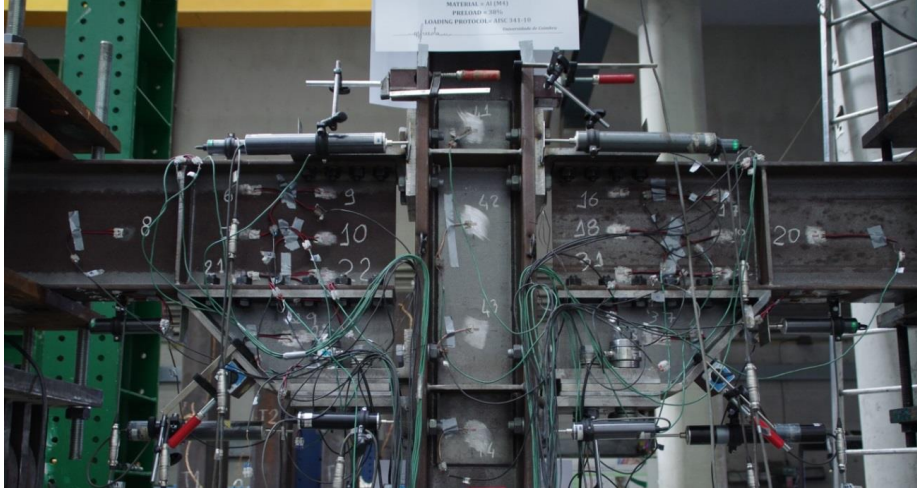
Fig. 4.18 – Sensors' layout
