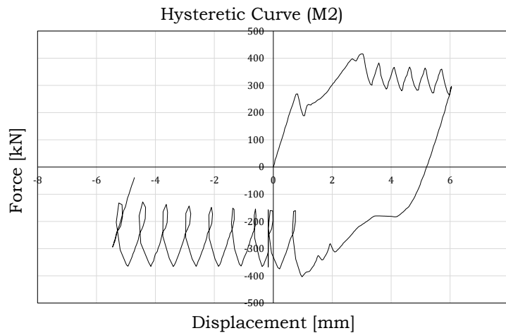
Fig. 2.8 – Hysteretic behaviour of soft materials: M2
