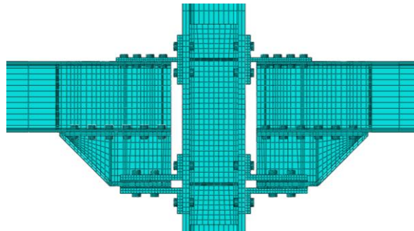
Fig. 4.93 – FE model - mesh
