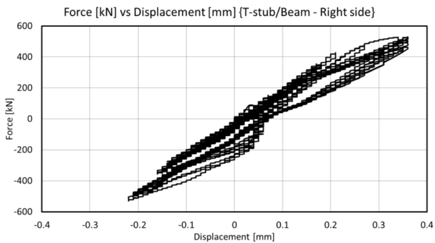
Fig. 4.85 – Force vs Relative displacement between T-stub and beam - Right side
