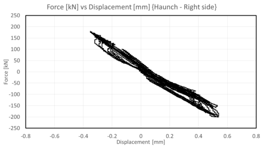
Fig. 4.55 – Force vs Relative displacement between Haunch and Beam - Right side
