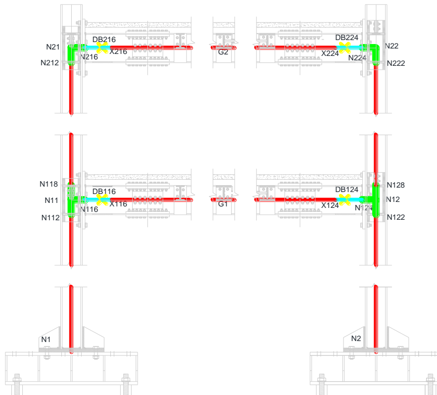
Fig. 5.56 – Seismostruct model
