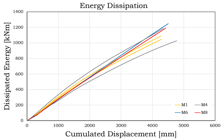
Fig. 2.23 – Energy dissipation capacity
