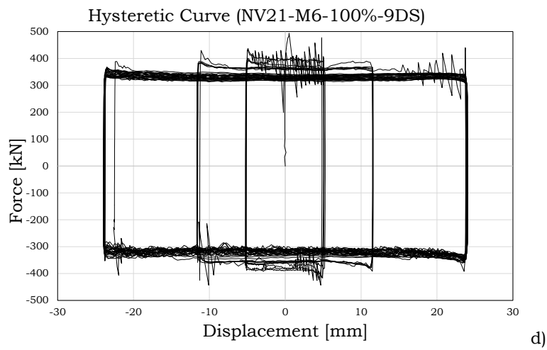
Fig. 2.35 – Influence of the disc spring configuration over the hysteretic response (M6)
