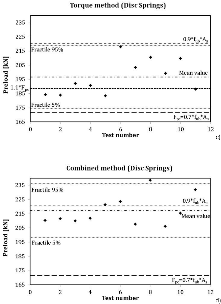
Fig. 3.6 – Summary of the tightening tests
