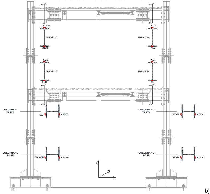
Fig. 5.180 – Stain gauges on frames
