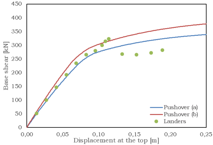
Fig. 5.120 - Base shear vs displacement at the top - LANDERS RBS
