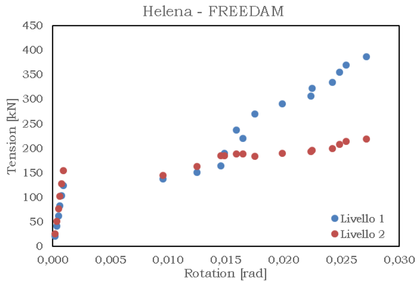
Fig. 5.83 – Tension vs rotation – HELENA min friction
