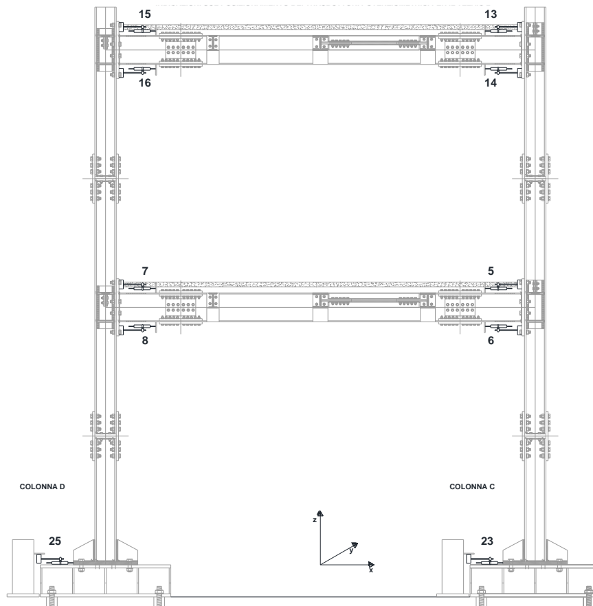
Fig. 5.179 – Displacement transducers on frames
