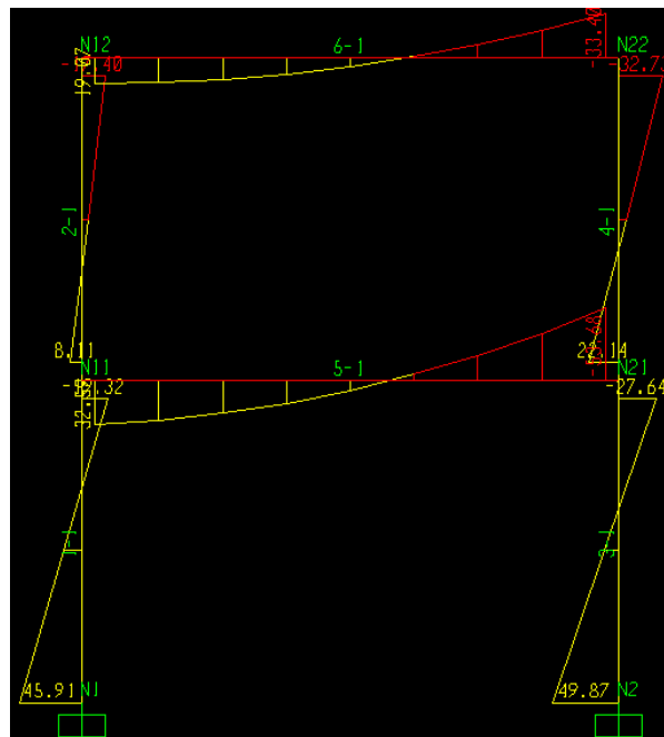
Fig. 5.24 – Bending moment for the check of the beams
