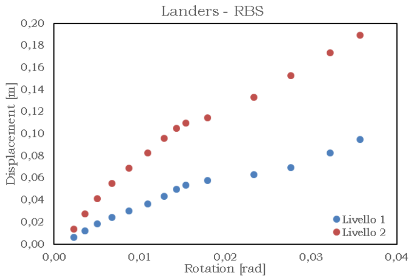
Fig. 5.121 - Displacement vs rotation - LANDERS RBS
