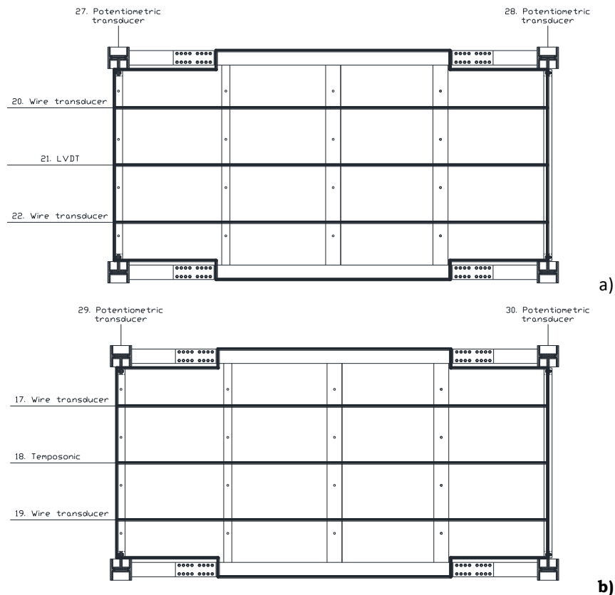
Fig. 5.178 – Transducers layout at the 1 st and 2 nd level
