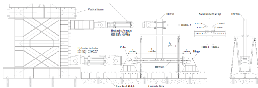
Fig. 5.57 – Test layout
