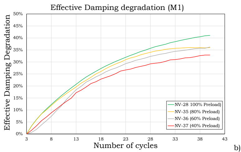
Fig. 2.29 – Bolts' preloading and effective damping for material M1
