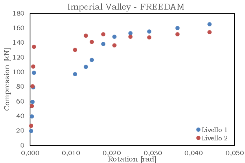
Fig. 5.94 – Compression vs rotation – IMPERIAL VALLEY min friction
