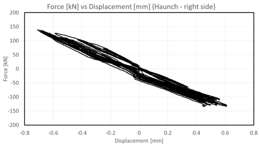
Fig. 4.39 – Force vs Relative displacement between Haunch and Beam - Right side
