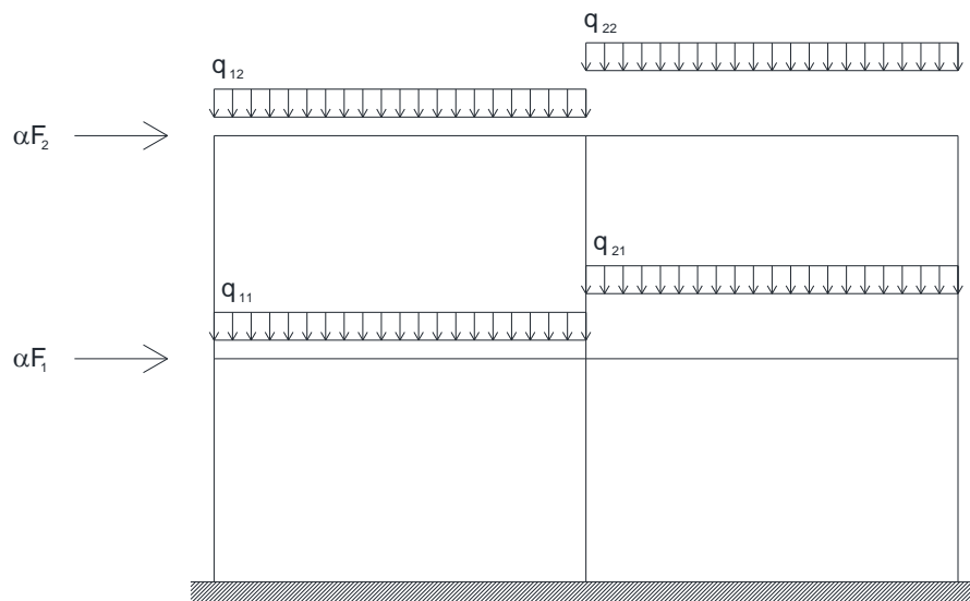
Fig. 5.10 – Two floors two spans frame
