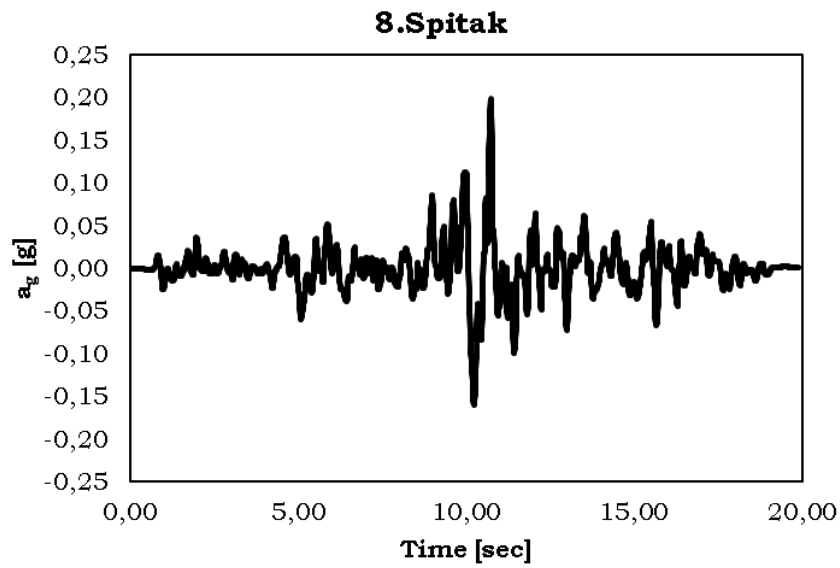
Fig. 5.43 – Spitak accelerogram
