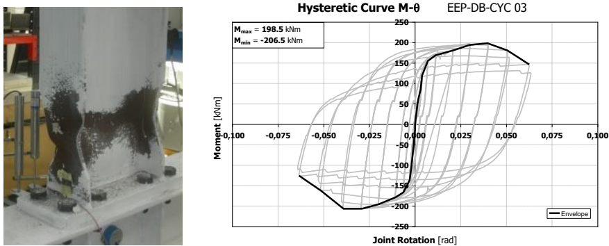
Fig. 5.28 – Cyclic behaviour of the beam-to-column joint with RBS tested in Iannone et al., (2008) [2]
