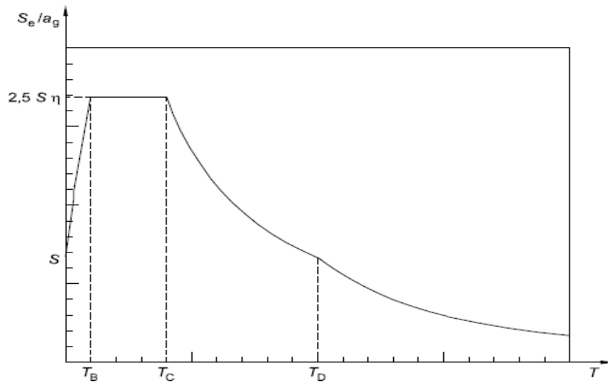
Fig. 5.44 - Elastic spectrum
