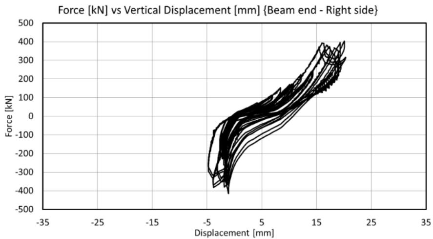
Fig. 4.73 – Force vs Vertical Displacement at the beam end - Right side
