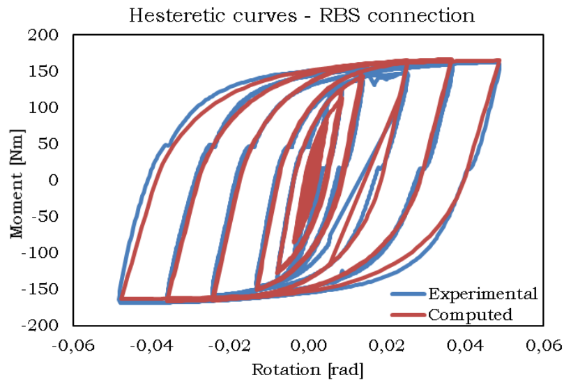
Fig. 5.59 – Hysteretic curves – RBS connection
