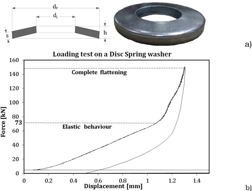
Fig. 3.4 – Disc Spring washers. a) Geometric features of a Disc Spring washer; b) Experimental behaviour of a disc spring washer
