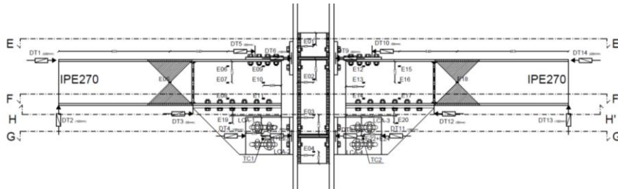
Fig. 4.19 – Sensors' layout scheme
