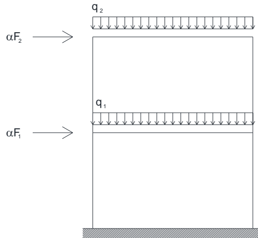
Fig. 5.12 – Two floors, single span frame with distributed and concentrated force.
