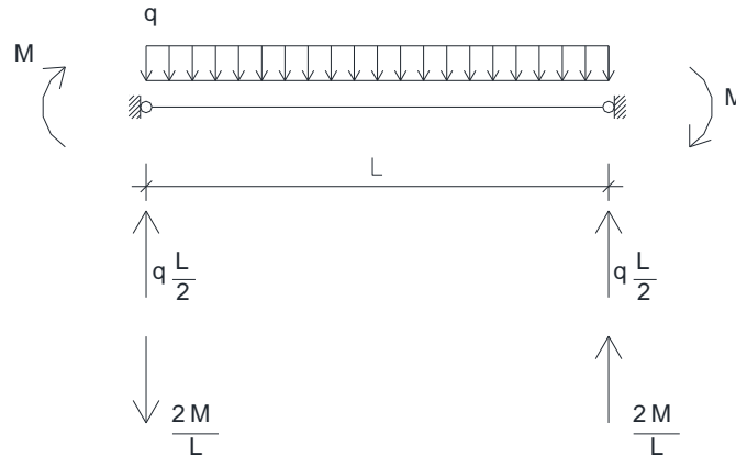
Fig. 5.20 – Static scheme that assure that the plastic hinges develop at the beam ends.
