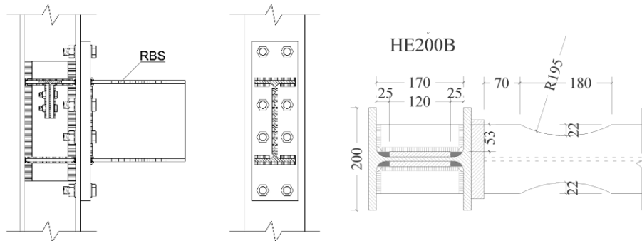
Fig. 5.26 – Benchmark case: Beam-to-Column Connection with RBS
