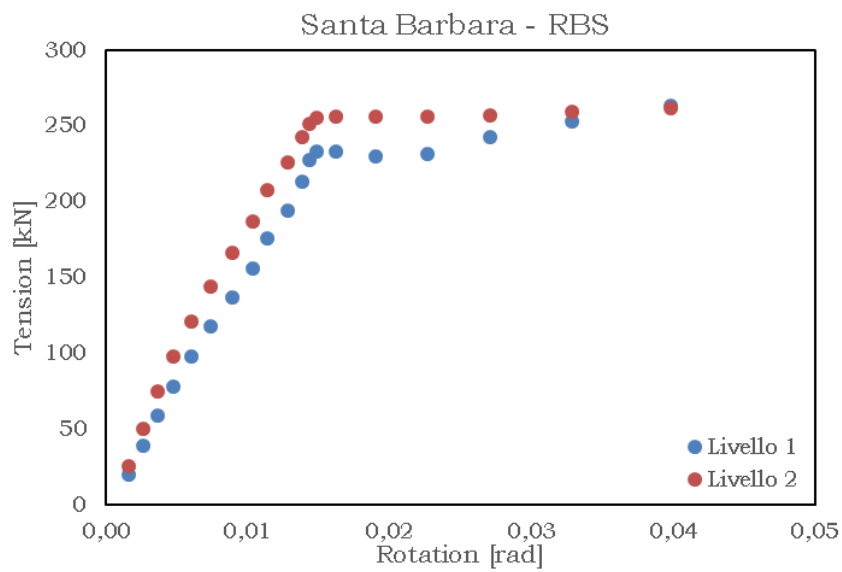
Fig. 5.147 – Tension vs rotation – SANTA BARBARA RBS
