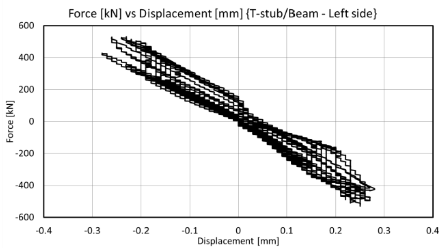
Fig. 4.84 – Force vs Relative displacement between T-stub and beam - Left side.
