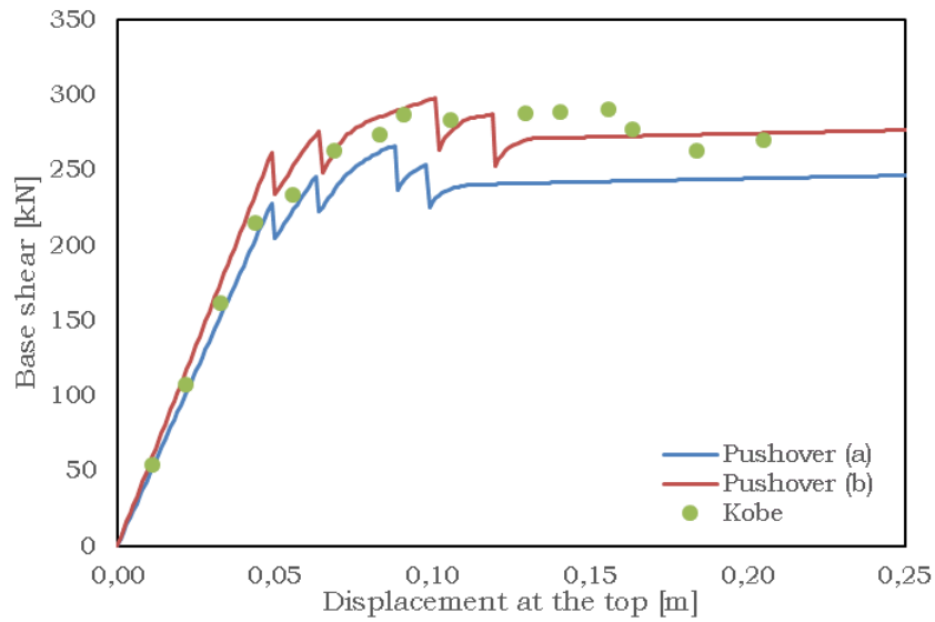
Fig. 5.104 – Base shear vs Displacement at the top – KOBE min friction
