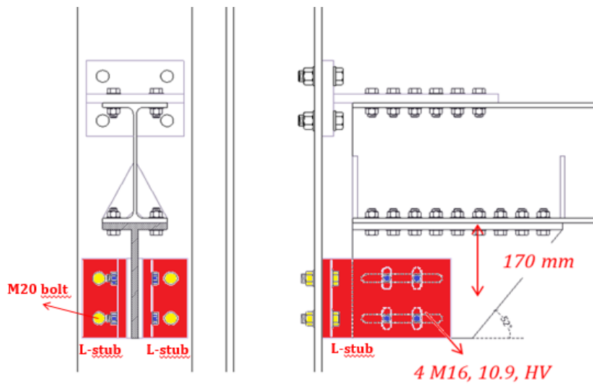
Fig. 5.35 – L-stubs
