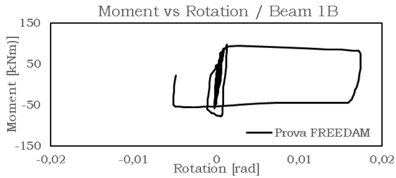
Fig. 5.218 – Moment vs rotation – Beam 1B – FREEDAM
