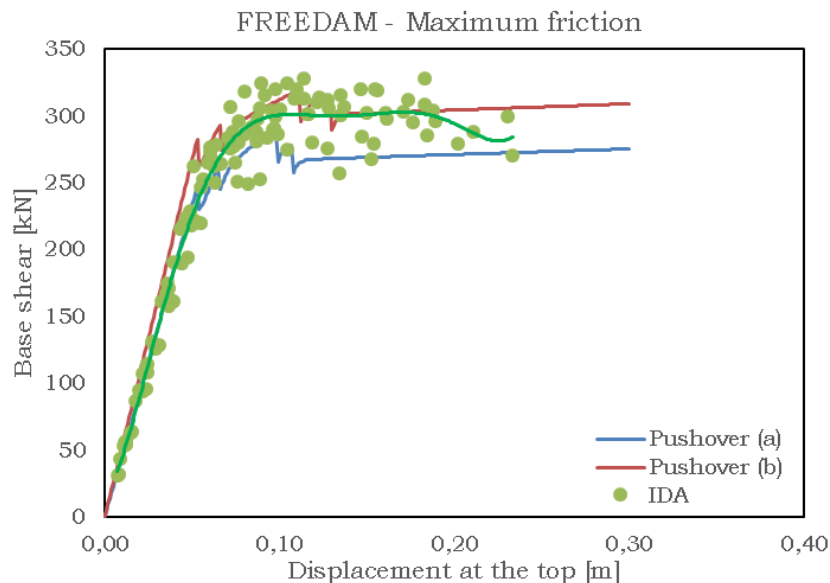
Fig. 5.161 – Base shear vs displacement – FREEDAM Max. friction
