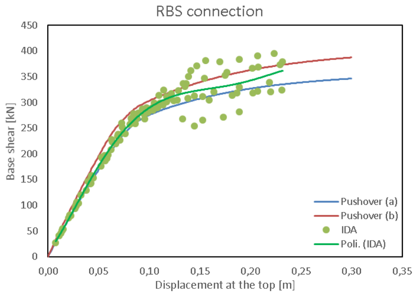
Fig. 5.163 – Base shear vs displacement - RBS
