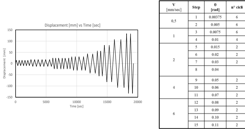
Fig. 4.98 – Loading protocol according to AISC 341/2010 [2]
