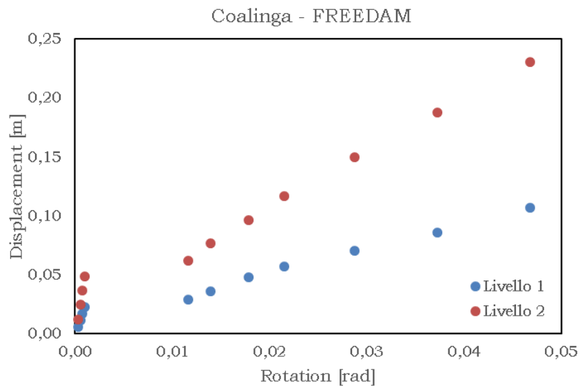
Fig. 5.65 - Displacement vs rotation – COALINGA Max friction
