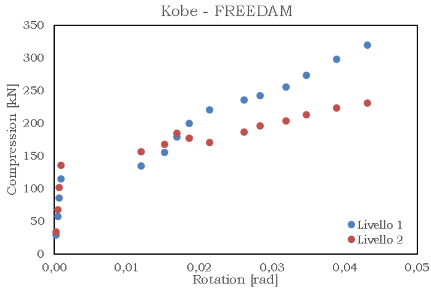
Fig. 5.106 – Compression vs rotation – KOBE min friction
