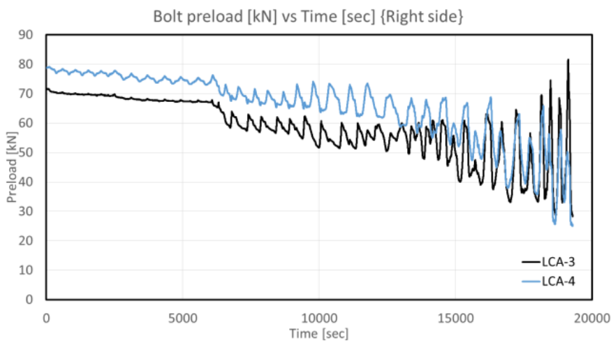
Fig. 4.33 – Bolt preload vs Time - Right side
