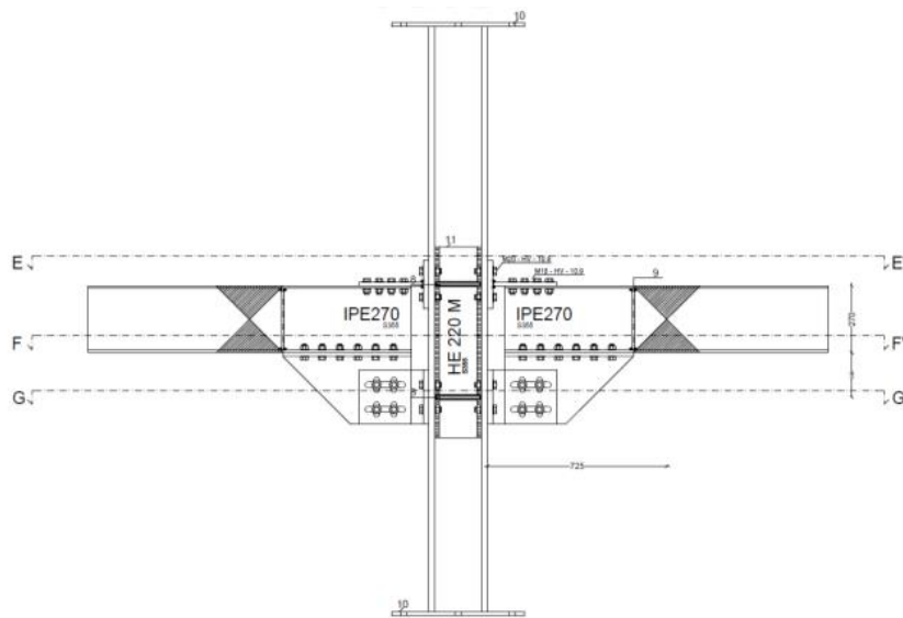
Fig. 4.11 – Internal joint configuration (HE220M / IPE270 - Vertical pads)
