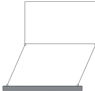
Fig. 5.17 – Index of mechanism 1 - Mechanism type-3.
