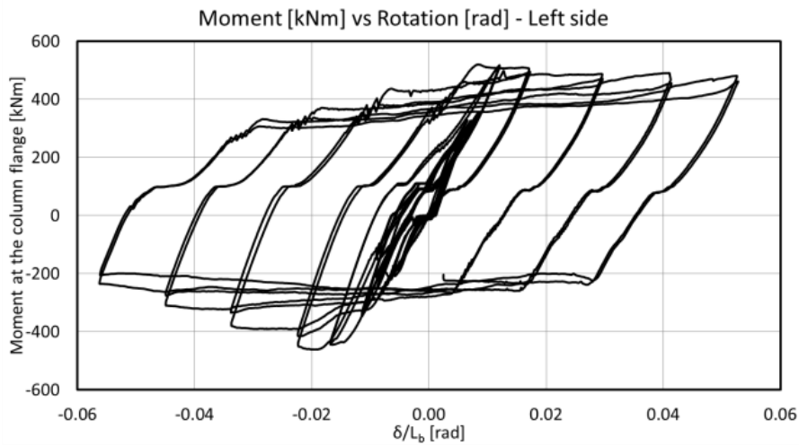
Fig. 4.76 – Moment evaluated at the column's face vs chord rotation – Left side of the joint.
