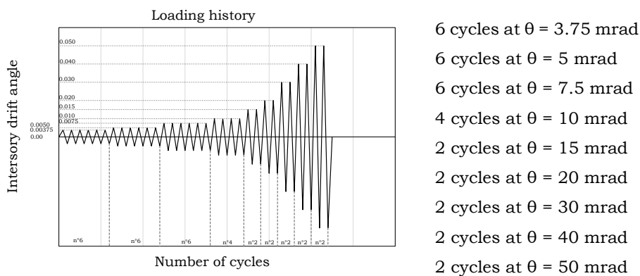
Fig. 4.16 – Loading protocol according to AISC 341/2010 [2]
