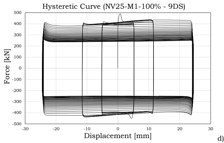
Fig. 2.33 – Influence of the disc spring configuration over the hysteretic response (M1)
