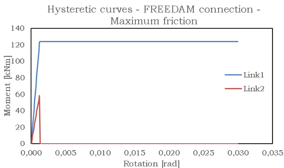
Fig. 5.53 – Hysteretic curves - FREEDAM connection – maximum friction
