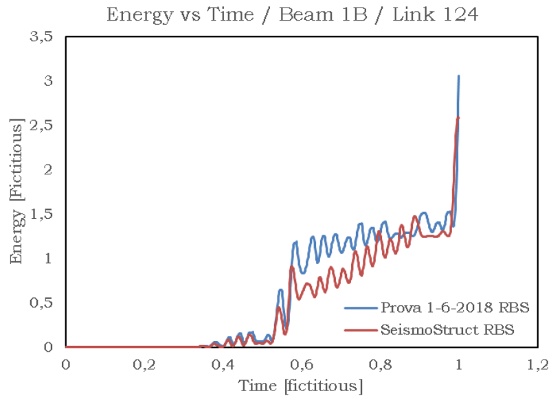
Fig. 5.196 – Energy vs time - Beam 1B- RBS
