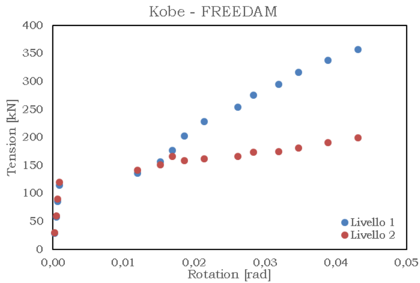
Fig. 5.107 – Tension vs rotation – KOBE min friction
