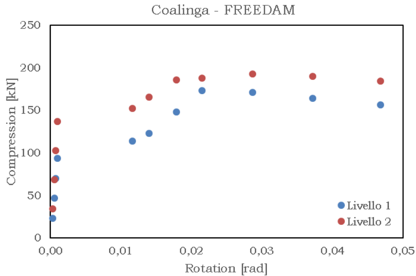
Fig. 5.66 – Compression vs rotation – COALINGA Max friction
