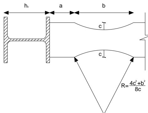
Fig. 5.27 – Design parameters for RBS connections
