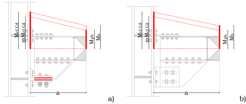
Fig. 4.4 – Distance between the axis of the beam plastic hinge and the column flange: a) configuration n.1; b) configuration n.2
