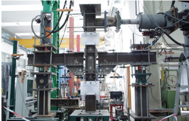
Fig. 4.96 – Specimen during the test
