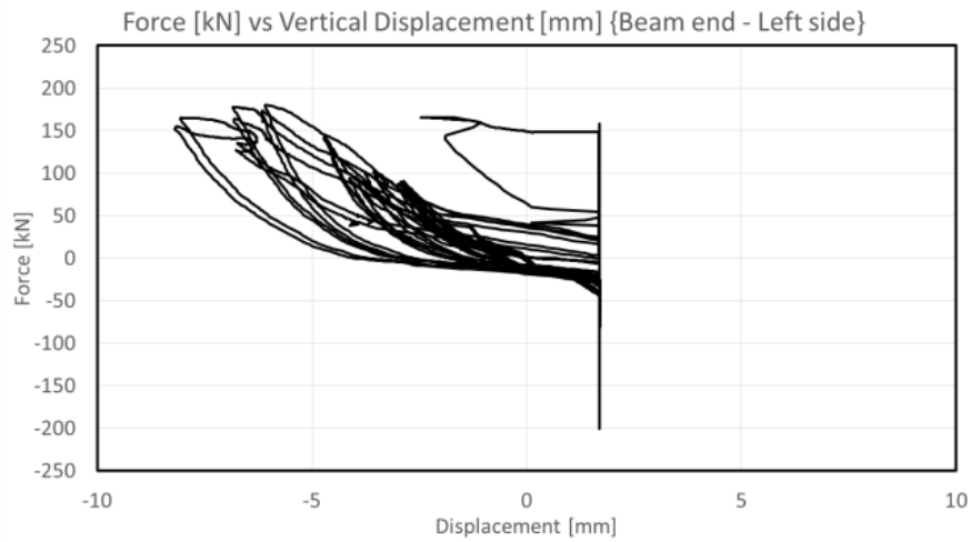
Fig. 4.56 – Force vs Vertical Displacement at the beam end - Left side.
