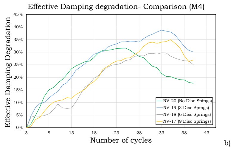
Fig. 2.37 – Bolts' preloading and effective damping for material M4
