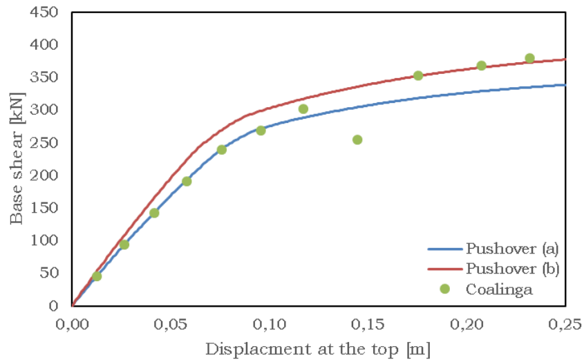
Fig. 5.72 – Base shear vs displacement at the top – COALINGA RBS
