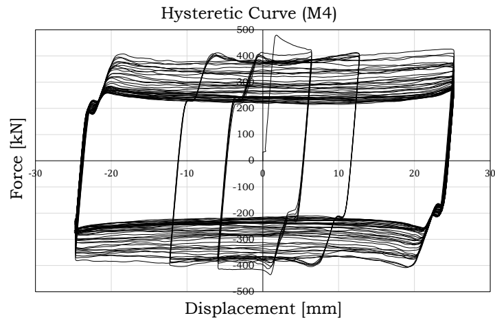
Fig. 2.11 – Hysteretic behaviour of soft materials: M4
