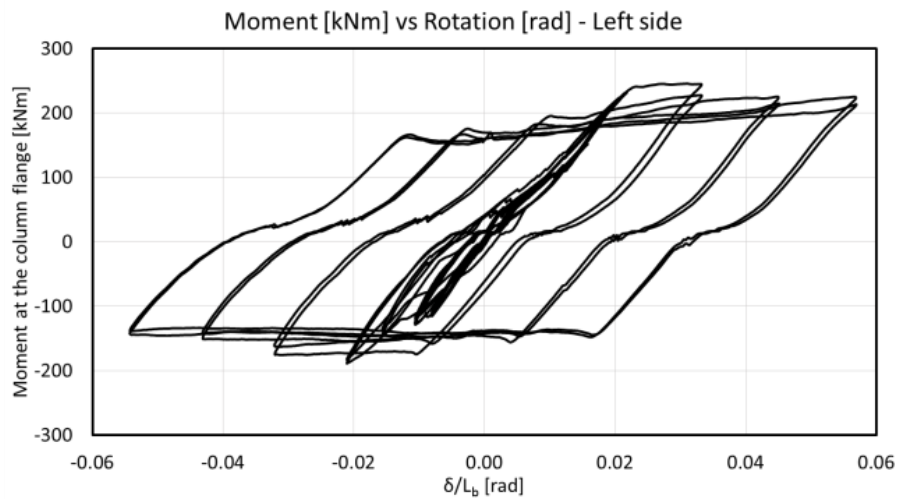
Fig. 4.44 – Moment evaluated at the column's face vs chord rotation – Left side of the joint.
