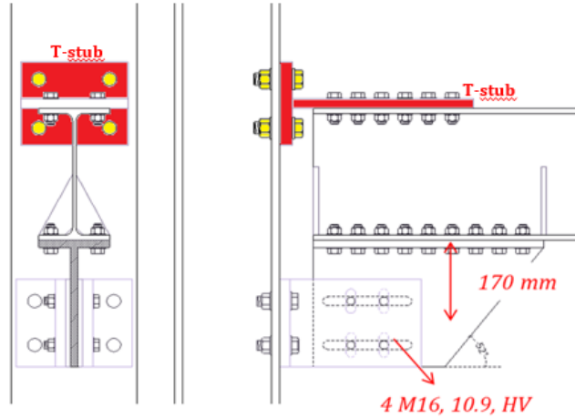
Fig. 5.31 – Geometrical parameters –T-stub
