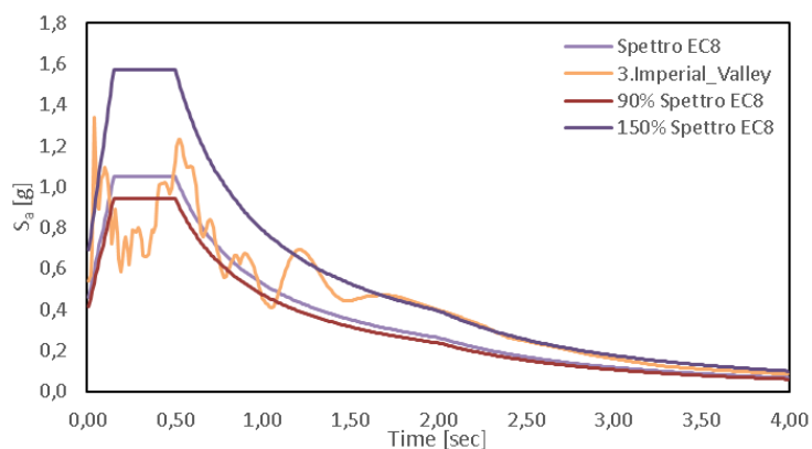
Fig. 5.170 – Spectral acceleration vs time – IMPERIAL VALLEY
