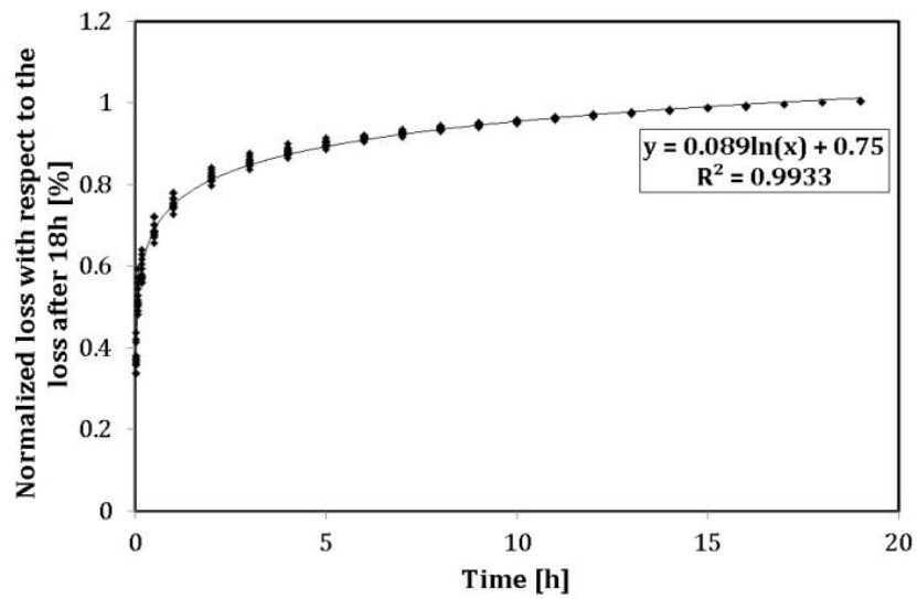
Fig. 3.8 – Regression curves of short term relaxation tests (Disc Springs) normalised with respect to the loss occurred in fixed time instants a) 1h; b) 6h; c) 12h; d) 18h.
