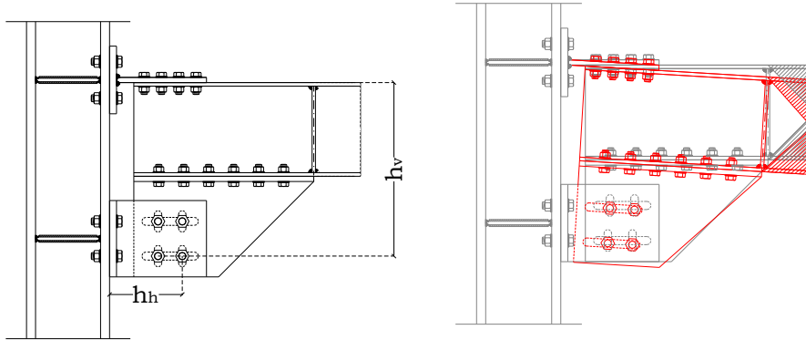
Fig. 4.8 – Rigid deformation of the FREEDAM-CYC02 joint
