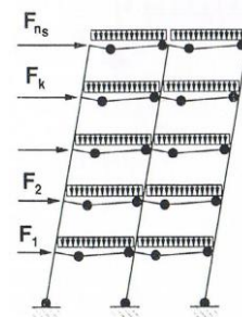
Fig. 5.7 – Global mechanism
