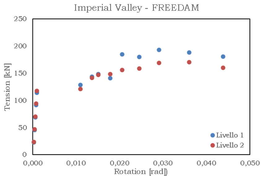
Fig. 5.95 – Tension vs rotation – IMPERIAL VALLEY min friction
