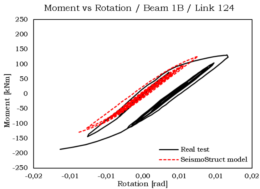
Fig. 5.206 – Moment vs rotation - Beam 1B - RBS 2
