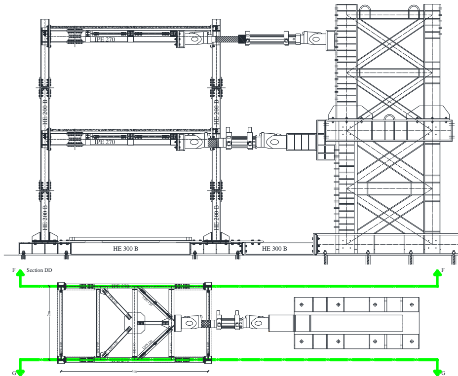
Fig. 5.176 – Experimental test set-up
