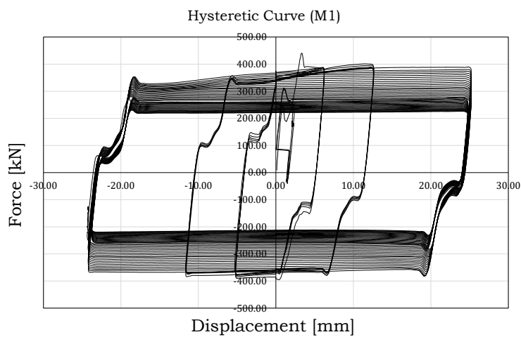
Fig. 2.10 – Hysteretic behaviour of soft materials: M1
