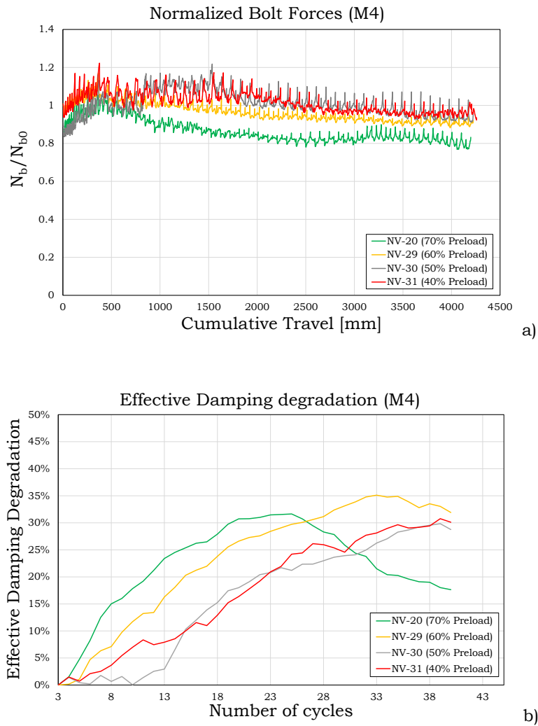
Fig. 2.30 – Bolts' preloading and effective damping for material M4
