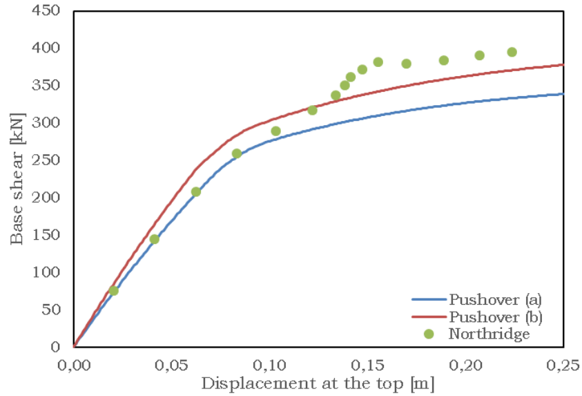
Fig. 5.132 – Base shear vs displacement at the top – NORTHTRIDGE RBS
