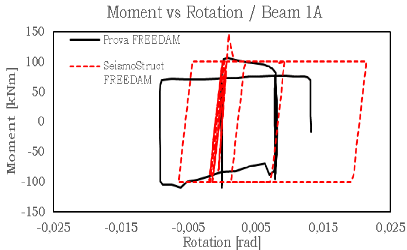
Fig. 5.216 – Moment vs rotation – Beam 1A- FREEDAM
