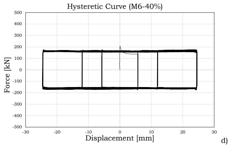
Fig. 2.27 – Influence of the bolts' pre-load over the force-displacement hysteretic response (M6)
