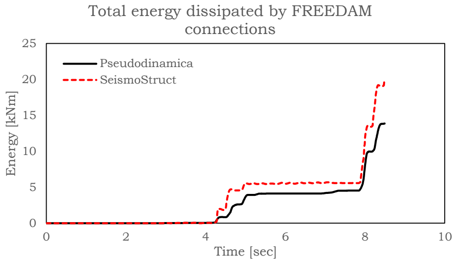
Fig. 5.224 – Total energy dissipated by FREEDAM connections
