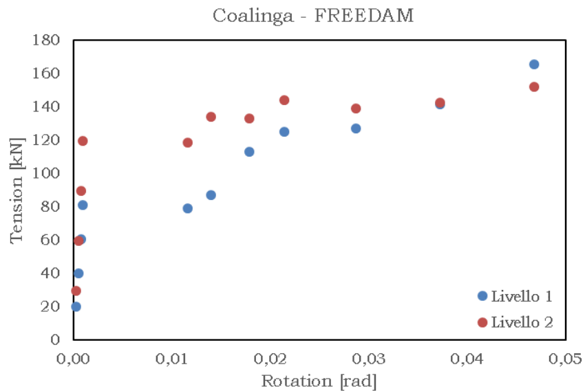
Fig. 5.67 – Tension vs rotation – COALINGA Max friction
