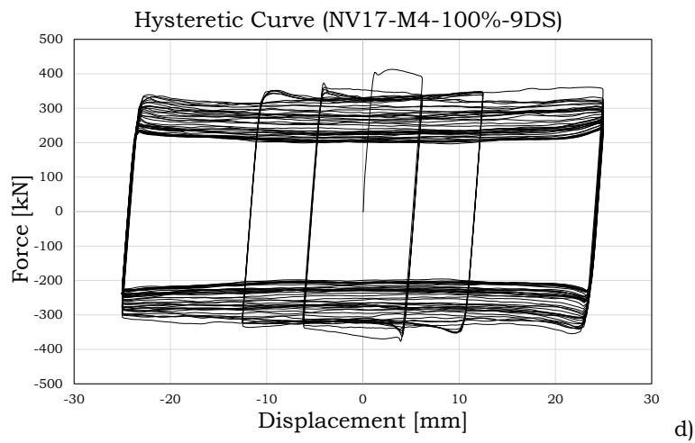
Fig. 2.34 – Influence of the disc spring configuration over the hysteretic response (M4)
