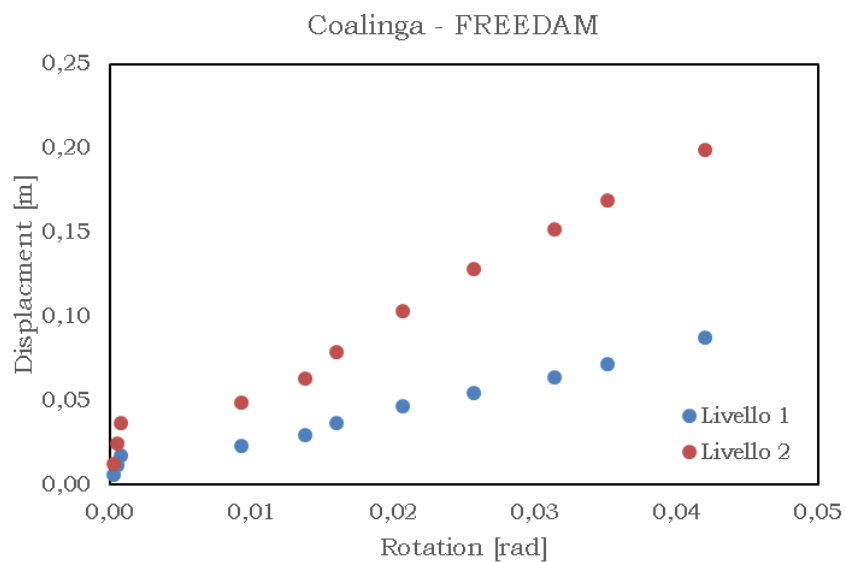
Fig. 5.69 – Displacement vs rotation – COALINGA min friction
