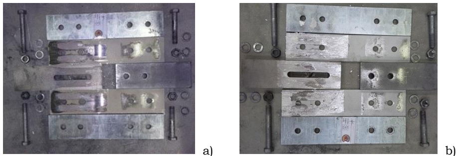
Fig. 2.14 – Damage of the interfaces: a) M1; b) M4
