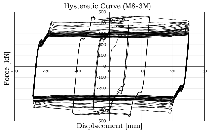
Fig. 2.17 – Hysteretic behaviour of hard materials: 3M friction shims
