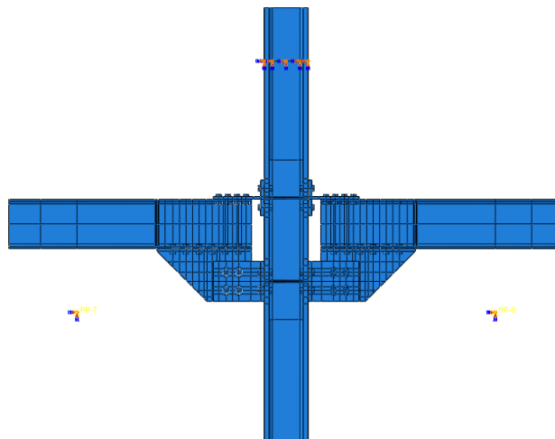
Fig. 4.92 – FE model of the Internal joint equipped with FREEDAM connection
