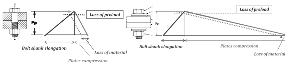
Fig. 2.32 – Effect of disc springs
