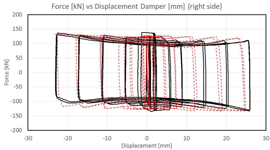
Fig. 4.105 – Comparison between experimental results and FE model (Damper-Right side)
