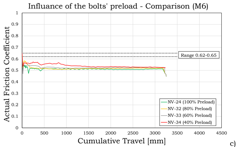
Fig. 2.28 – Influence of the bolts' pre-load over the actual friction coefficient
