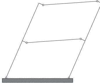
Fig. 5.15 – Index of mechanism 1 - Mechanism type-2 (Coincident with global mechanism).
