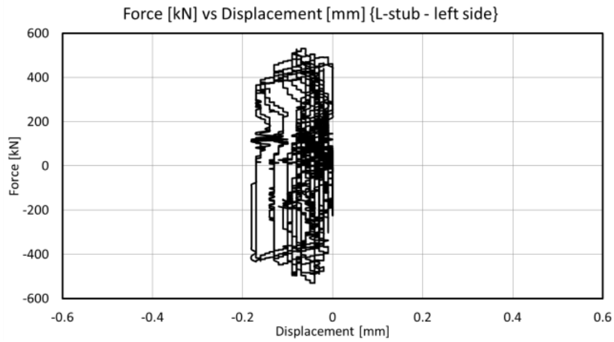
Fig. 4.82 – Force vs Relative displacement between L-stub and column - Left side
