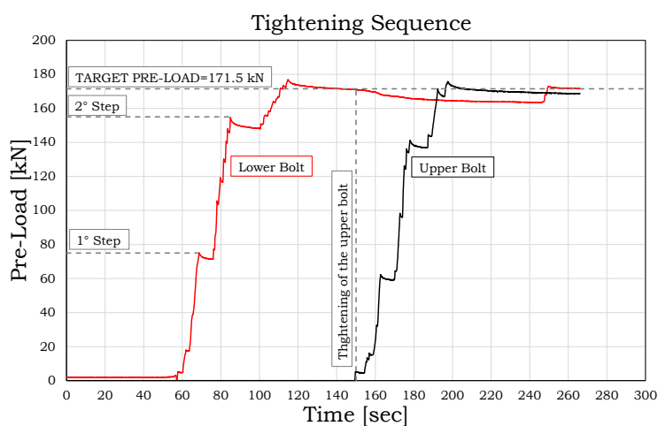
Fig. 2.6 – Tightening sequence
