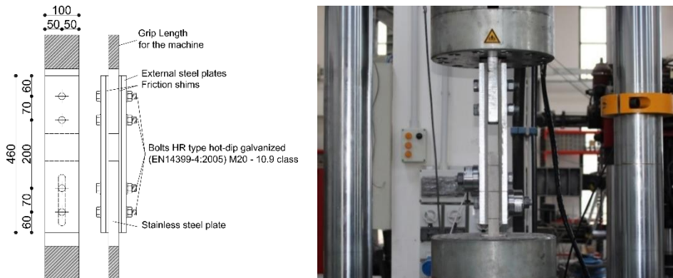
Fig. 2.5 – a) Typical layout of a specimen; b) Specimen in the testing machine
