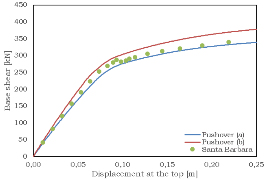
Fig. 5.144 – Base shear vs displacement at the top – SANTA BARBARA RBS
