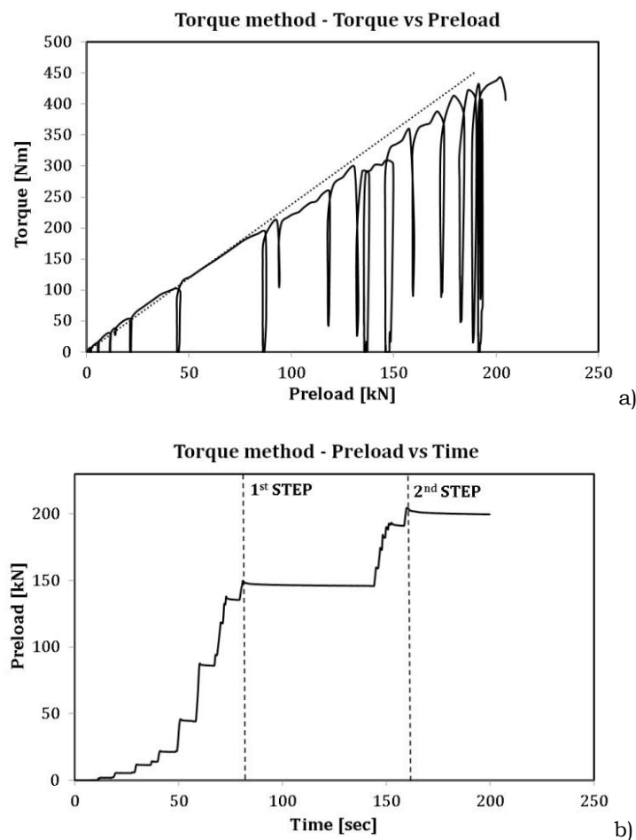
Fig. 3.5 – Examples of tightening sessions
