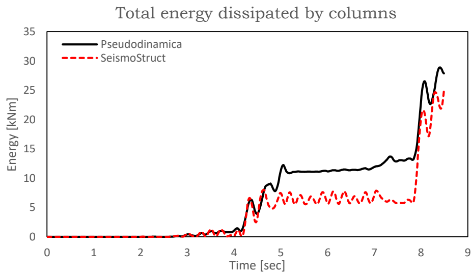
Fig. 5.225 – Total energy dissipated by FREEDAM connections
