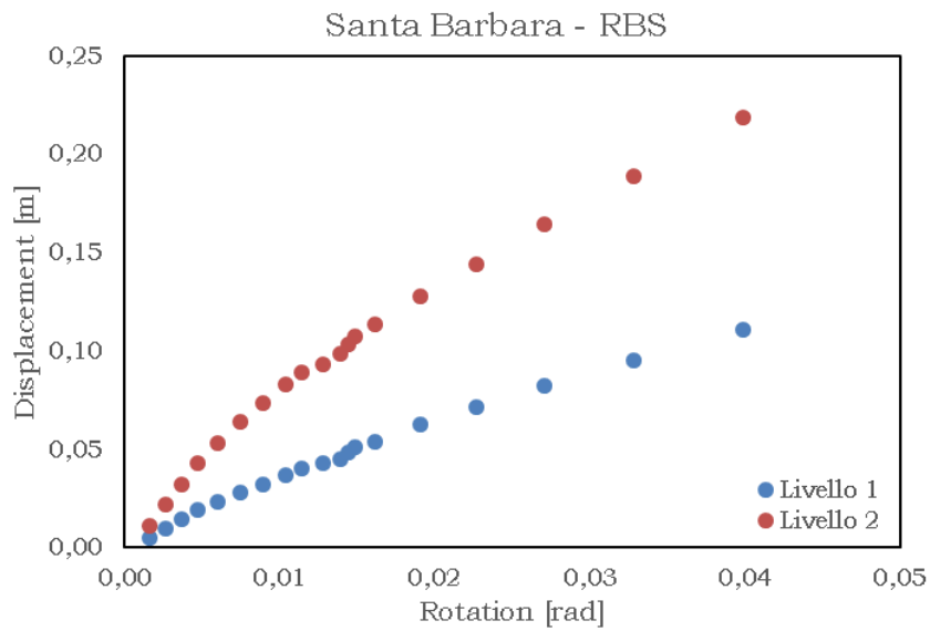
Fig. 5.145 – Displacement vs rotation – SANTA BARBARA RBS
