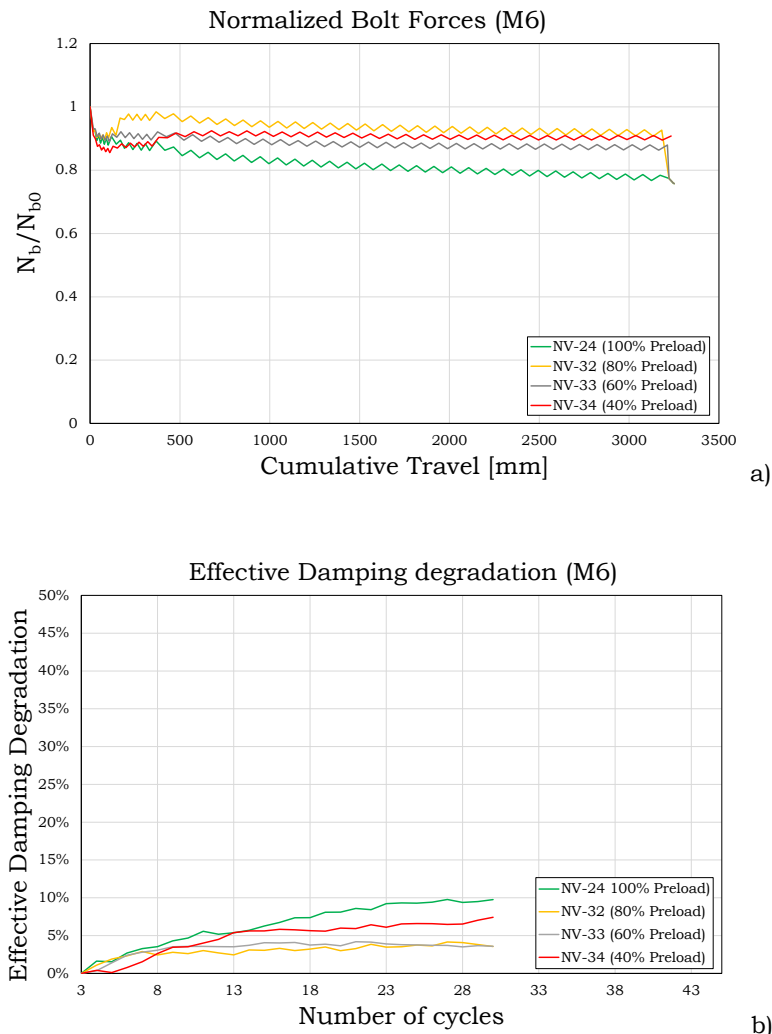
Fig. 2.31 – Bolts' preloading and effective damping for material M6
