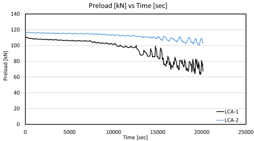
Fig. 4.80 – Bolt preload vs Time - Left side
