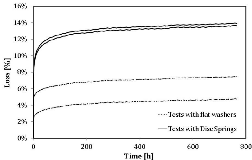
Fig. 3.9 – Medium-term relaxation tests results
