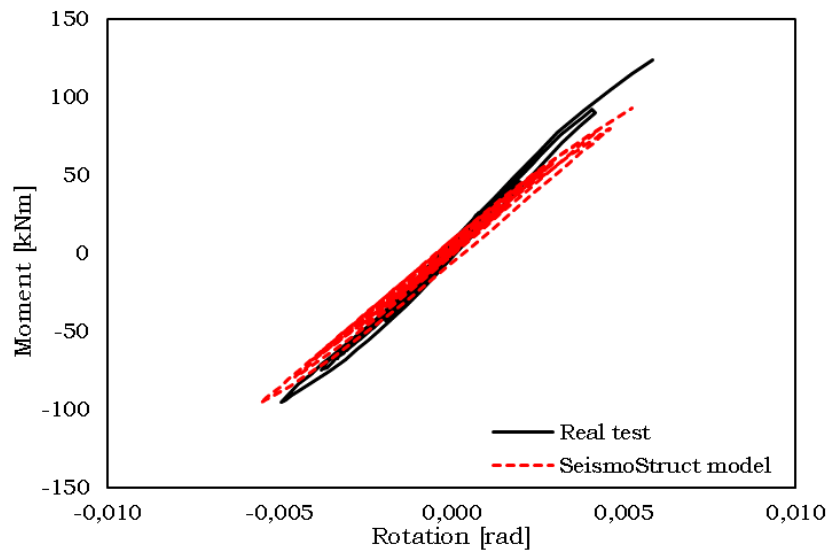
Fig. 5.208 – Moment vs rotation - Beam 2A - RBS 2
