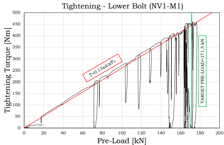
Fig. 2.7 – Typical Torque vs Pre-load diagram
