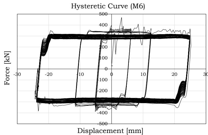
Fig. 2.15 – Hysteretic behaviour of hard materials: Carbide M6
