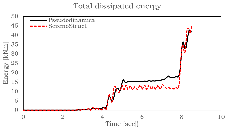
Fig. 5.226 – Total dissipated energy
