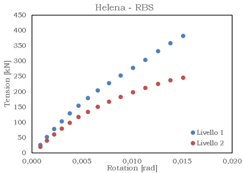
Fig. 5.87 – Tension vs rotation – HELENA RBS
