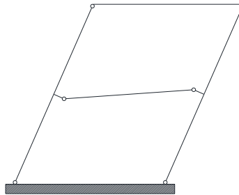
Fig. 5.14 – Index of mechanism 2 - Mechanism type-1.
