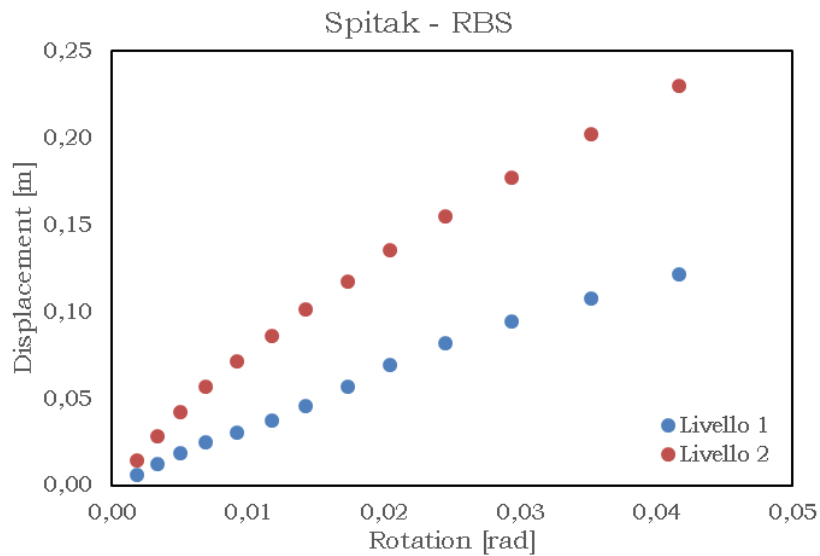
Fig. 5.157 – Displacement vs rotation – SPITAK RBS
