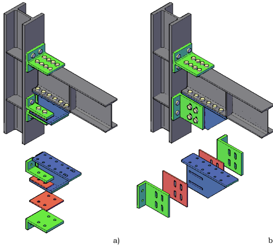
Fig. 4.2 – FREEDAM joint configurations: a) horizontal friction device; b) vertical friction device
