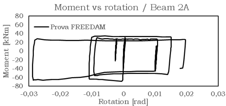
Fig. 5.220 – Moment vs rotation – Beam 2A – FREEDAM
