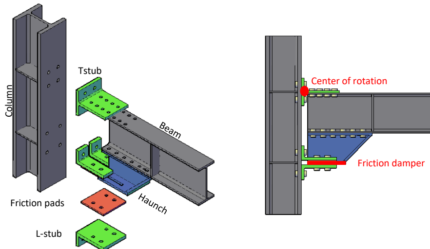
Fig. 2.1 – FREEDAM connection
