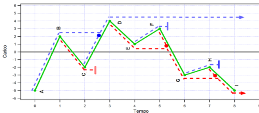
Fig. 5.168 – Rainflow scheme
