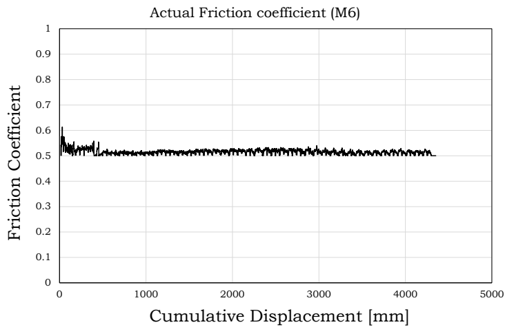
Fig. 2.20 – "Actual" friction coefficient vs cumulative travel: M6
