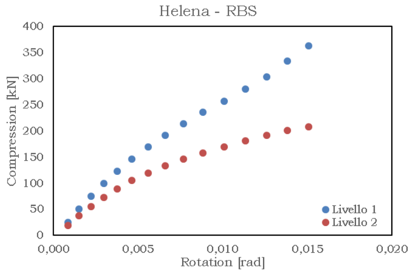
Fig. 5.86 – Compression vs rotation – HELENA RBS
