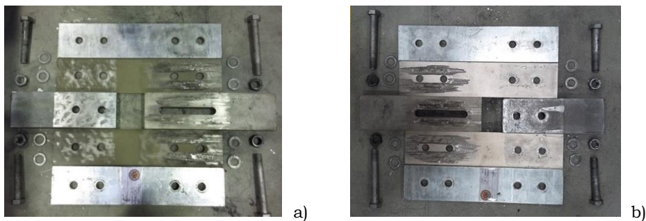
Fig. 2.18 – Damage of the interfaces: a) M6; b) 3M friction shims
