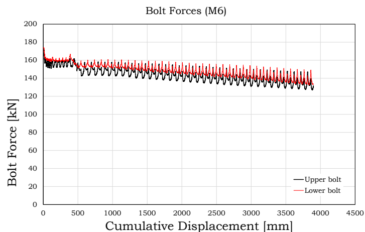
Fig. 2.19 – Typical diagrams of the bolt forces
