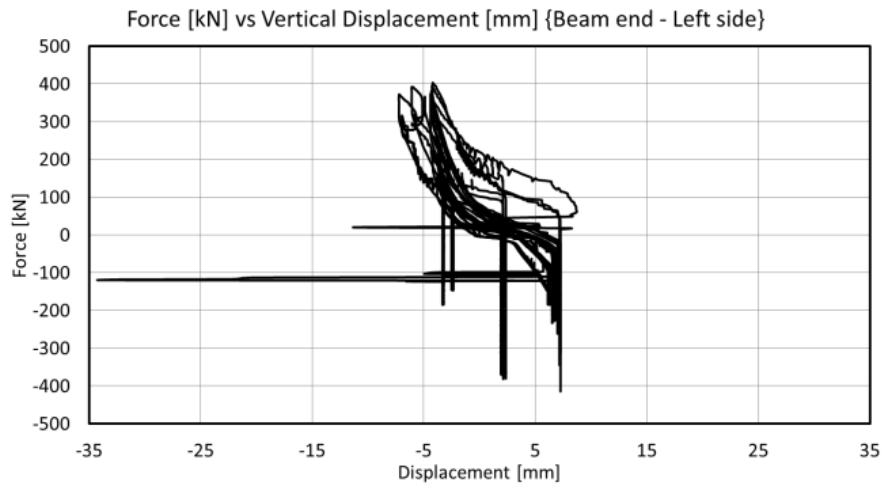
Fig. 4.72 – Force vs Vertical Displacement at the beam end - Left side
