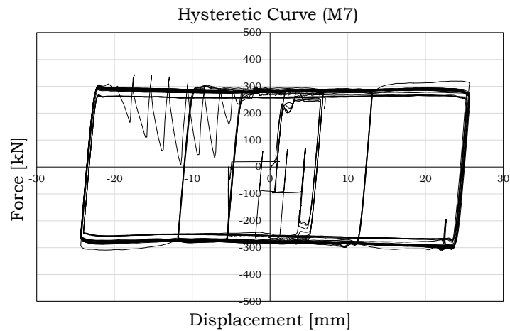
Fig. 2.16 – Hysteretic behaviour of hard materials: Carbide M7
