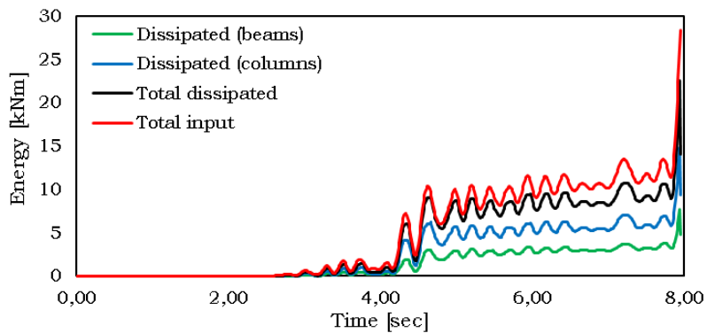
Fig. 5.203 – Overall dissipated energy - RBS 1
