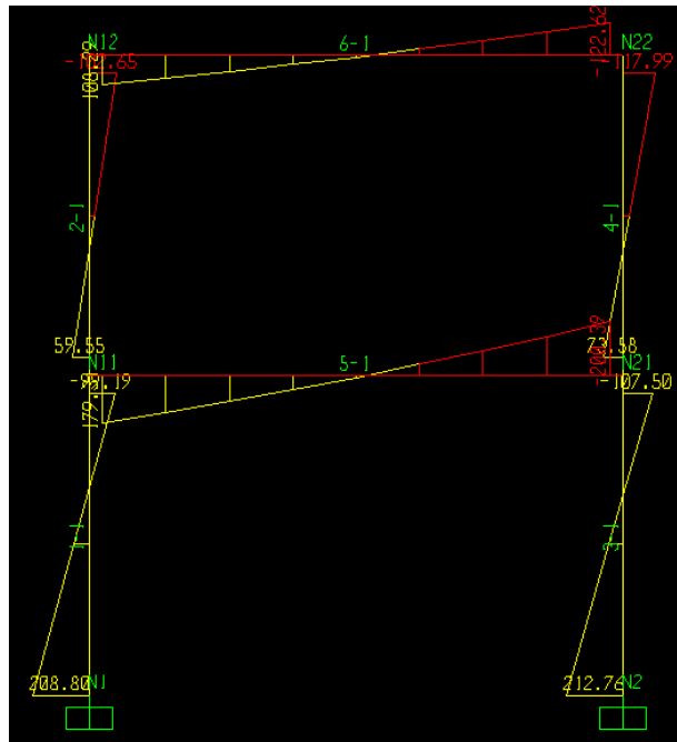
Fig. 5.25 – Bending moment for the check of the columns
