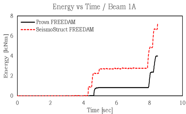
Fig.5.217 – Energy vs time – Bema 1A - FREEDAM
