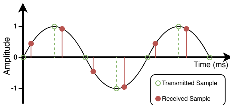
Figure 2.6: Representation on erroneous sampling due to clock offset between the transmitter and the receiver.
