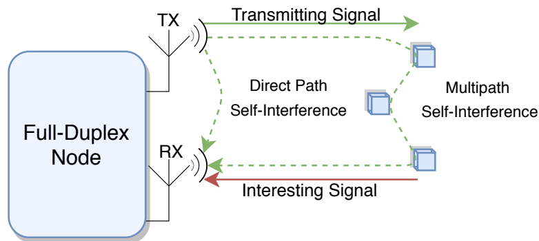
Figure 3.8: Self-Interference problem.
