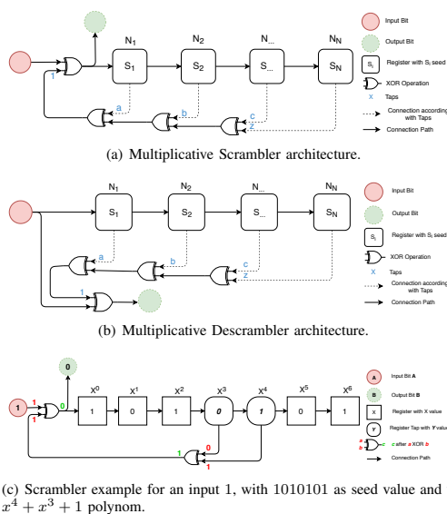
Fig. 8. Multiplicative scrambler architecture represented in 8(a) and its respective descrambler in 8(b)). A specific example is shown in 8(c)).
