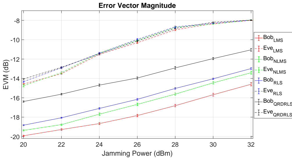
(a) EVM plot of adaptive algorithms.
