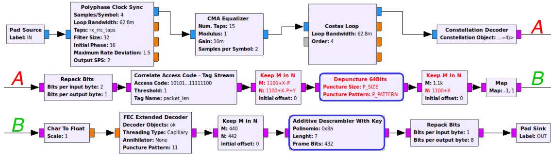
(b) Decoding hierarchical block used on reception in simulation.
