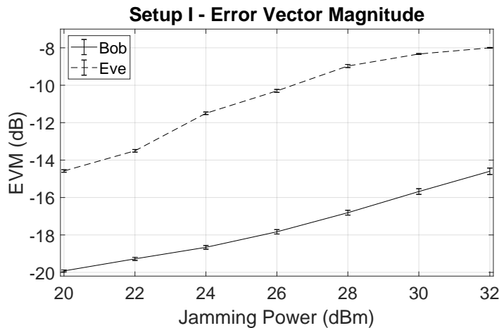
(a) EVM plot of setup I .
