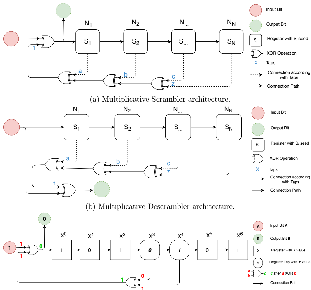
Figure 2.14: Multiplicative scrambler architecture represented in 2.14(a) and its respective descrambler in 2.14(b). A specific example is shown in 2.14(c).
