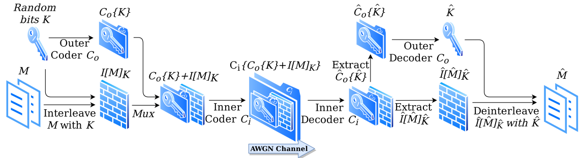
Figure 3.3: ICS security scheme architecture (figure adapted from [9]).
