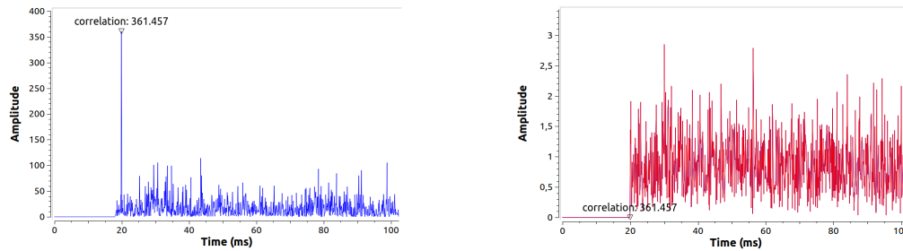
(a) Correlation values output from the Synchronization block. (b) Stream outputs of Synchronization block, where both streams are synchronized.
