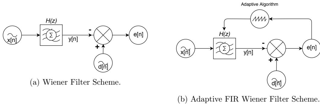
Figure 3.11: The Wiener Filter scheme is represented in 3.11(a), and the adaptive FIR Wiener Filter in 3.11(b). Figures adapted from [83] and [85].
