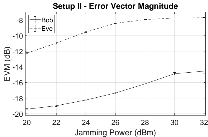
(a) EVM plot of setup II .
