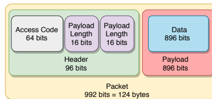
Fig. 5. Packet content and its length representation.
