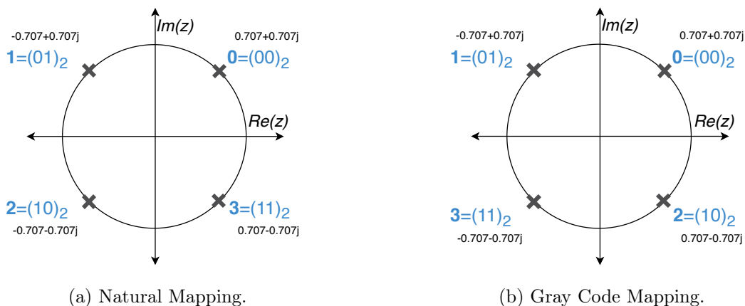
Figure 2.3: Difference between Natural Mapping 2.3(a) and Gray Code Mapping 2.3(b) on a QPSK constellation.
