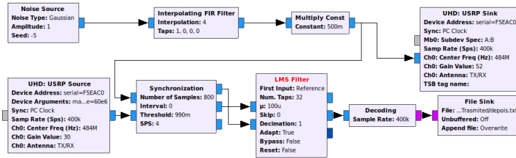
(d) Interference generation and its cancellation on the legitimate receiver.
