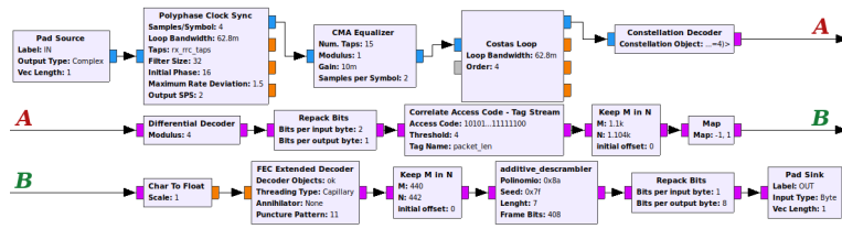
(b) "Decoding" block - Adapted SCS-HK receiver.
