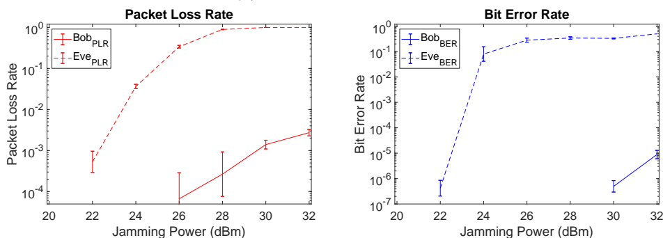
(b) PLR and BER plots of setup I .
