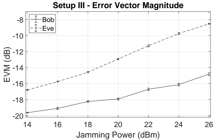
(a) EVM plot of setup III .
