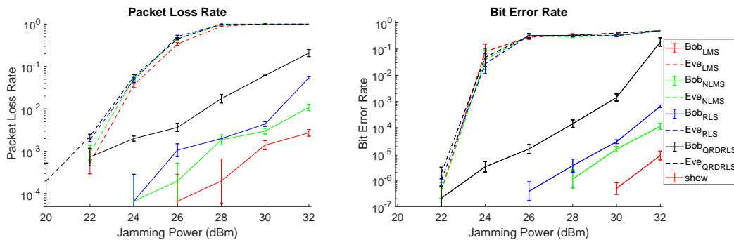
(b) PLR and BER plots of adaptive algorithms.
