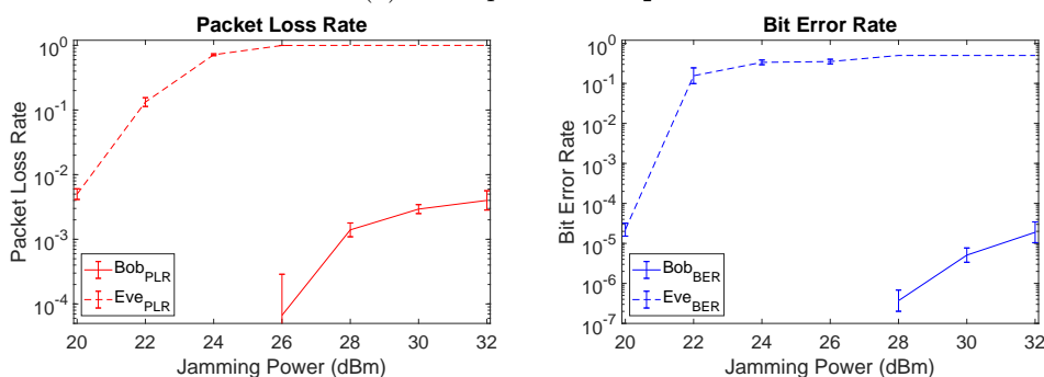
(b) PLR and BER plots of setup II .
