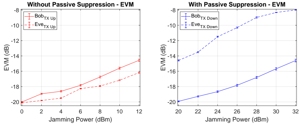
(a) EVM plot with and without passive suppression mechanism.
