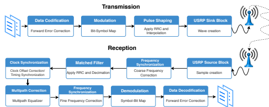
Fig. 1. General concepts of a wireless transceiver.
