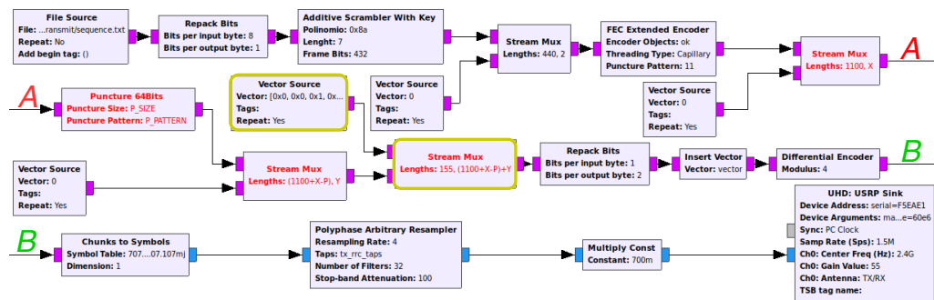
(a) Alice's side of the real-world prototype.
