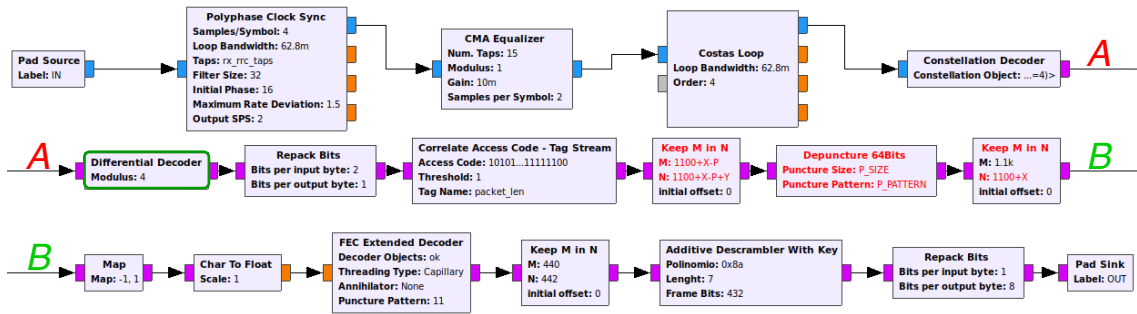
(b) Decoding hierarchical block used on reception.
