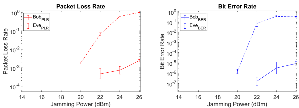
(b) PLR and BER plots of setup III .
