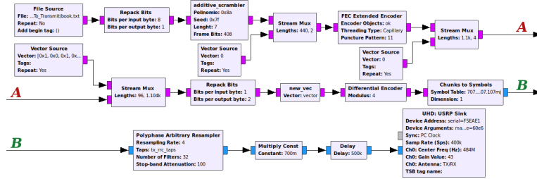
(a) Transmitter using the adapted SCS-HK.
