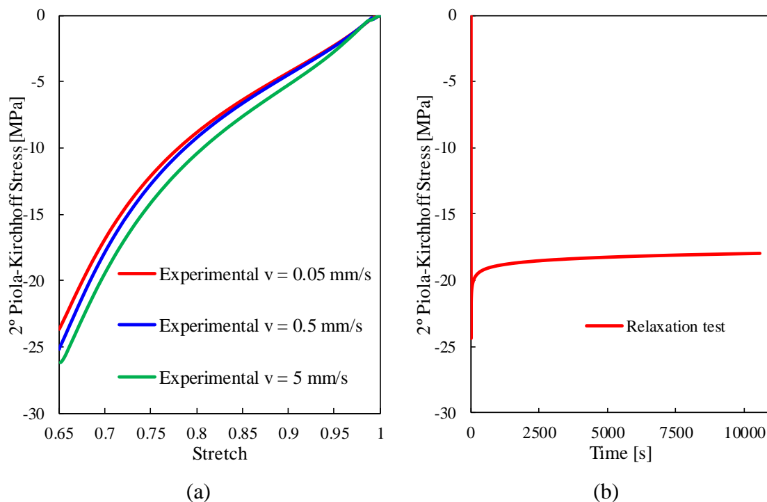
Figure 5.5. Experimental evolution of the second Piola Kirchhoff stress obtained from the orange PUR experimental tests: (a) uniaxial compression tests at different values of grip velocity and (b) relaxation test.
