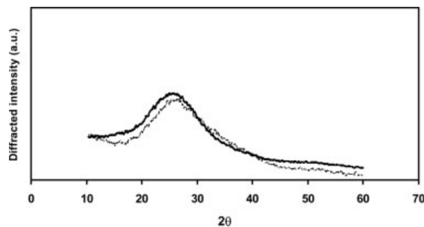
Figure 7. X-ray diffraction patterns of (—) C6PPD and (- - -) P8PPD.
