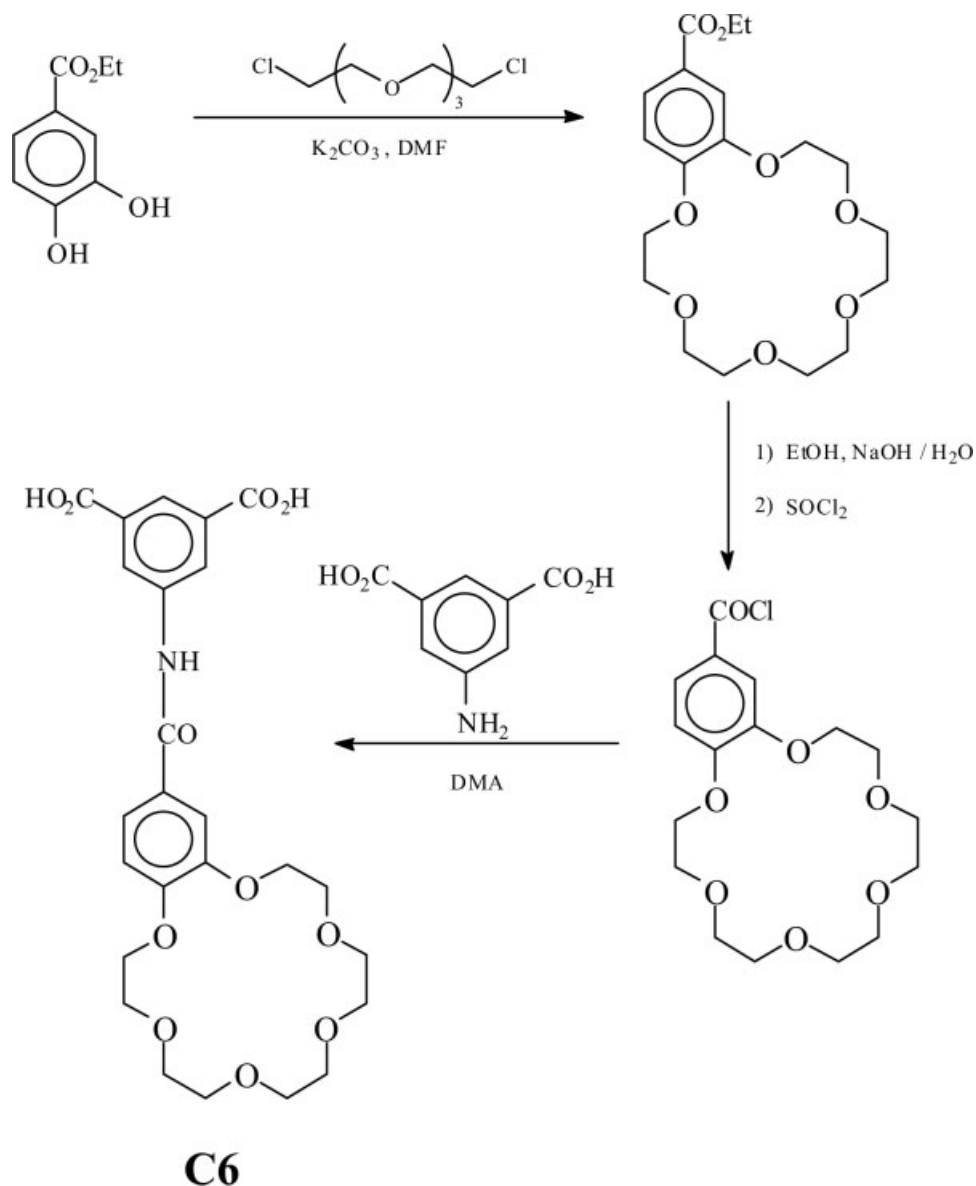
Scheme 1. Experimental sequences for the synthesis of 4-(3',5'-dicarboxyphenylamino)benzo-18-crown-6.
