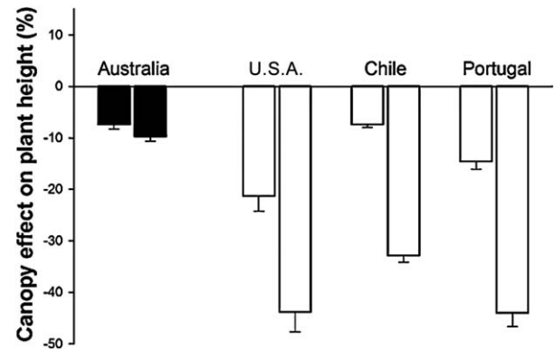
FIGURE 2 Variation in the effect of the Eucalyptus globulus canopy on understorey height between native (Australia) and non-native ranges (U.S.A., Portugal, Chile). Each bar indicates a site sampled in countries corresponding to the native (Australia) and non-native (U.S.A., Chile, Portugal) range of E. globulus . Values on the y axis are calculated as the difference between the mean plant height (cm; mean \pm 1 SE) of vegetation under E. globulus patches and in open areas, divided by the height in open areas for all pairs of plots at a given site
