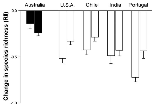
FIGURE 1 Relative interaction index (RII) values for species richness observed under the canopies of Eucalyptus globulus relative to open areas. Each bar indicates a site sampled in countries corresponding to the native (Australia) and non-native (U.S.A., Chile, Portugal, India) ranges of E. globulus . Error below means represent 1 SE
