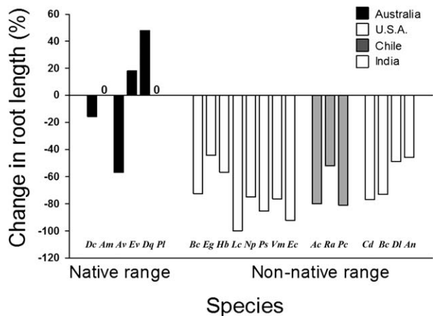
FIGURE 3 Effect of leachates on root length. Each bar represents a different species either native to the native range (Australia) or non-native range (U.S.A., Chile, India) of Eucalyptus globulus . The y axis shows the mean percentage decrease in root growth in leachates, relative to root growth in the controls for each species. Values correspond to the average amongst different Petri dishes used for each species in controls and treatments with leachates. Species corresponding to each bar are indicated below them (From left to right in the figure; Dc = Dichelachne crinita ; Am = Acacia melanoxylon ; Av = Acacia verticillata ; Ev = Eucalyptus viminalis ; Dq = Deyeuxia quadriseta ; Pl = Poa labillardieri ; Bc = Bromus carinatus ; Eg = Elymus glaucus ; Hb = Hordeum brachyantherum ; Lc = Lasthemia californica ; Np = Nasella pulchra ; Ps = Poa secunda ; Vm = Vulpia microstachys ; Ec = Escholzia californica ; Ac = Amsinckia calycina ; Ra = Rodophiala advena ; Pc = Pasithea coerulea ; Cd = Chloris dolichostachya ; Bc = Brassica campestris ; DI = Dalbergia latifolia ; An = Acacia nilotica )
