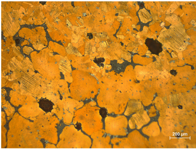
Fig. 10. OM micrograph from the cross-section of the sickles 81.07 showing a transition area between the dendritic structure (lower part of the image) and annealing twins and slip lines in some grains (upper part of the image) evidencing a selective application of thermomechanical treatments.
