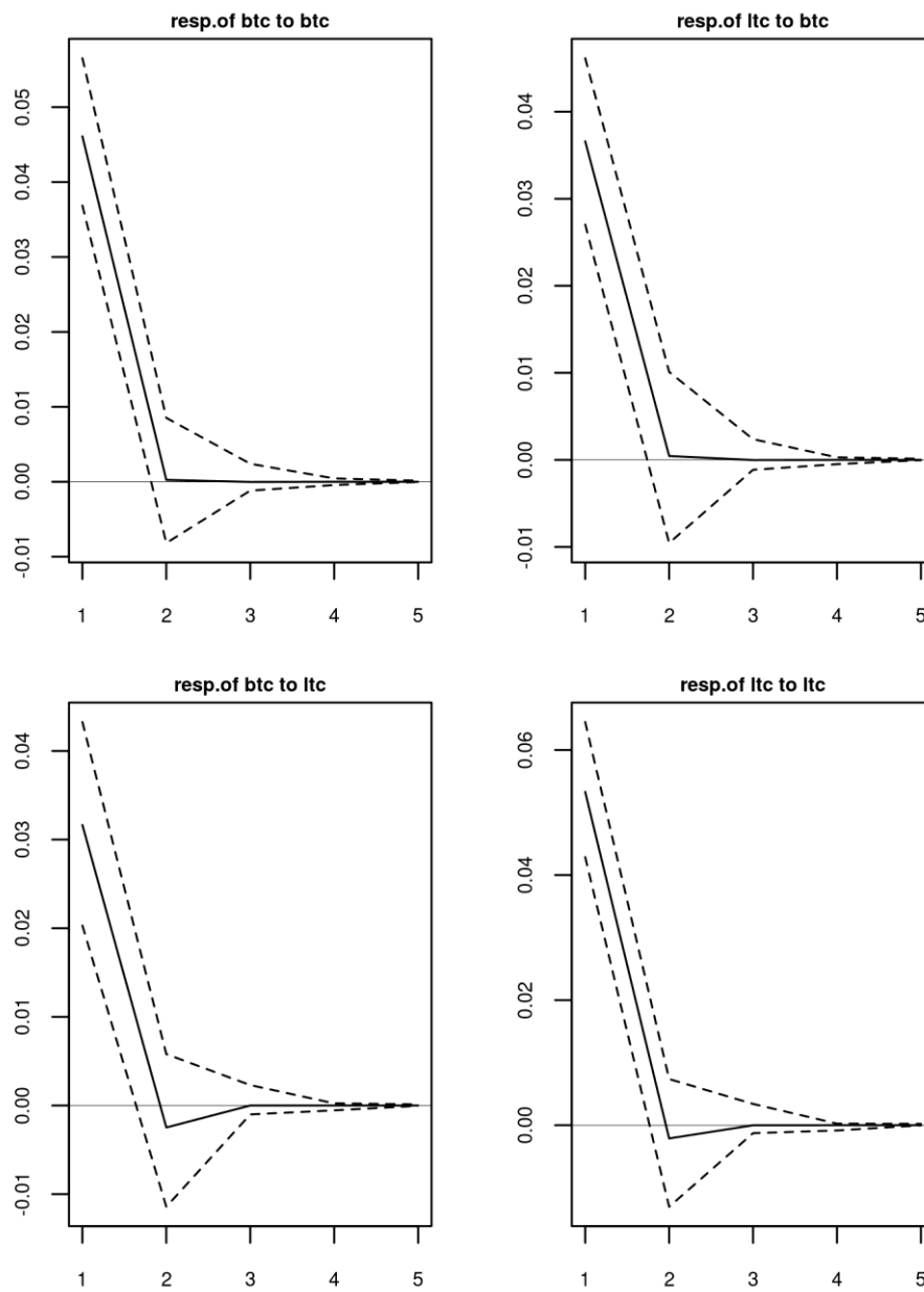
Figure no. 3 – Generalized impulse responses and 95% confidence interval - Segment S1 (May 2, 2013 – August 7, 2013).
