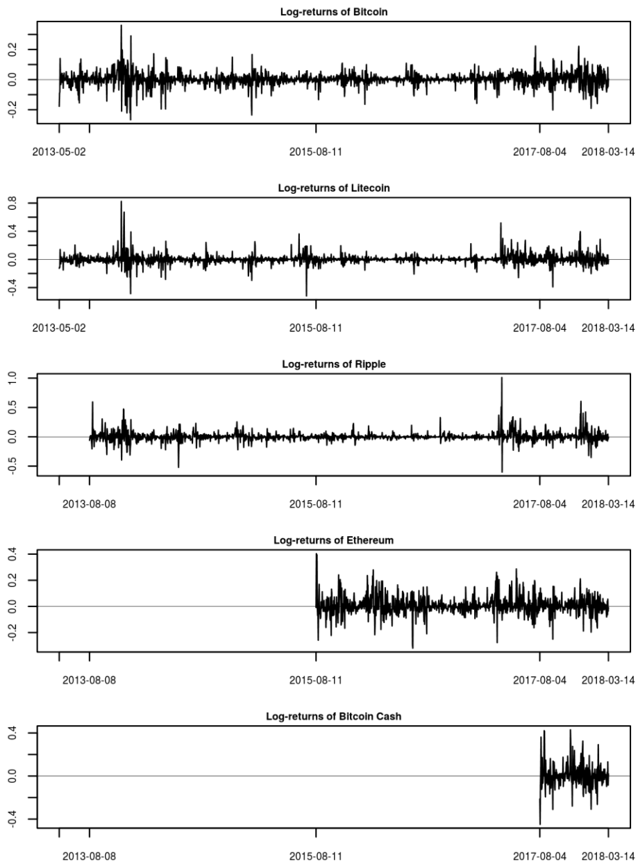
Figure no. 2 – Log-returns of bitcoin, litecoin, ripple, ethereum and bitcoin cash. Source: Coin Metrics ( https://coinmetrics.io/ , accessed March 19, 2018).
