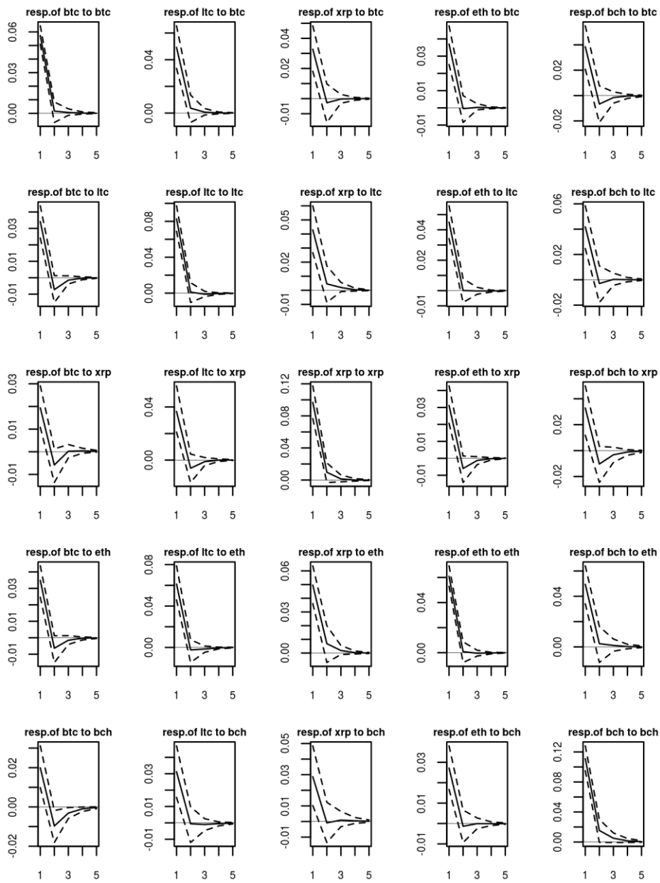
Figure no. 6 – Generalized impulse responses and 95% confidence interval - S4 (August 4, 2017 – March 14, 2018).
