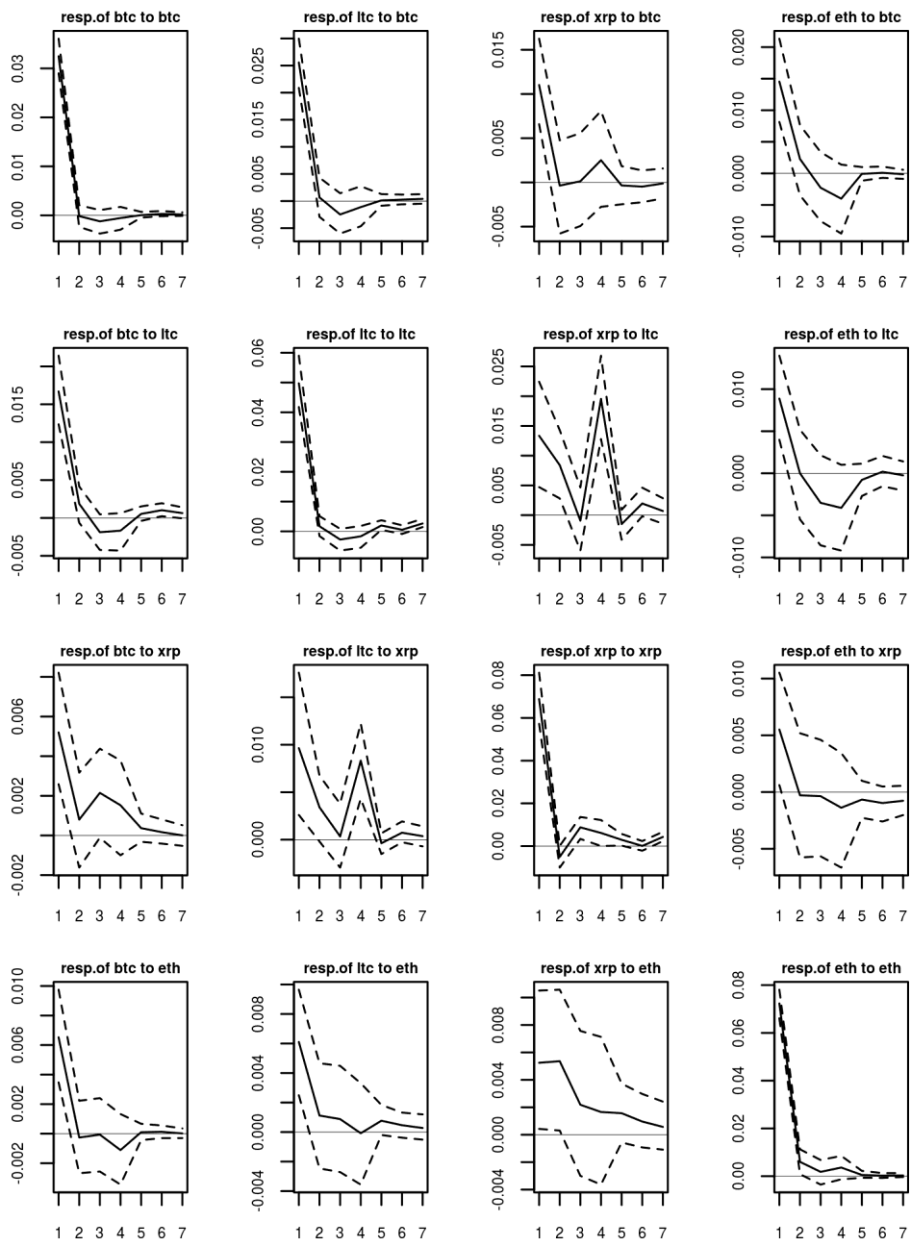
Figure no. 5 – Generalized impulse responses and 95% confidence interval - Segment S3 (August 11, 2015 – August 3, 2017).
