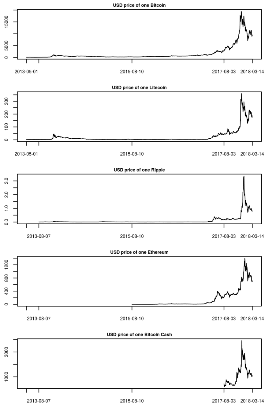
Figure no. 1 – Prices of bitcoin, litecoin, ripple, ethereum and bitcoin cash in USD. Source: CoinMetrics site ( https://coinmetrics.io/ , accessed March 19, 2018).
