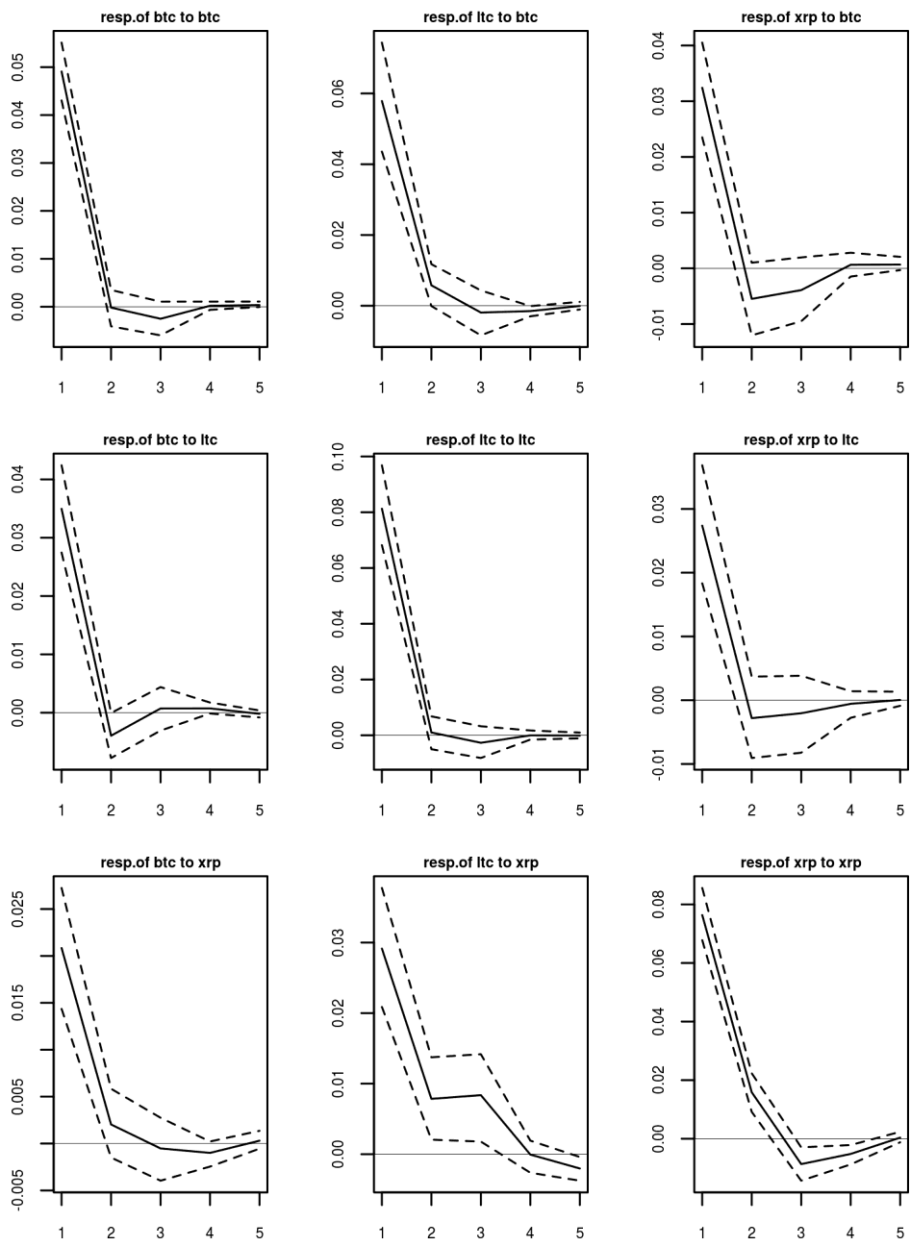
Figure no. 4 – Generalized impulse responses and 95% confidence interval - Segment S2 (August 8, 2013 – August 10, 2015).
