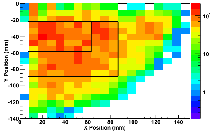
Figure 19. Map of the fired pixels in one of the Micromegas detectors installed in NEXT-MM (color of the pixel corresponds to the number of times it has been fired). The two regions selected to obtain the energy spectra after the analysis (of 10 \times 9 and 7 \times 5 pixels, respectively) are indicated.
