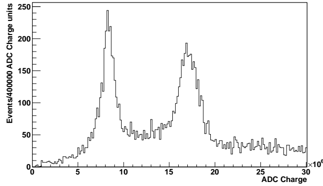
Figure 17. Raw spectrum (before applying any selection criteria) registered by one Micromegas in NEXT-MM where the peak of the ^{241}\text{Am} 59.5 keV gamma can be seen. The escape peaks corresponding to the characteristic X-rays of Xenon are also seen around 29 keV.
