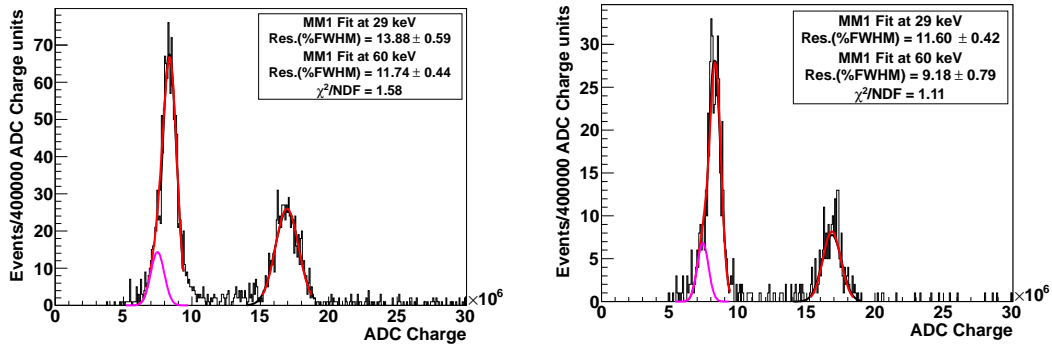
Figure 18. Energy spectra after the application of the selection criteria for two different areas of the Micromegas. Left: an area of 10 \times 9 pixels corresponding to \sim 32\% of the detector surface was selected. An energy resolution of 11.7% FWHM is obtained for the 59.5 keV peak. At \sim 29 keV the peak is a sum of the escape peaks from the characteristic X-rays of Xenon and the ^{241}\text{Am} gamma at 26.4 keV. Two gaussian fits are used and the energy resolution obtained for 29 keV is 13.9% FWHM. Right: when a more restricted region is studied ( 7 \times 5 pixels, i.e., 12% of the sector's surface), the obtained resolution is 11.6% and 9.9% FWHM for 29 and 59.5 keV respectively. This indicates that inter-pixel gain variations are important.
