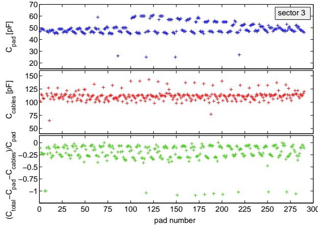
Figure 14. Measured capacitance with respect to ground for each separate pad (up). Measured capacitance for the cables up to the front-end electronics (middle). Difference between the measured and expected capacitance, normalized to the pad capacitance. When the connection to the pad is missing, a clear -1 is visible (down). The level of connectivity achieved for the sector in figure is above 95%.
