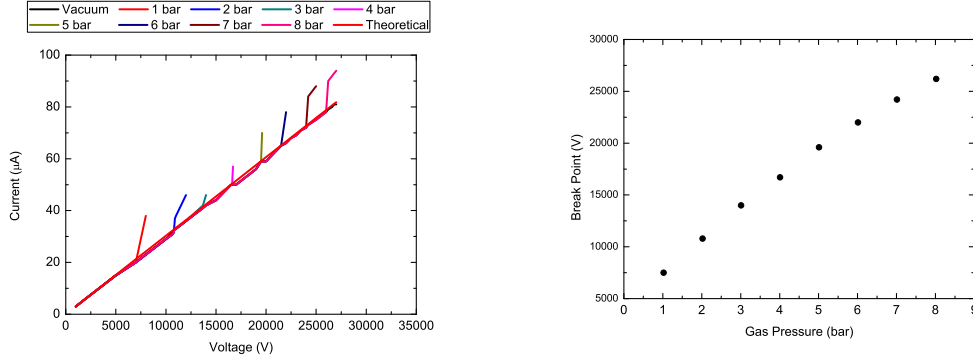
Figure 10. Current and breakdown point evolution depending on the system pressure.
