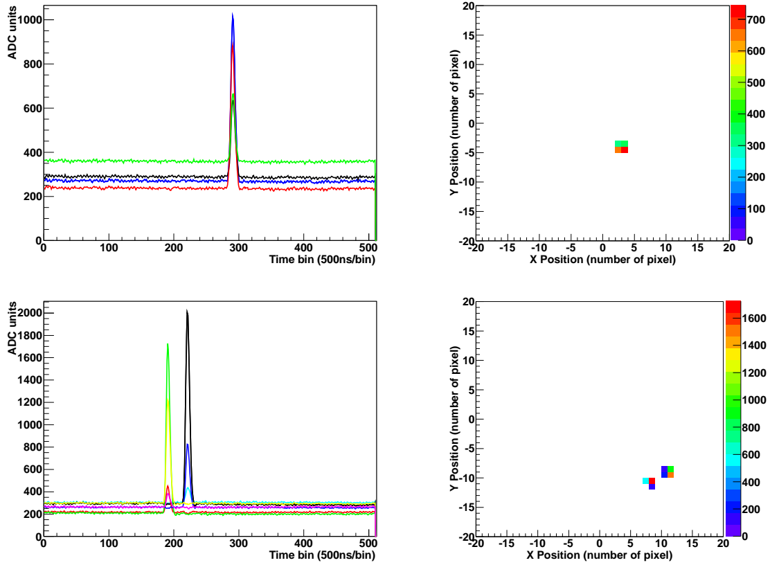
Figure 20. Examples of events attributed to the ^{241}\text{Am} source, in the upper part a 29 keV event, in the lower part a 59.5 keV event with two clusters (as result of the simultaneous detection of two 29 keV events or a connectivity problem of one of the pixels). Pulses in the activated pixels are shown on the left, while the 2D projections of the tracks in the XY plane, indicating (in ADC charge units) the total charge of the pixel with the color scale, are shown on the right.
