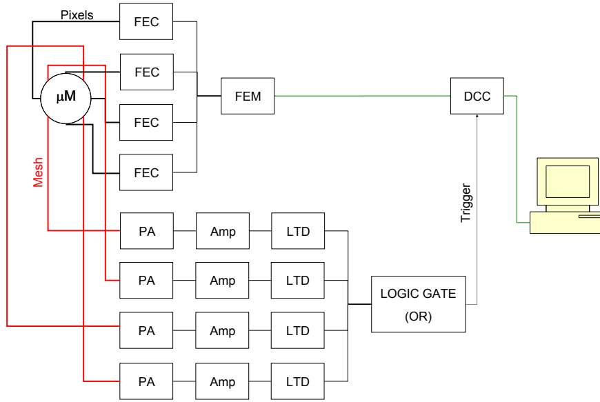
Figure 7. Conceptual sketch of the acquisition system of NEXT-MM adapted to four mesh signals as in the case of the Microbulk Micromegas. For the case of the Bulk detector, only one mesh signal has to be taken. If mesh signals have to be registered to obtain an energy spectrum, the amplified signals are processed by a Multi-Channel Analyzer (see text for components description).
