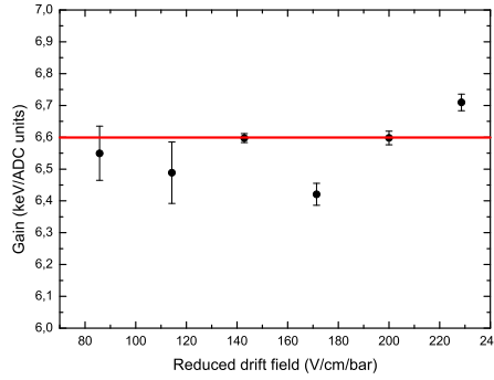
Figure 12. Evolution of the gain in terms of the applied drift voltage for a Bulk Micromegas operated at 1 bar of premixed Ar-(2%)iC 4 H 10 mixture. No significative variation of the gain is appreciated.
