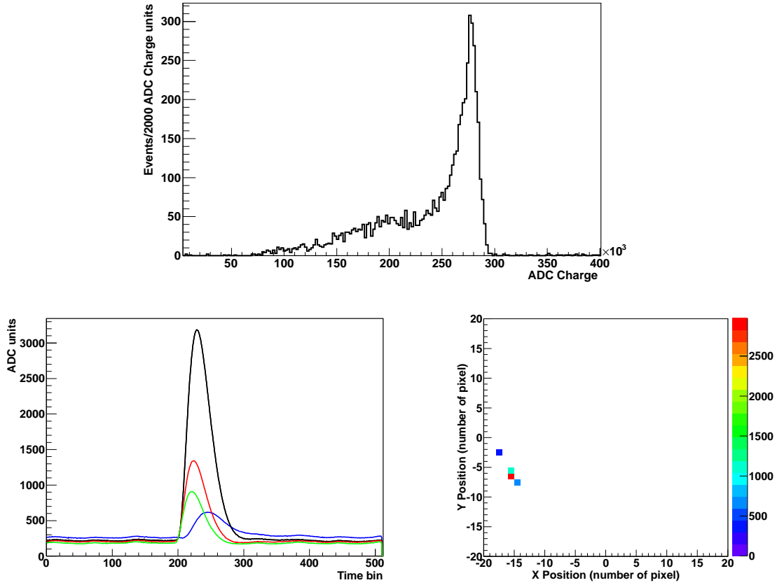
Figure 13. ^{241}\text{Am} energy spectrum obtained from the pixel signals of Microbulk Micromegas operated at 1 bar of a premixed Ar-(2%)iC 4 H 10 mixture (top) and example of a \sim 5.5 MeV event: pulses in the activated pixels (bottom left) and 2D projection of the track in the XY plane, indicating (in ADC charge units) the total charge of the pixel with the color scale (bottom right).
