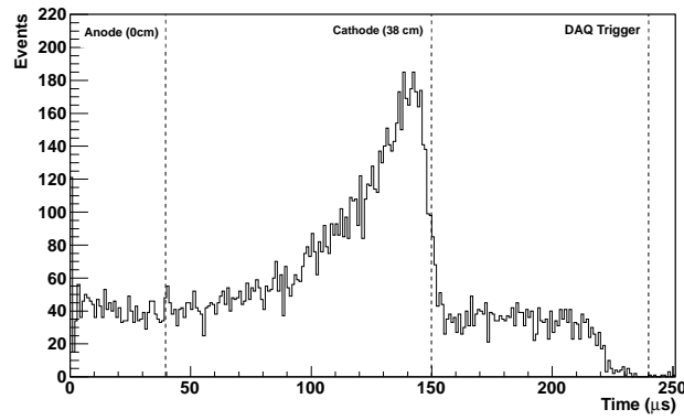
Figure 16. Time distribution of the events registered in one Micromegas. The anode plane starts at 40\ \mu\text{s} , according to the trigger delay, and the cathode extends up to 150\ \mu\text{s} , where the maximum of the distribution is situated.
