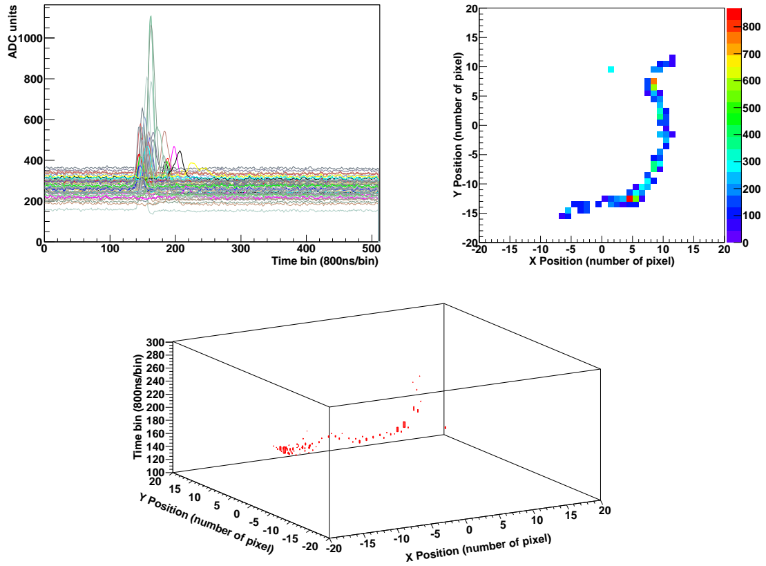
Figure 15. Example of background event: pulses in the activated pixels (left), 2D projection of the track in the XY plane, indicating (in ADC charge units) the total charge of the pixel with the color scale (right), and a 3D reconstruction of the event with a relative z position (bottom).
