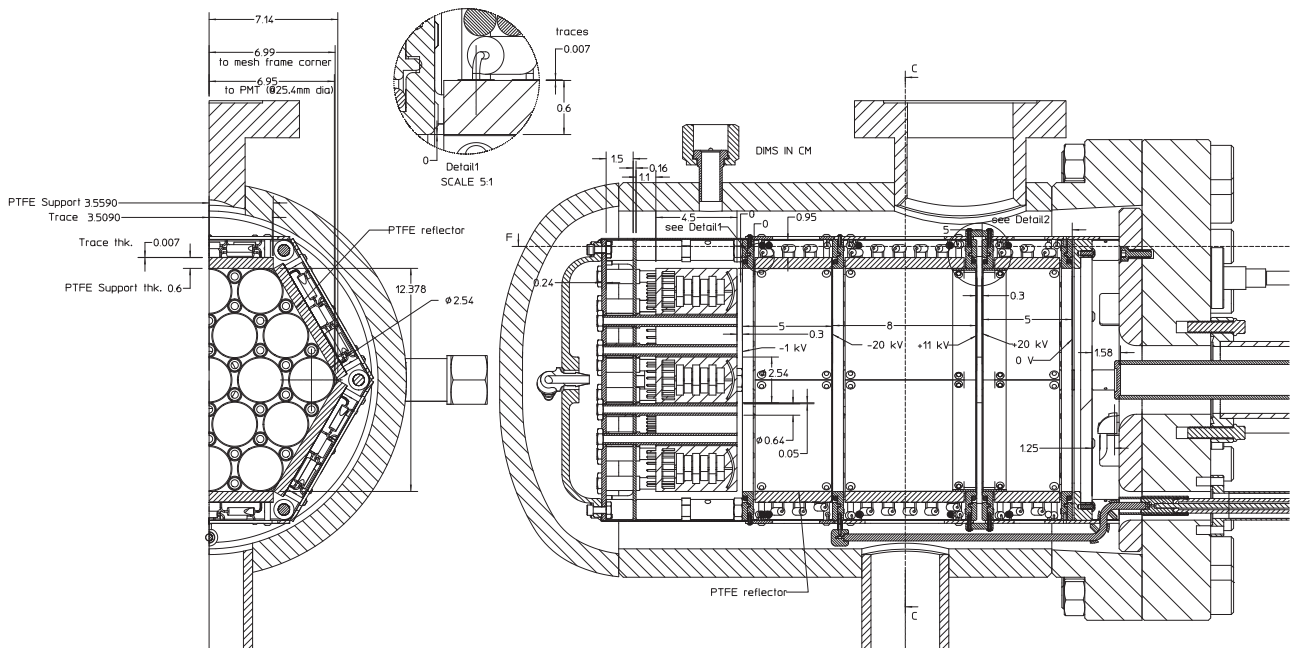
Fig. 3. Cutaway schematic of the TPC.
