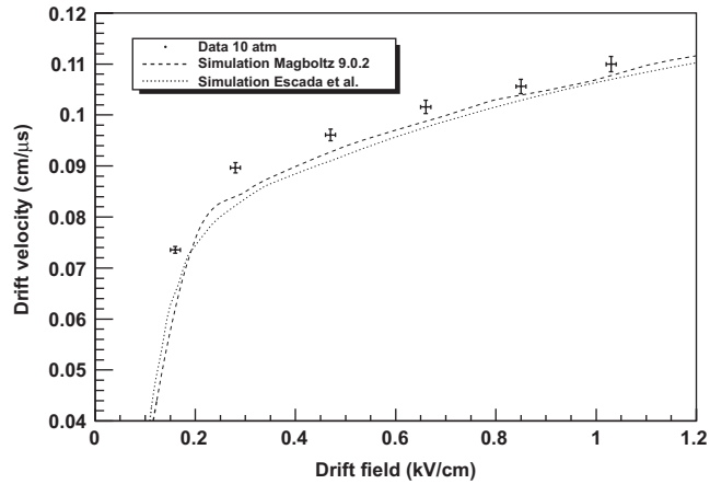
Fig. 20. Drift velocity dependence on drift field: The electron drift velocity obtained from the maximum drift times measured (which correspond to the full drift length of 8 cm) for X-ray energy depositions. These data were taken at 10.1 atm.
