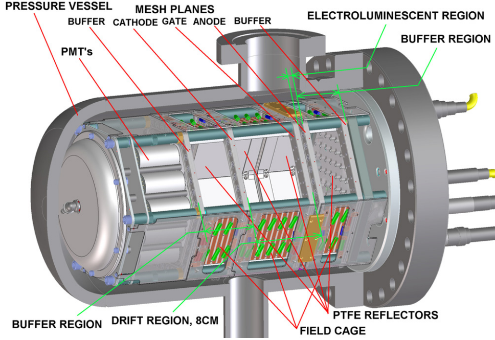
Fig. 1. NEXT-DBDM electroluminescent TPC configuration: An array of 19 photomultipliers (PMTs) measures S1 primary scintillation light from the 8 cm long drift region and S2 light produced in the 0.5 cm electroluminescence (EL) region 13.5 cm away from the PMTs. Two 5 cm long buffer regions behind the EL anode mesh and between the PMTs and the cathode mesh grade the high voltages (up to \pm 17 kV) down to ground potential.
