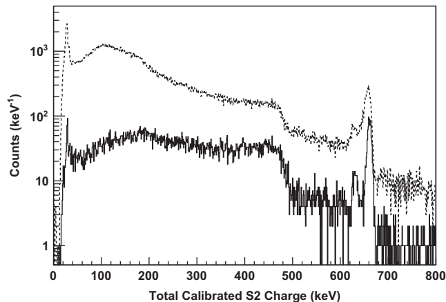
Fig. 8. Energy spectrum for ^{137}\text{Cs} 662 keV gamma rays: The dashed line shows the calibrated spectrum (using the full energy 662 keV peak alone) from a data run taken at 10 atm with a 0.3 kV/cm drift electric field and an E/P of 2 kV/(cm atm) in the EL region. The 1 mCi source is strongly collimated. Gamma rays enter the TPC along the drift axis ( z ). Below the full energy peak at 662 keV, the smaller X-ray escape peak at \sim 630 keV, the Compton edge at 477 keV and the xenon X-ray peak at \sim 30 keV can be seen. The solid line is the same spectrum with a requirement that the reconstructed average position of an event be less than \sim 1.2 cm from the TPC axis. The small feature near 184 keV is due to Compton backscatters. The no-source background spectrum (not shown) has a broad peak near 100 keV.
