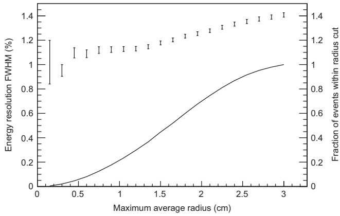
Fig. 11. Energy resolution dependence on radial cut: Full energy 662 keV events are chosen and, for each, an average x - y position is computed (and scaled to true TPC coordinates) using all of the S2 signal. The FWHM energy resolution (data points) is obtained from a gaussian fit to the peak after placing a cut on the radial position (the abscissa). The radial cut efficiency (solid line and right ordinate axis) is also shown. These data were taken at 10 atm with a 0.16 kV/cm field in the drift region and 2.1 kV/(cm atm) in the EL region.
