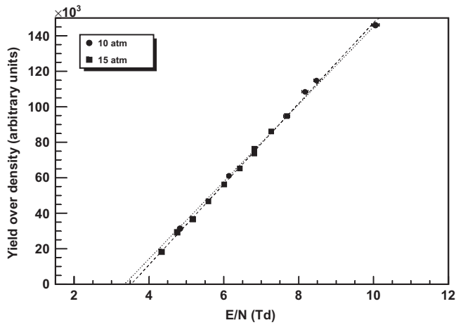
Fig. 19. Density normalized light yield vs. EL reduced field. The lines are the results of fits to a linear function for the 10 atm (dotted) and 15 atm (dashed) data points.
