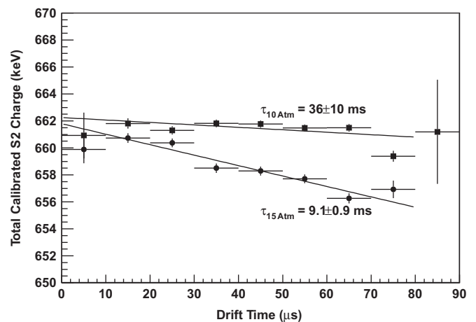
Fig. 9. Electron attachment losses: The average calibrated S2 charge versus the charge-weighted drift time is shown for full energy events. Attachment lifetimes are obtained from the exponential fits. The 10 atm data was taken with a 0.19 kV/cm field in the drift region and the 15 atm data with 0.59 kV/cm.
