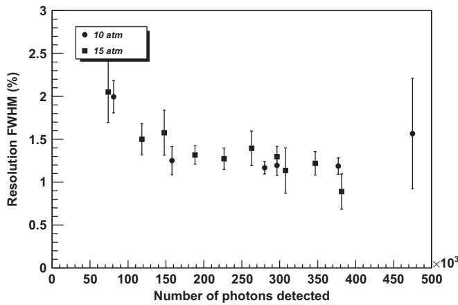
Fig. 12. Energy resolution dependence on amount of light detected: 662 keV full energy peak resolutions are shown for data runs with different total S2 light yield (controlled primarily by the E/P in the EL region). Energy spectra were obtained by selecting events reconstructed in the central 1 cm radius region and with an S1 signal with more than 100 measured photons and not more than 600. A small electron drift-time-dependent attachment correction is applied. These data were taken with drift fields of 0.5–0.6 kV/cm at 10 atm and 0.16–0.72 kV/cm at 15 atm.
