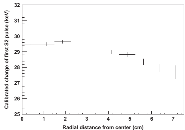
Fig. 10. Radial dependence of energy response: Xenon X-ray energy depositions were selected from full-energy 662 keV events for which the first S2 pulse has energy in the 20–40 keV range. The reduced response at larger radial positions (also observed in a detailed Monte Carlo simulation of the TPC) is due to geometric and optical effects of the EL light collection efficiency. These data were taken at 10 atm with a 1.0 kV/cm field in the drift region and 2.68 kV/(cm atm) in the EL region.
