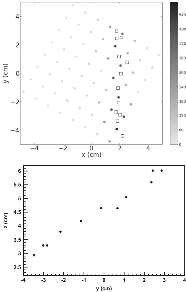
Fig. 23. Cosmic ray muon track measured in the 8 \times 8 SiPM array near the EL region: Top: The 64 SiPMs covering an 8 cm by 8 cm area in the center of the TPC are shown as circles shaded relatively according to the total amount of light observed by each. The x - y coordinates at each point in the reconstructed track are given by the squares. Bottom: The z coordinate is calculated from the time delay between the SiPM signals and the event S1 with the known drift velocity.
