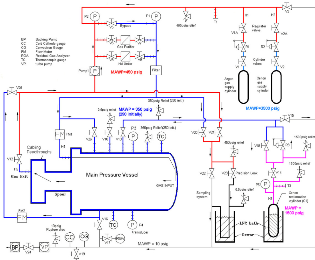
Fig. 2. Gas system schematic (simplified): The bottom left of the diagram shows the main pressure vessel with its connections to the vacuum, fill, recirculation/purification, sampling and reclamation components.
