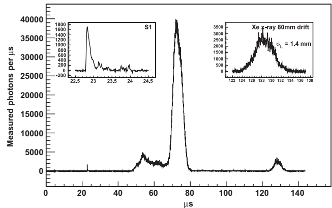
Fig. 4. Typical full energy 662 keV gamma ray event waveform: the sum of the previously calibrated waveforms of the 19 photomultipliers is shown. The S1 pulse (shown in detail in the left inset) due to xenon scintillation is short and with O(200) measured photons. Two S2 pulses caused by electroluminescence of xenon from ionization electrons follow. The first with \sim 270,000 measured photons is likely due to a 630 keV electron from the photoelectric interaction of the 662 keV gamma ray; the pulse structure reflects the ionization density of the track along its \sim 2.5 cm long projection on the drift ( z ) direction. The second (shown in detail in the right inset) with \sim 12,000 measured photons is likely due to the interaction, a few cm away, of a 30 keV xenon X-ray following the photoelectric process; since the 30 keV energy deposition is nearly point-like the pulse shape is gaussian with a \sigma_L of 1.4 mm set by the longitudinal diffusion of the electrons during the \sim 8 cm drift. This event is from a data run taken at 10 atm with a 0.16 kV/cm drift electric field and an E/P of 2.1 kV/(cm atm) in the EL region.
