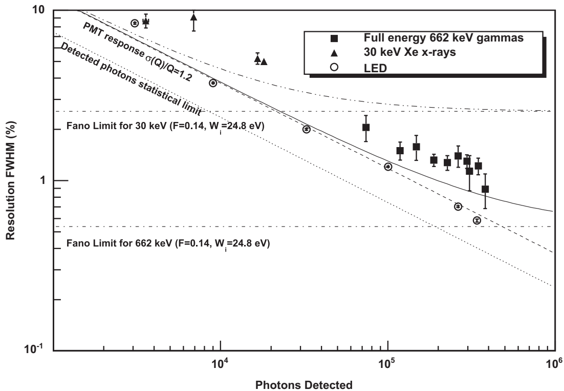
Fig. 16. Energy resolution in the high-pressure xenon NEXT-DBDM electroluminescent TPC: Data points show the measured energy resolution for 662 keV gammas (squares), ~30 keV xenon X-rays (triangles) and LED light pulses (circles) as a function of the number of photons detected. The expected resolution including the intrinsic Fano factor, the statistical fluctuations in the number of detected photons and the PMT charge measurement variance is shown for X-rays (dot dot dashed) and for 662 keV gammas (dot dot dot dashed). Resolutions for the 662 keV peak were obtained from 15.1 atm data runs while X-ray resolutions we obtained from 10.1 atm runs.
