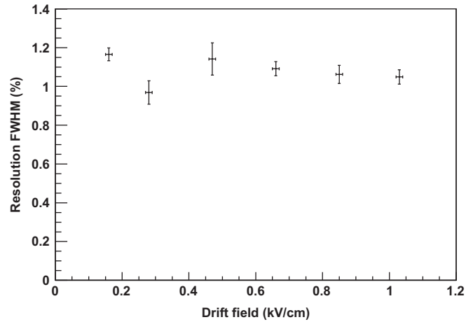
Fig. 17. Energy resolution dependence on drift field: These data were taken at 10.1 atm with 2.1–2.7 kV/(cm atm) in the EL region. The energy resolution attained is largely independent of the drift electric field in the investigated range.
