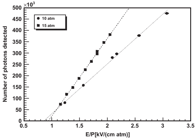
Fig. 18. Light yield dependence as a function of E/P in the EL region.
