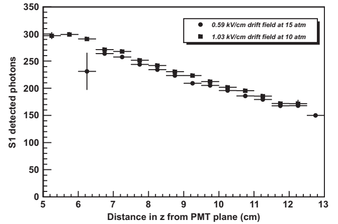
Fig. 22. S1 signal dependence on z position: For events with full energy 662 keV depositions, the number of measured S1 photons is shown versus the average distance of the ionization track from the PMT plane (obtained from the S2 charge-weighted drift time and the measured drift velocity). Two runs are shown with E/P in the drift region of 0.04 and 0.10 kV/(cm atm) with very similar S1 yield.
