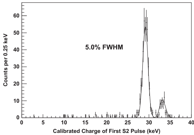
Fig. 15. Energy resolution at 10 atm for 30 keV xenon X-rays: A 5% FWHM energy resolution for 30 keV was obtained. These data were taken at 10.1 atm with a 1.03 kV/cm field in the drift region and 2.68 kV/(cm atm) in the EL region.
