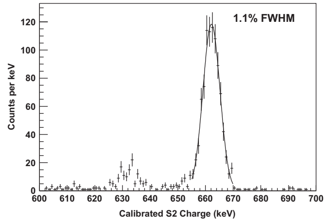
Fig. 13. Energy resolution at 10 atm for 662 keV gamma rays: These data were taken at 10.1 atm with a 0.16 kV/cm field in the drift region and 2.08 kV/(cm atm) in the EL region. If assumed to follow a 1/\sqrt{N} dependence this resolution extrapolates to 0.57% at Q_{\beta\beta} = 2.459 MeV.
