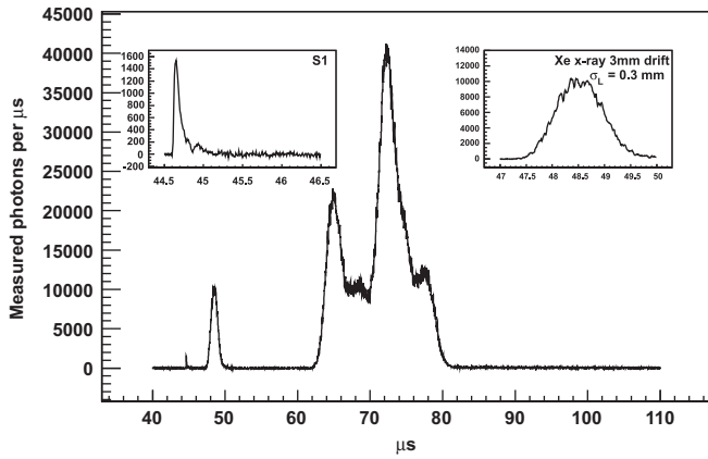
Fig. 5. A second typical full energy event: In this event from the same data run as in Fig. 4 the xenon X-ray interacted close to the EL region. The ionization electrons from it drifted for just 3 mm and underwent a correspondingly small longitudinal diffusion \sigma_L of 0.3 mm.
