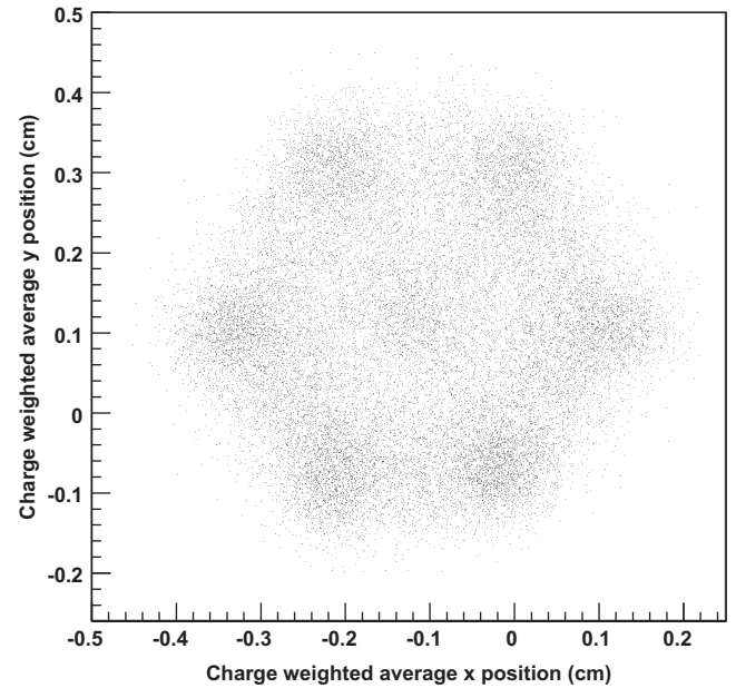
Fig. 6. Position reconstruction: The charge-weighted average of the 19 PMT positions is used for x - y reconstruction. Events with energy depositions between 50 and 100 keV were selected; at these energies ionization tracks extend for just a few mm. The edges of the hexagonal area correspond to the TPC cross-section. Due to the spatial uniformity of the PMT plane illumination a scaling factor of \sim 30 (not applied here) is needed to obtain true x - y positions from these charge-weighted averages. These data were taken with the ^{137}\text{Cs} source, at 10 atm and with E/P of 2 kV/(cm atm) in the EL region.
