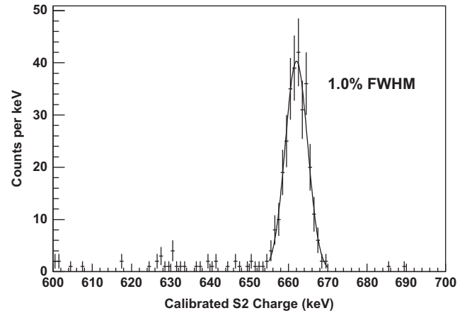
Fig. 14. Energy resolution at 15 atm for 662 keV gamma rays: A 1.0% FWHM energy resolution was obtained for events reconstructed in the central 0.75 cm radius region. The attachment losses correction with \tau = 9.0 ms was applied. A PMT with a clear time varying response was removed from the measurement. These data were taken at 15.1 atm with a 0.59 kV/cm field in the drift region and 1.87 kV/(cm atm) in the EL region.
