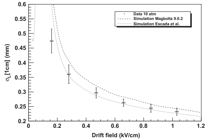
Fig. 21. Longitudinal diffusion dependence on drift field: The measured longitudinal diffusion is presented here as the \sigma spread along the drift direction for a 1 cm drift. These data were taken at 10.1 atm.
