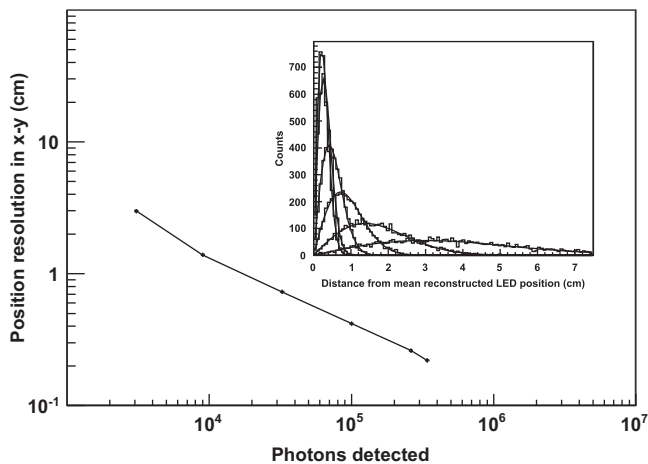
Fig. 7. Position resolution for LED light pulses: The position resolution in the x - y plane as a function of the number of detected photons is shown. The inset shows the radial distributions (and fits) from which the individual resolution values were obtained.
