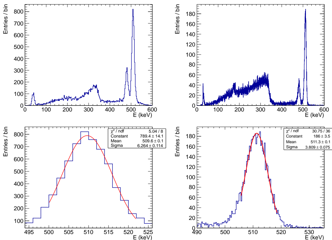
Figure 20. Top: Energy spectra for ^{22}\text{Na} gamma-ray events within the fiducial volume of NEXT-DEMO after spatial corrections. Left for the ultraviolet configuration (UVC); right for the blue configuration (BC). Bottom: Gaussian fits to the photoelectric peaks of the above energy spectra, indicating an energy resolution at 511 keV of 2.89% FWHM for the UVC and 1.75% FWHM for the BC.
