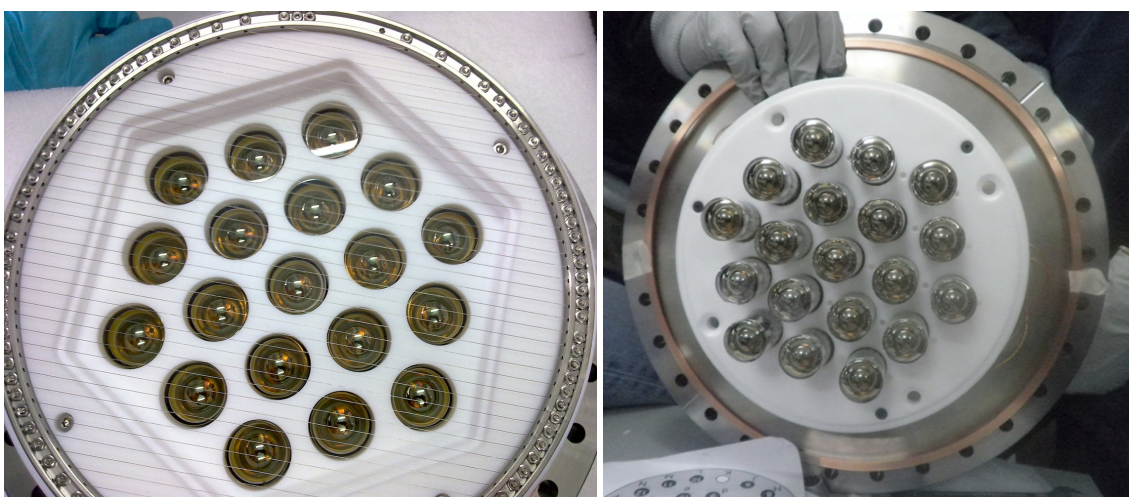
Figure 9. The energy (left) and tracking (right) planes of NEXT-DEMO, each one equipped with 19 Hamamatsu R7378A PMTs.
