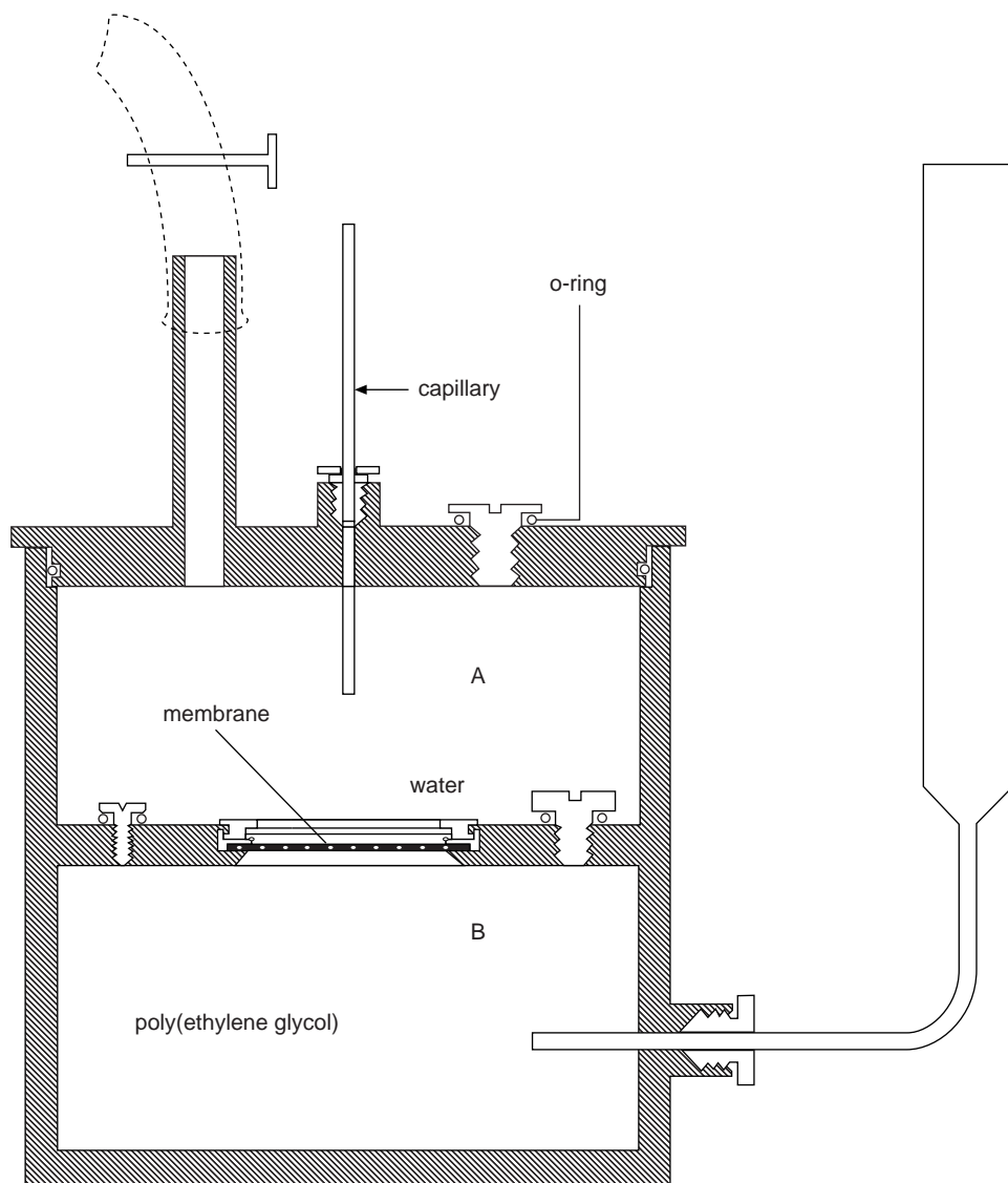
FIGURE I. Diffusion cell.
