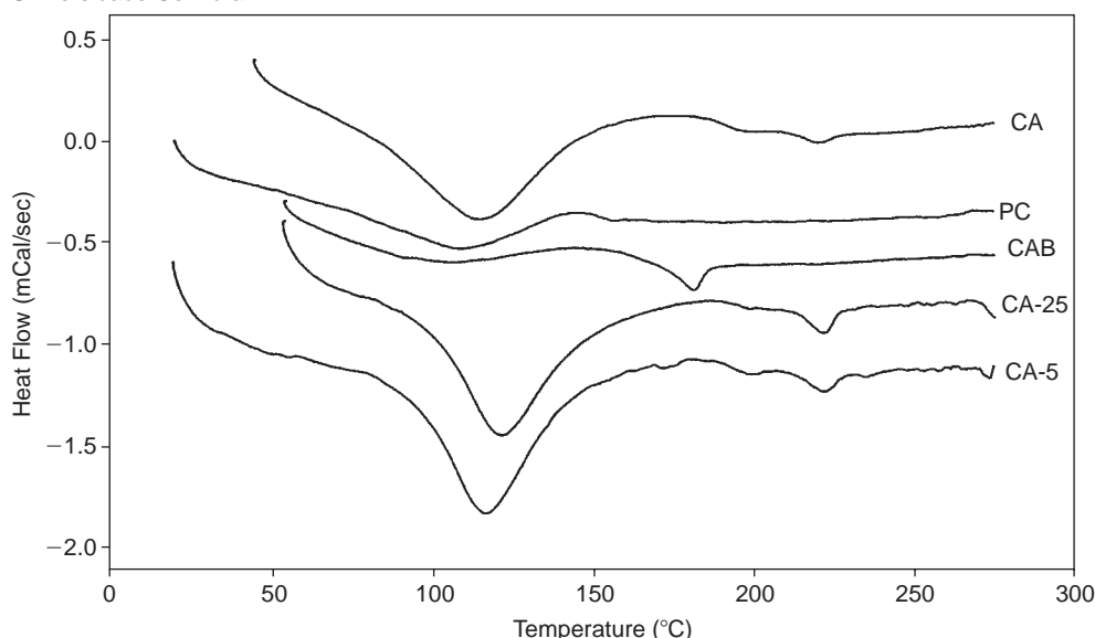
FIGURE 2. DSC profiles of the cellulose ester membrane systems CA-cellulose acetate , CP-cellulose propionate , CAB-cellulose acetate-butyrate , CA-25-cellulose acetate (25 °C - see text) , CA-5-cellulose acetate (5 °C - see text) .
