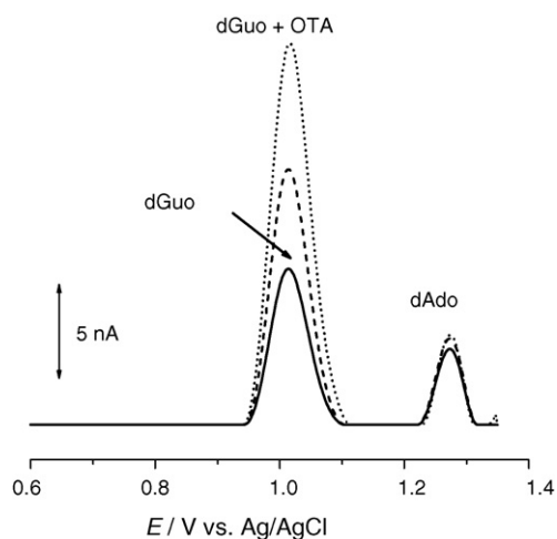
Fig. 7. DP voltammograms obtained in pH 4.5 0.1 M acetate buffer with dsDNA biosensors (—) before and after incubation during (---) 5 and (●●●) 10 min in a solution of 100 \mu\text{M} OTA. Pulse amplitude 50 mV, pulse width 70 ms and scan rate \nu = 5 \text{ mV s}^{-1} .
