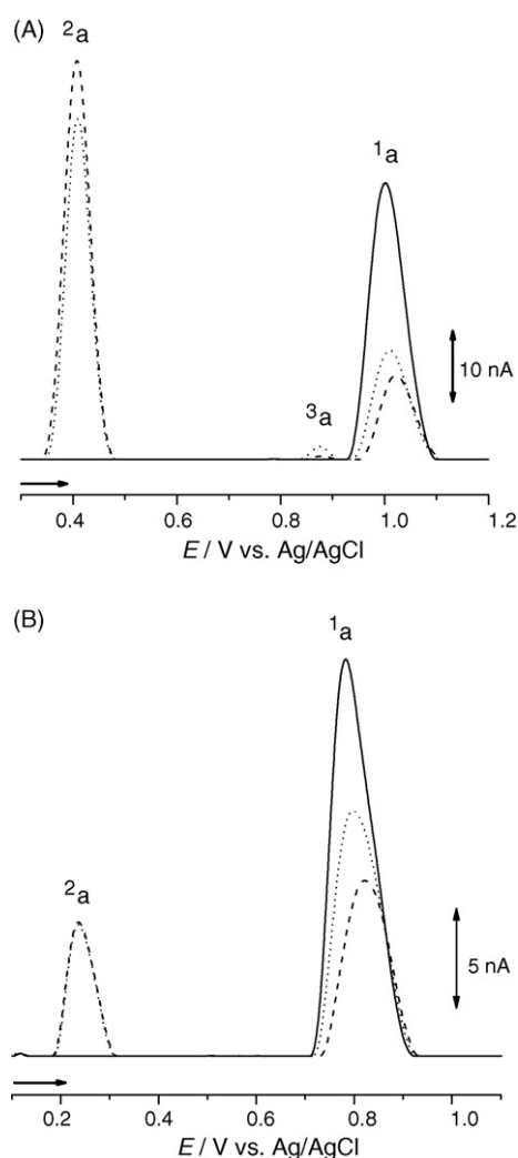
Fig. 3. Base line corrected DPV recorded in 5 \mu\text{M} OTA in: (A) pH 4 0.2 M acetate buffer and (B) pH 7 0.2 M phosphate buffer; (—) first and (●●●) second and (■) third scan; Pulse amplitude 50 mV, pulse width 70 ms and scan rate \nu = 5 \text{ mV s}^{-1} .
