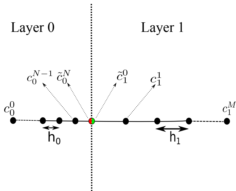
Figure 4: Schematic illustration of grid nodes in the first two layers and the interface points (in red and green). They are computed a posteriori as a linear combination of the neighbouring grid points (eqns. (6.4)–(6.5)). At the other interfaces a single concentration value occurs.
