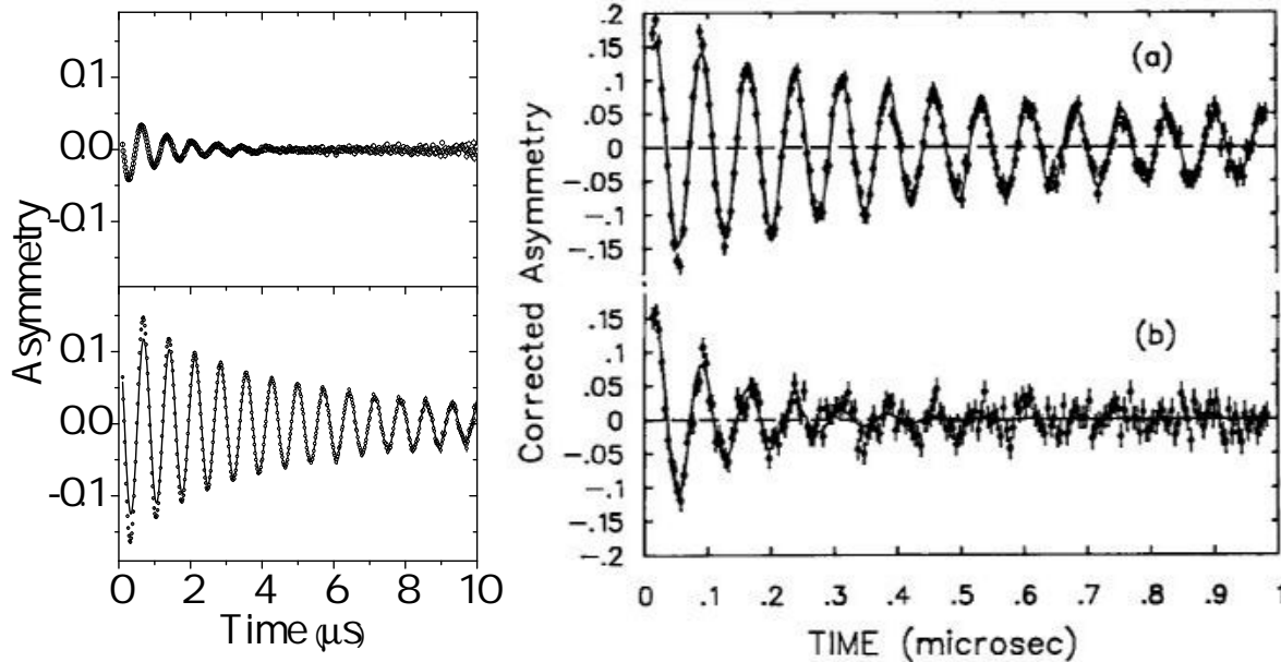
FIG. 1: Left: \mu SR signal of slightly Mg-doped zirconia \text{ZrO}_2\text{:Mg} at 8 K (data from Ref. 6). The signal (full data in the lower frame) is decomposed in a slowly relaxing component (solid line in the lower frame) and a fast relaxing component (upper part of the figure). Right: \mu SR spectra of \text{Al}_2\text{O}_3 at (a) 8(2) K and (b) 16(3) K (figure from Ref. 7, copied with permission). The solid lines are fit curves with a single exponential function but with different relaxations. The precession frequencies in all cases are close to the Larmor frequency of diamagnetic muon.
