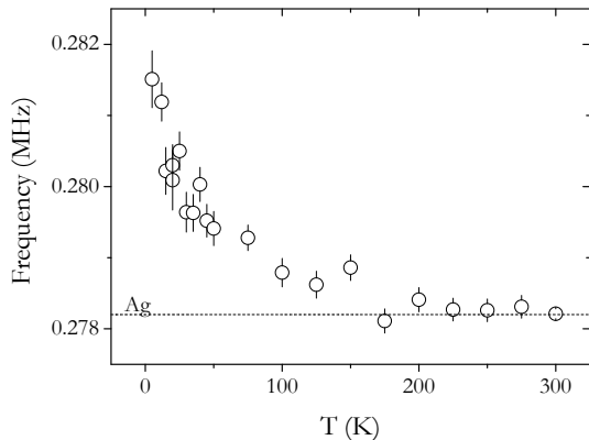
FIG. 5: \mu SR frequency of \text{ZrO}_2\text{:Mg} at B = 2 mT as function of temperature. The expected frequency from the calibration with an Ag sample is shown for comparison.
