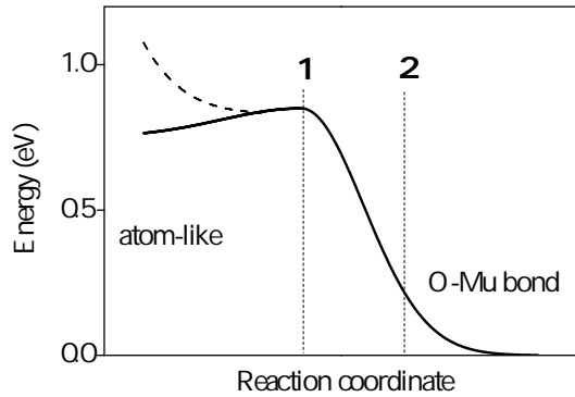
FIG. 6: Schematic representation of the total energy for the conversion from atom-like interstitial to anion-bound muonium (adapted from Ref. 26). The dashed line indicates the potential during the first steps of the lattice relaxation. The vertical lines (marked 1 and 2) indicate branching points (see text).
