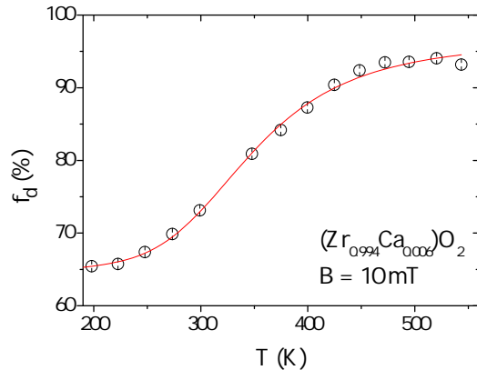
FIG. 7: Recovery of the diamagnetic fraction as a function of temperature for \text{ZrO}_2:\text{Ca} (from Ref. 6).
