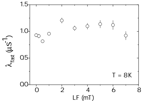
FIG. 4: Longitudinal-field relaxation rate of the fast relaxing signal in \text{ZrO}_2\text{:Mg} at 8 K.
