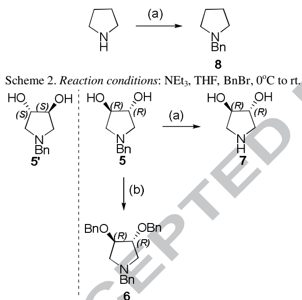
Scheme 3. Reaction Conditions: (a) Pd(0)EnCat, EtOH, H 2 ; (b) NaH, DMF, BnBr.
