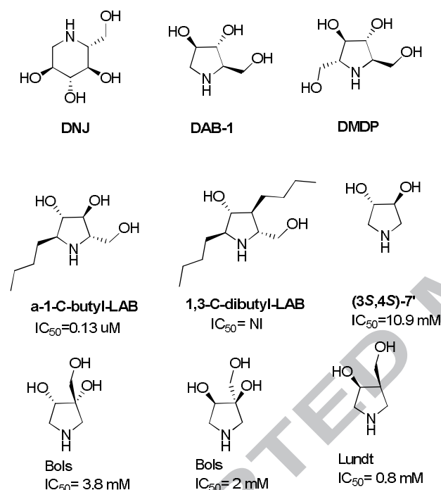
Figure 1. Examples of natural and synthetic iminosugars.
