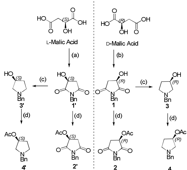
Scheme 1. Reaction conditions: (a)(i) BnNH 2 , MeOH/H 2 O, 170°C; (ii) 160°C (b) BnNH 2 , Xylene, 170°C (c) LiAlH 4 , THF, NaOH (20%) (d) py, Ac 2 O, rt
