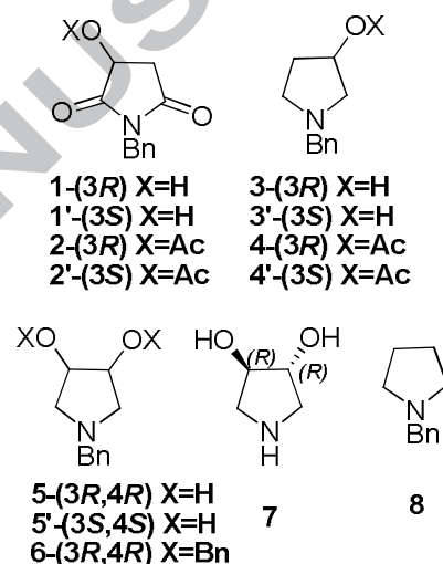
Figure 2. Library of 5-membered iminosugars synthesized and test.
