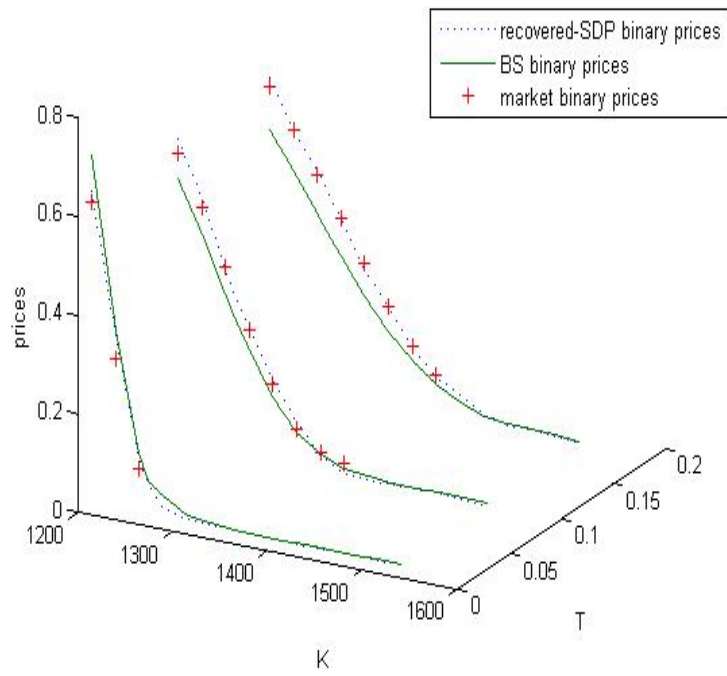
Figure 13: Recovered binary call prices from S&P500 data using the SDP approach against Black-Scholes binary prices and S&P500 2008 binary prices.
