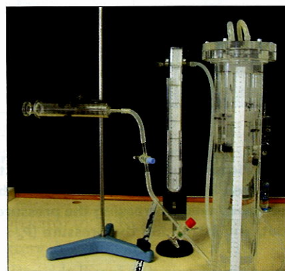
Fig. 1. The Cartesian diver is an inverted test tube with an air bubble trapped inside. The tube is placed in a closed 1-m long acrylic cylinder containing water. The pressure on the liquid surface in the cylinder is controlled with a syringe (on the left) and measured with a manometer (in the center).
