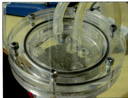
Fig. 2. The top of the cylinder with a removable lid tightly fixed with screws and an O-ring to ensure good closure.
