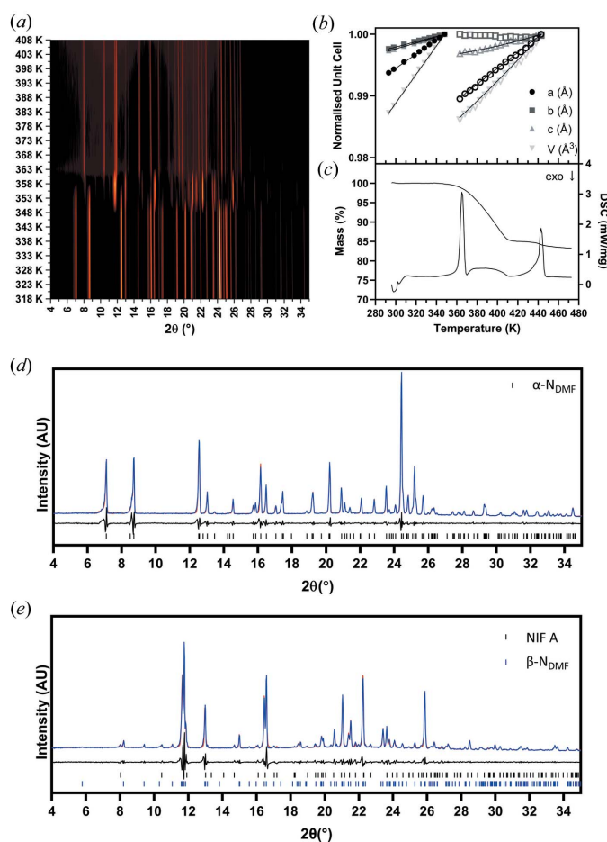
Figure 4 Thermal data of N_{\text{DMF}} capturing the desolvation to \alpha -NIF. (a) Surface plot of VT-XRPD data from 318 K to 408 K. (b) Unit-cell parameters from Rietveld refinements of each XRPD pattern. Closed symbols represent data for the solvate; open symbols represent data for desolvated structure. The data were fitted with the Berman equation of state (Angel et al. , 2014; Gonzalez-Platas et al. , 2016; Berman, 1988). (c) DSC and TGA traces for N_{\text{DMF}} . (d) XRPD pattern for the DMF solvate collected at 293 K [the model (blue) is superimposable on the data (red) indicating a good fit]. (e) XRPD pattern obtained at 358 K (after phase change). The pattern is well accounted for by indexed phase ( \beta - N_{\text{DMF}} ) and minor component of NIF A. For both fitted patterns [(d) and (e)], the experimental data are shown in blue, whilst the calculated profile is shown in red. The difference profile is displayed underneath the diffraction pattern.
