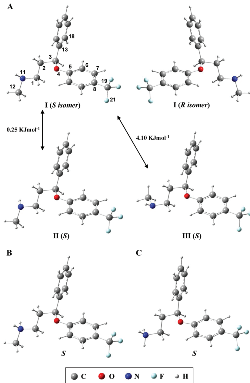
Figure 5. Schematic representation of the most stable conformers calculated for fluoxetine (A), N-protonated fluoxetine (B), and N-protonated norfluoxetine (C) (B3LYP/6-31G** level of calculation; the atom numbering for fluoxetine is included, according to that previously used in X-ray studies of the molecule 31 ).
