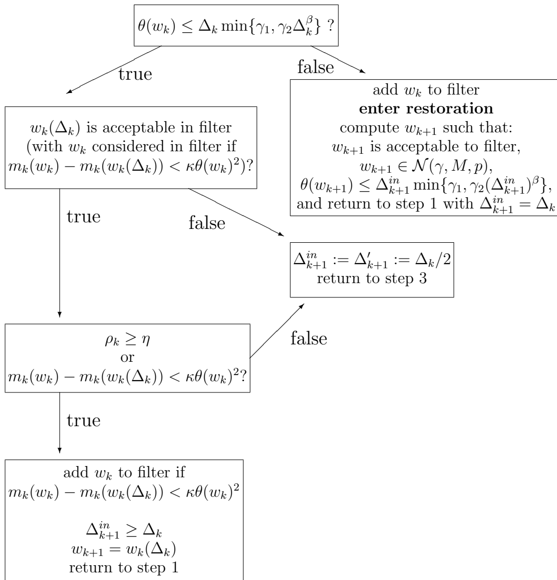
FIGURE 1. Steps 4-11 of Algorithm 3.1.
