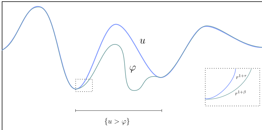
Fig. 1 Detachment of u from \varphi at the free boundary
