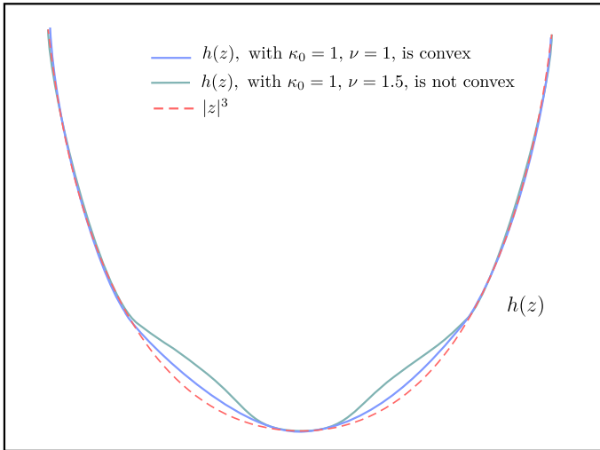
Fig. 2 The function h(z) for p = 3 and certain values of \kappa_0 and \nu
