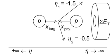
Fig. 1. Schematic illustration of the kinematic variables in the measurement. Panel (a) illustrates the convention in p + \text{Pb} collisions. Panels (b) and (c) illustrate how a single pp event provides a measurement of \sum E_T at two values of \eta^{\text{dijet}} = (\eta_1 + \eta_2)/2 , in this case for \eta^{\text{dijet}} = +1 and for \eta^{\text{dijet}} = -1 , respectively.
