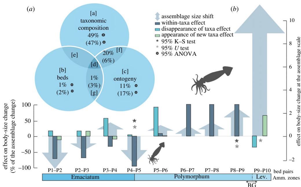
Figure 3. (a) Venn diagram depicting the partition of belemnites body-size variation between taxonomic composition, bed separation and ontogeny. The values between parentheses correspond to the whole time-series and the values without parentheses correspond to the Pli–Toa boundary. See the ‘Material and methods’ section for more details on the variation partitioning methodology. (b) Effect on body-size change at the assemblage and species scale of organization. The bed pairs in the horizontal axis represent pairwise comparisons. See electronic supplementary material (table S6) for details. For a correct interpretation of the right-side scale, the bottom of the arrowhead should be considered, rather than the tip of the arrow. Note that the x -axis depicts comparisons of consecutive pairs of beds (not to scale). BG, belemnite gap; U -test, Mann–Whitney U -test; K -S test, Kolmogorov–Smirnov test.
