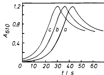
Figure 3. Influence of hexacyanoferrate on the induction period of the reaction between 1 \times 10^{-4} M N,N,N',N' -tetramethyl- p -phenylenediamine and 1.25 \times 10^{-4} M K_2S_2O_8 in water pH \approx 4 . l = 1 cm, 25 °C. [K_3Fe(CN)_6] = 0 (a), 5 \times 10^{-7} M (b) and 2.5 \times 10^{-6} M (c).
