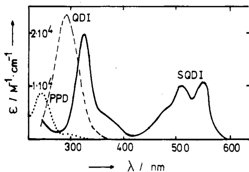
Figure 1. Spectra of N,N -diethyl- p -phenylenediamine (PPD) and its oxidation products (SQDI and QDI).
