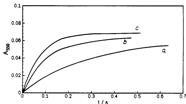
Figure 7. Absorbance-time curves for the oxidation of N,N -diethyl- p -phenylenediamine (varying concentration) by a mixture of \text{K}_2\text{S}_2\text{O}_8 ( 8.33 \times 10^{-5} M) and \text{Ru}(\text{bpy})_3^{2+} ( 3.3 \times 10^{-5} M) after illuminating it for 20 s. \lambda = 550 nm, l = 0.22 cm, [\text{PPD}] = 1.33 \times 10^{-4} M (a), 3.3 \times 10^{-4} M (b) and 6.67 \times 10^{-4} M (c).
