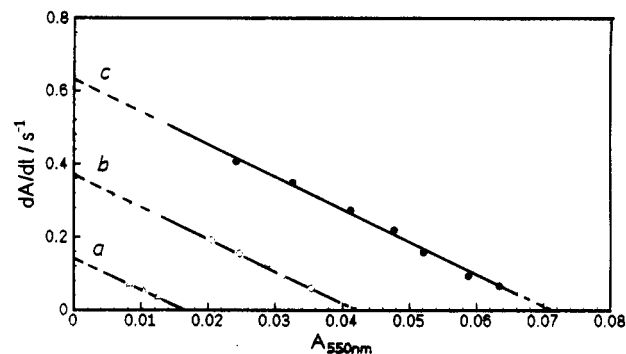
Figure 8. Plot of the formation rate of SQDI ( dA/dt ) against the corresponding absorbance ( A_{550\text{nm}} ). \lambda = 550 nm, l = 0.22 cm (see Table 2).
