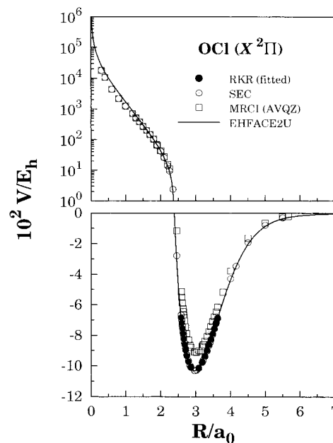
Figure 2. Interatomic potential for OCl( X^2\Pi ). As in Figure 1, the open circles nearly coincide with the solid ones over the regions where they overlap.
