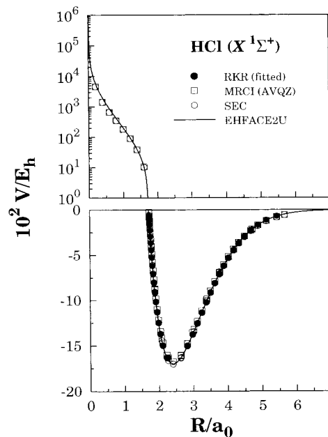
Figure 1. Interatomic potential for HCl( X^1\Sigma^+ ). Note that the open circles nearly coincide with the solid ones over the complete range of internuclear distances.
