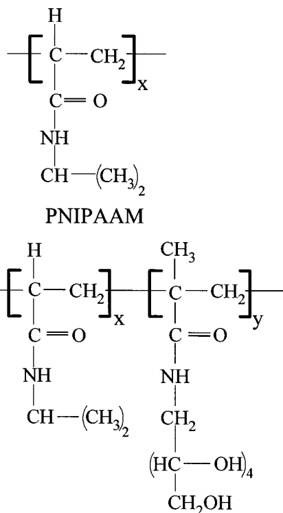
Figure 1. Scheme of the molecular structures of the repeating units in PNIPAAM and in copoly(PNIPAAM x /VS y ) where on average x/y \approx 6.5 (see text).
