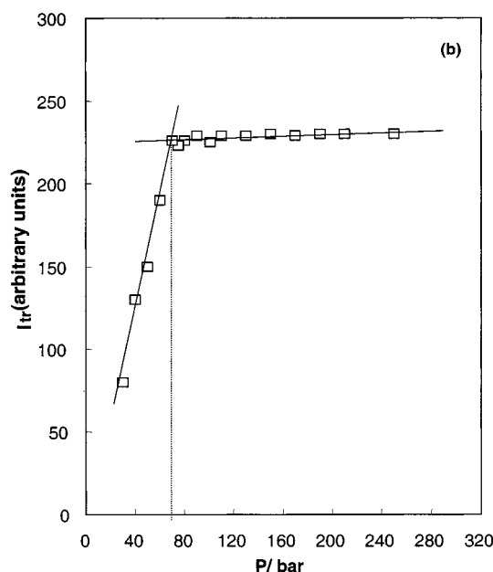
Figure 3. Examples of isobaric (a) and isothermal (b) runs during phase transition plotted as transmitted intensity vs T or p , respectively. The dashed lines locate the cloud-point temperature or pressure. (a) P3 (3.07 wt %) + water solution at p = 262.5 bar run; (b) CP1 (4.32 wt %) + water solution at T = 310.3 K run.
