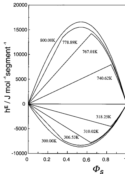
Figure 8. Modeled results (see eq 3 and Table 2) for the excess enthalpy, h^E , in \text{J mol}^{-1}\text{ segment}^{-1} vs polymer segment fraction, \Phi_s , of (P1 + water) at p = 1 bar. Results are represented for eight temperatures. While at 300 K (or below) and at 800 K (or above) the (P1 + water) system is in its one-phase region irrespective of concentration; at all other intermediate temperatures there is some window of immiscibility. The straight lines in the h^E vs \Phi_s plot represent the two-phase region.
