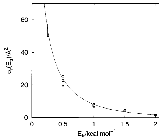
Figure 2. Cross sections for the bimolecular reaction \text{H} + \text{ArCN} , \square and \triangle ; calculation with vibrational energy on the van de Waals modes of ArCN, \Delta .
