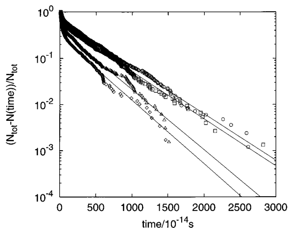
Figure 5. Decay rate for the HCN* molecules as a function of time and translational energy: (○) E_{tr} = 1.0 kcal mol -1 ; (□) E_{tr} = 2.0 kcal mol -1 ; (△) E_{tr} = 4.0 kcal mol -1 ; (◇) E_{tr} = 6.0 kcal mol -1 . See the text for the fitted curves.
