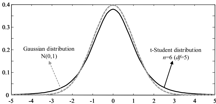
Figure F.2: t -Student versus Gaussian distribution: the t -Student distribution is more spread out than the Gaussian distribution and depends on the number of degrees of freedom df , which is computed from the sample size n as df = n - 1 . The lesser df is, more spread out is the t -Student distribution.
