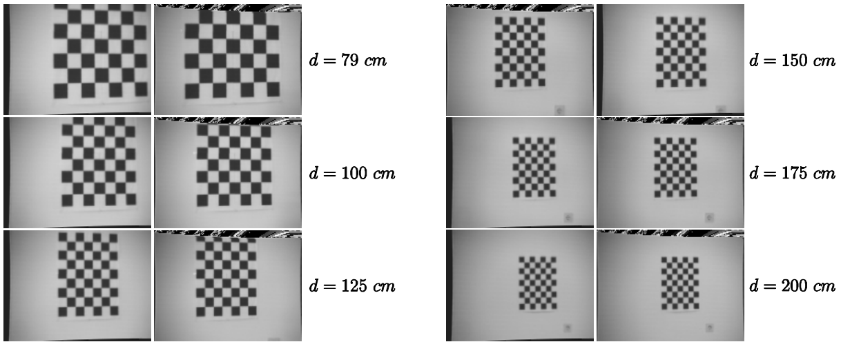
Figure 4.12: Set of image pairs used to calibrate the parameters of the sensor model. Every image pair focuses on a checkerboard — a planar obstacle — that is parallel to the image plane of both cameras of the stereo-rig. Each stereo pair was acquired with a different distance d between the stereo-rig and the checkerboard.
