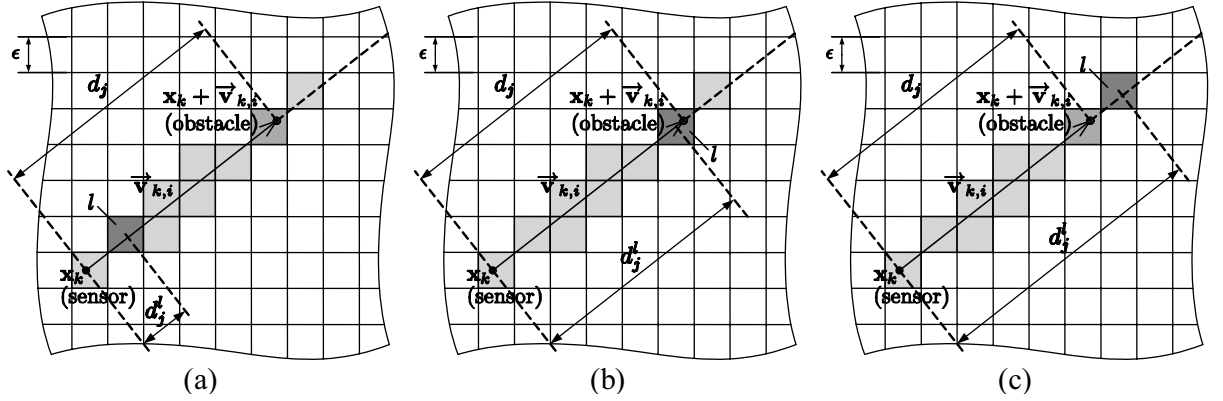
Figure 4.5: Converting a range measurement into a coverage estimate of a given voxel l \in \mathcal{Y} (darkest shaded voxel): (a) the voxel is likely to be fully empty ( c_l = 0 ) if it is located between the sensor and the obstacle; (b) the voxel's coverage takes values 0 \leq c_l \leq 1 if the voxel contains the point where the obstacle is detected, depending on the difference -\frac{\epsilon}{2} \leq (d_j^l - d_j) \leq \frac{\epsilon}{2} ; (c) the voxel is likely to be fully occupied ( c_l = 1 ) if it is located immediately behind the detected obstacle.
