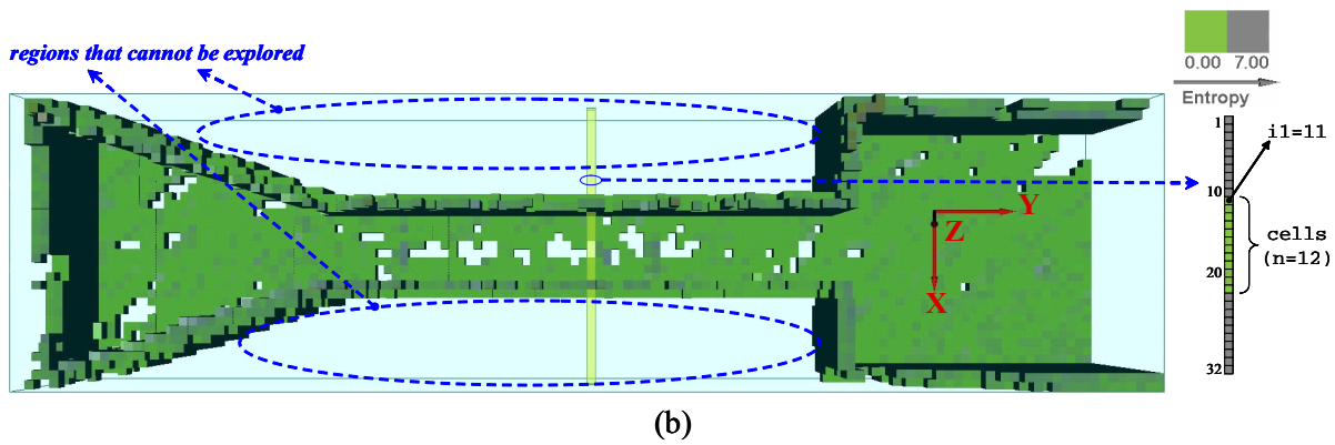
Figure 7.2: Example of a large-scale map obtained through a computer simulation: (a) different views of the map; (b) parallelepiped encompassing the whole environment and, on the right, an example of a strip along the xx axis, whose 12 explored voxels are stored in memory (all the voxels with entropy lesser than 7 bits).
