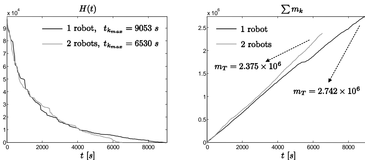
Figure 5.11: Comparison of a 3-D mapping mission using a single robot or two robots: entropy of the map along the mission (left) and cumulative number of processed measurements along the mission (right). For the presented case, the parameters' values I_{min} = 0.0145 and s_{k_{max}} = 2500 were used.
