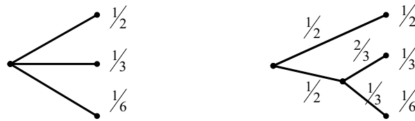
Figure 3.4: When breaking down a choice into two successive choices, the original entropy is the weighted sum of the individual values of entropy.
