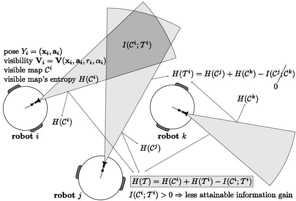
Figure 6.7: Example showing visible maps with 3 robots i , j and k . The mutual information I(\mathcal{C}^i; \mathcal{T}^i) > 0 , decreases the team's visible map joint entropy H(\mathcal{T}) , i.e. the team covers a smaller part of the map's uncertainty H(\mathcal{C}) .
