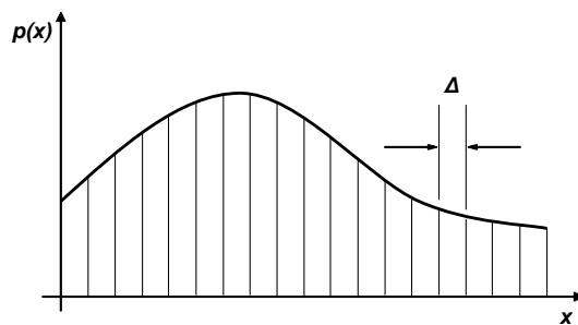
Figure 3.7: Quantization of a continuous random variable.
