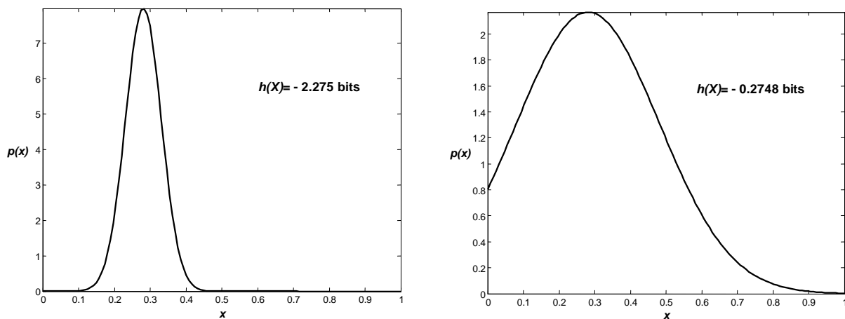
Figure 3.6: Differential entropy is a relative measure of information and uncertainty, though it cannot be taken as an absolute measure.
